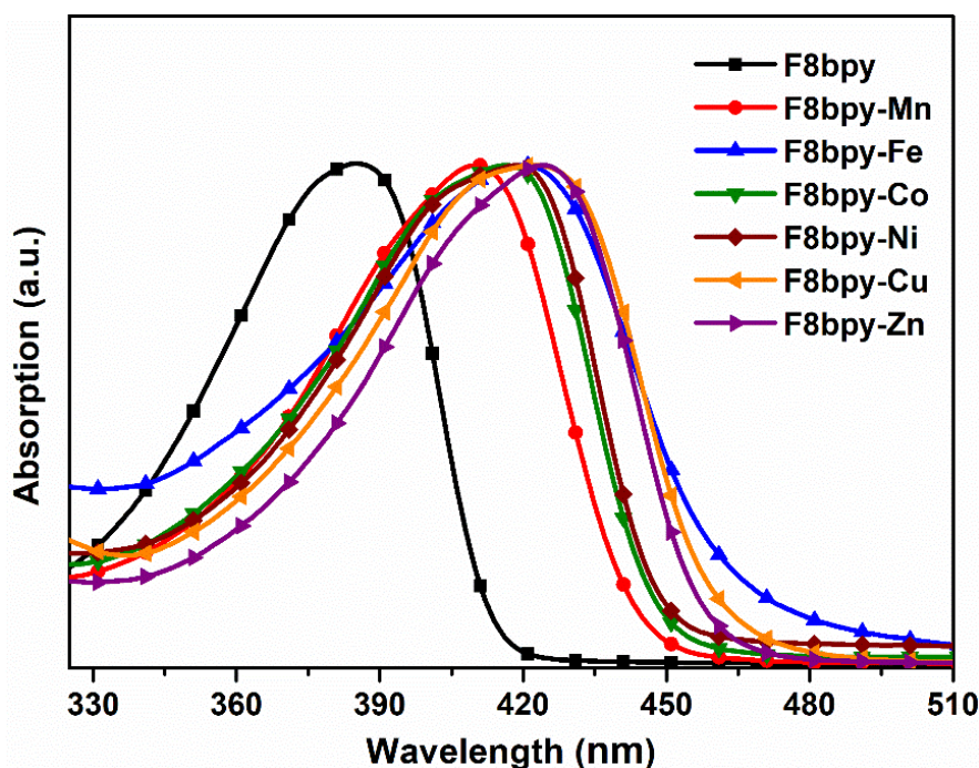
Figure 3. UV-vis absorption spectra of F8bpy/metal complex in chlorobenzene.
