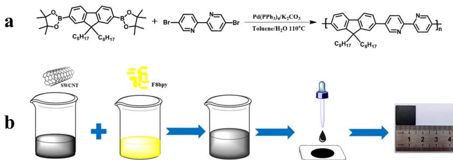
Figure 1. Synthesis of F8bpy (a), and schematic illustration showing the preparation process of the F8bpy or F8bpy/metal complex/SWCNT nanocomposites (b).
