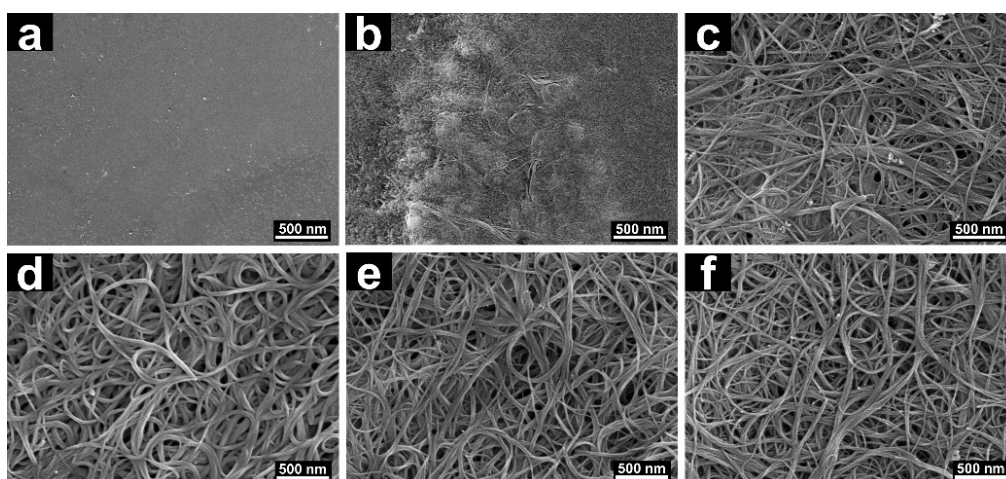
Figure 2. SEM images of F8bpy/SWCNT hybrid films with different SWCNT contents: 0 (a), 10 (b), 30 (c), 50 (d), 70 (e), and 90 wt.% (f).
