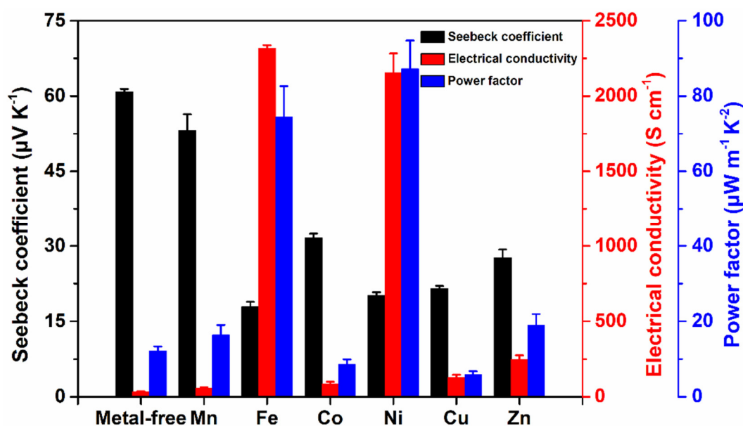
Figure 6. Thermoelectric properties of F8bpy/metal complex/SWCNT composite films with different transition metal ions (SWCNT 50 wt.%).
