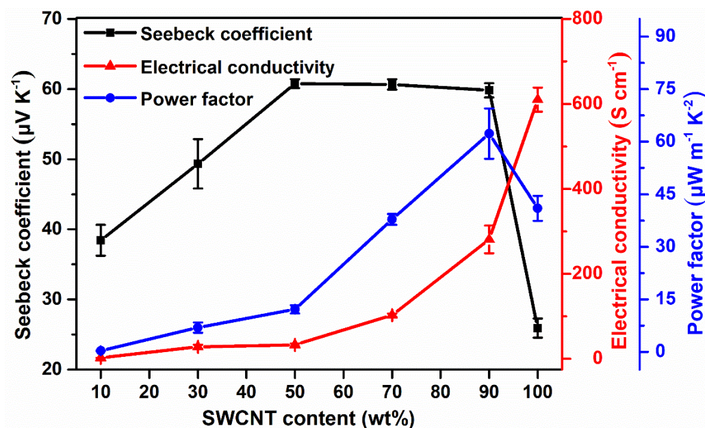
Figure 5. Electrical conductivities, Seebeck coefficients, and power factors at room temperature for the pure F8bpy/SWCNT composite films and pure SWCNT film.
