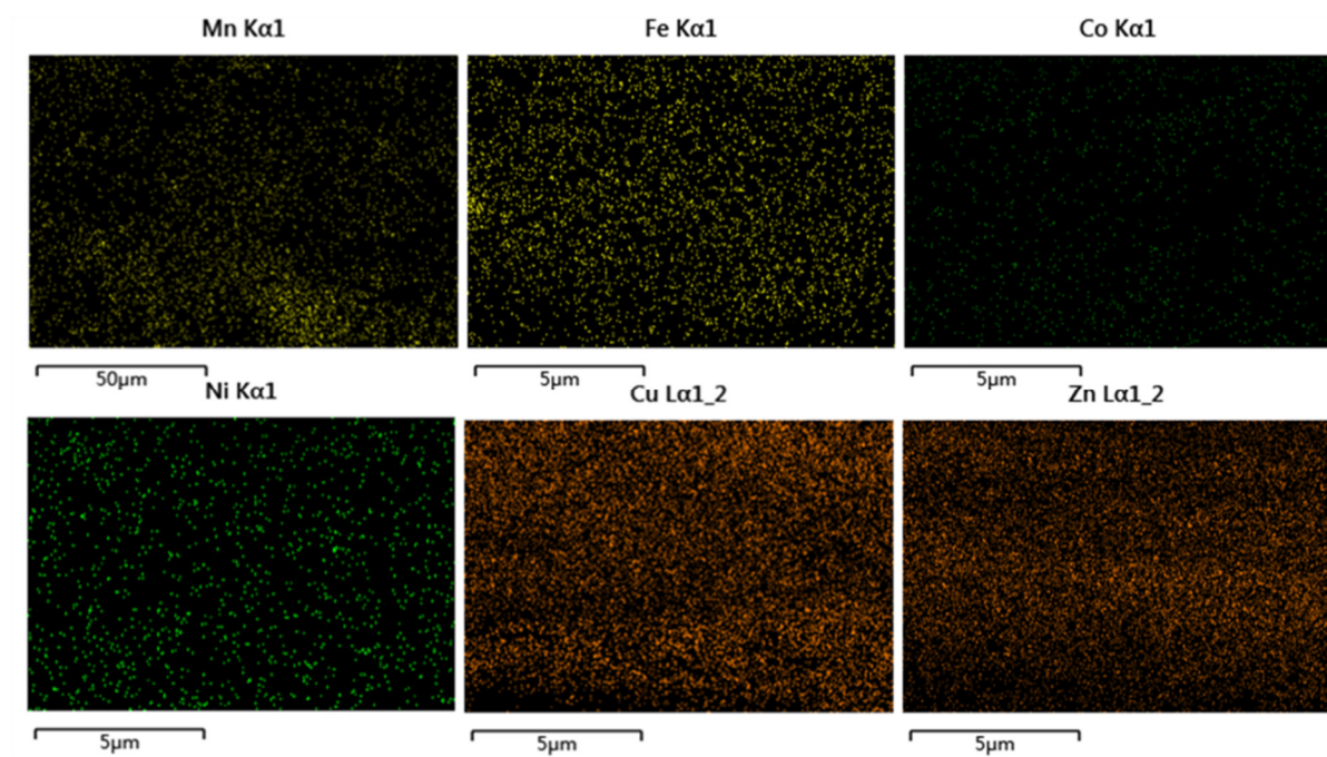
Figure 4. Energy dispersive X-ray spectroscopy (EDS) images of F8bpy/metal/SWCNT composites films with different transition metal ions.
