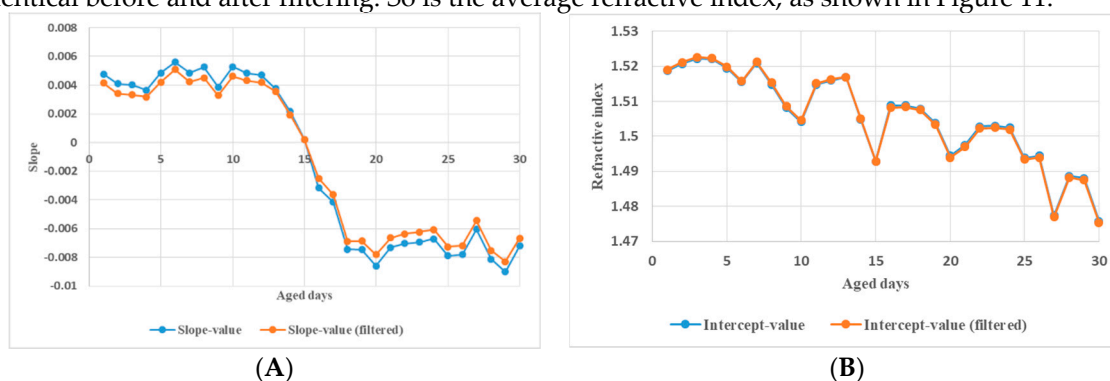
Figure 10. Comparison of the slope (A) and the intercept (B) of the linear fitting between unfiltered and filtered refractive index vs. frequency data.
