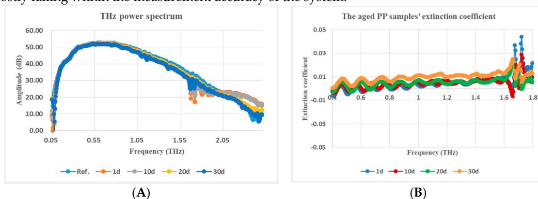
Figure 2. Terahertz (THz) frequency transmission spectra (A) and extinction coefficients (B) of samples during aging.
