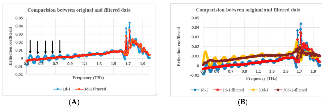
Figure 8. Comparison of extinction coefficient vs. frequency between unfiltered and filtered data; (A). 1d-1 aged PP sample, (B). 1d-1, 30d-1 aged PP samples, and A is one part of B.
