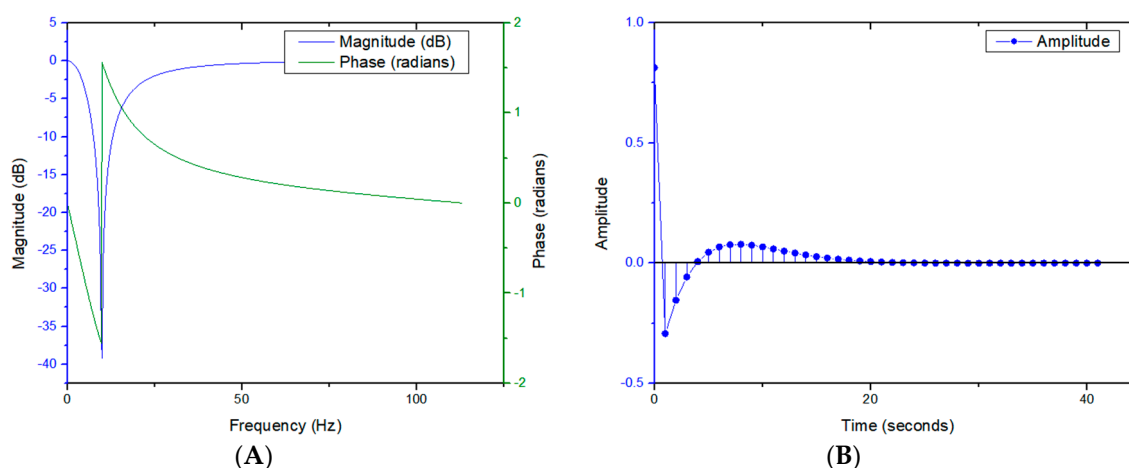
Figure 9. Second-order Butterworth band-stop infinite impulse response filter (IIR) filter's response curves; (A). Magnitude and phase response (B). Impulse response.
