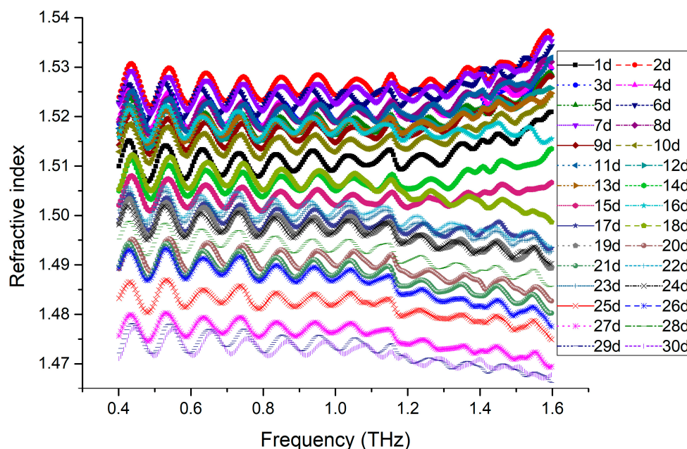
Figure 3. Refractive index vs. THz frequency for samples in different aged states.
