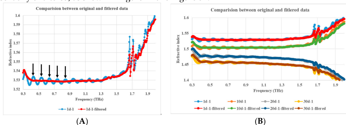
Figure 7. Comparison of refractive index vs. frequency between unfiltered and filtered data; (A). 1d-1 aged PP sample, (B). 1d-1, 10d-1, 20d-1, 30d-1 aged PP samples, and A is one part of B.
