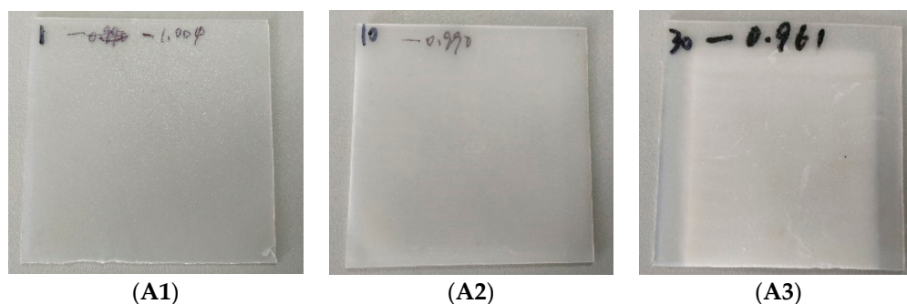
Figure 1. Photographs polypropylene (PP) samples at different aged stages; (A1). 1d aged PP sample, (A2). 10d aged PP sample, (A3). 30d aged PP sample.
