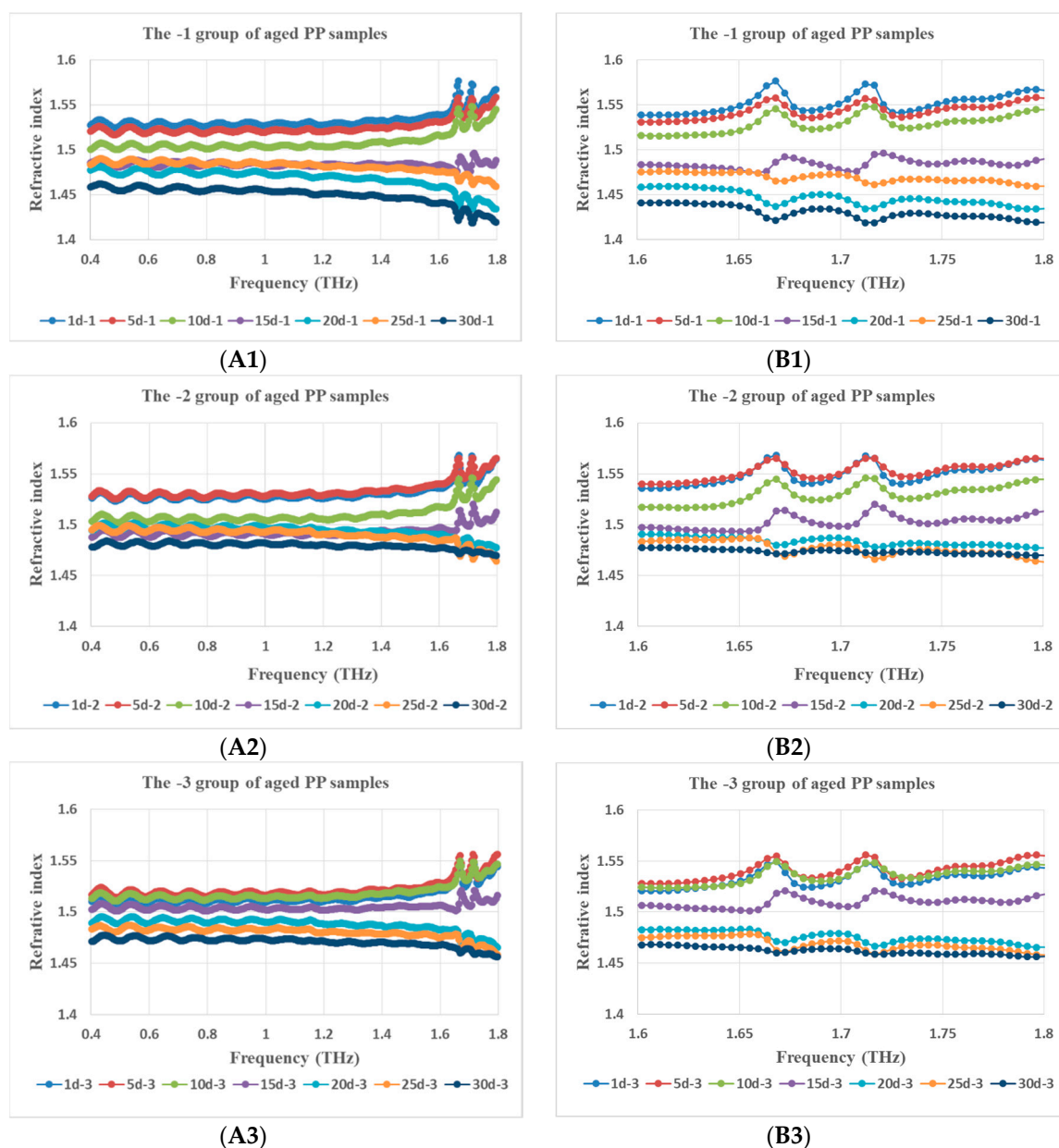
Figure 6. Refractive index vs. THz frequency for 3 groups of PP samples in different aged states (A1, A2, A3 stands for -1, -2, -3 group and B is the enlargement of part A).
