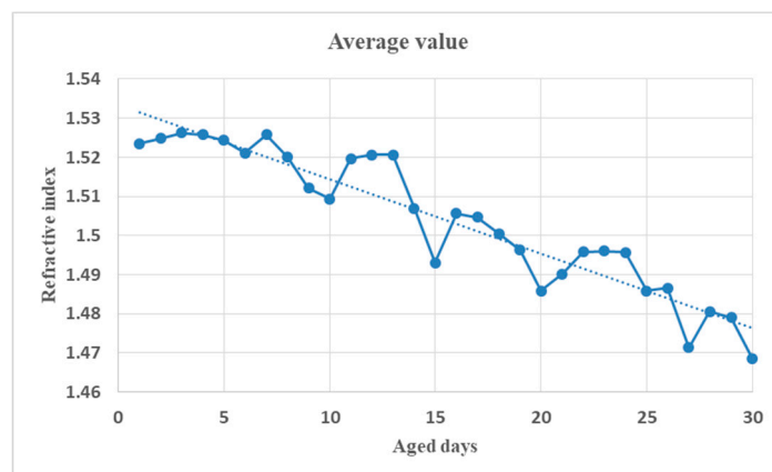
Figure 5. Relationship between the average value of refractive index and the aged days (The dotted straight line is its linear fitting).
