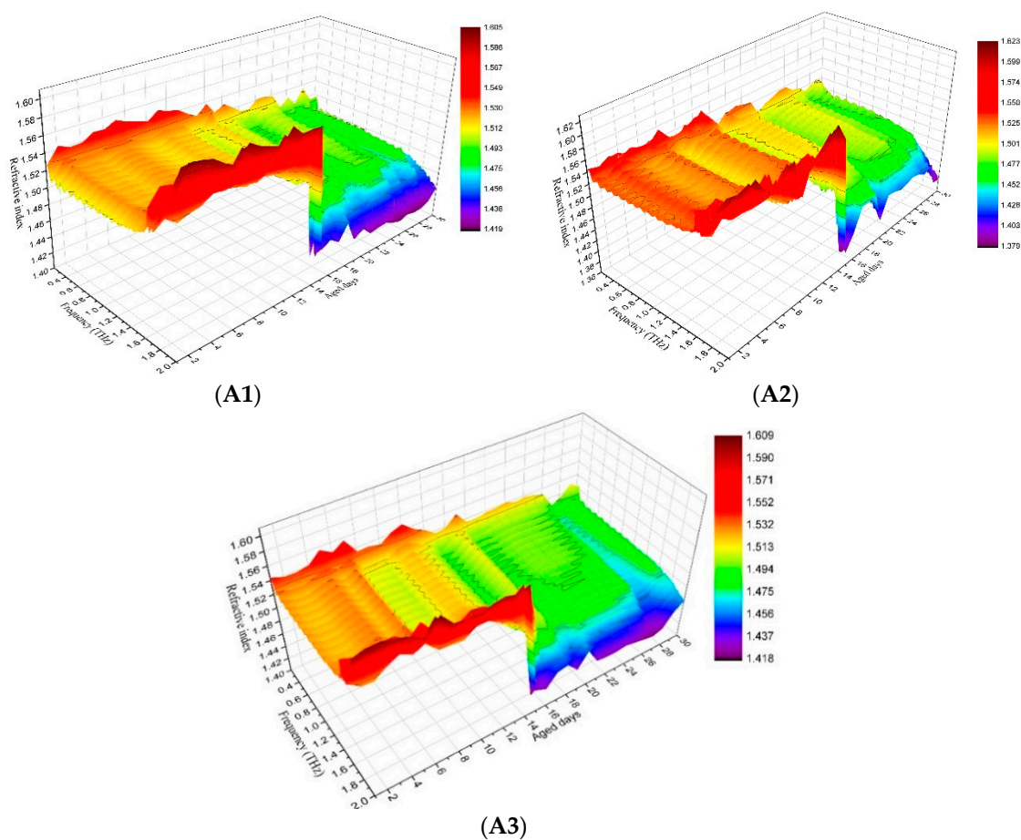
Figure 4. Three-dimensional diagram between refractive index, THz frequency and aged days (A1, A2, A3 stands for -1, -2, -3 group).
