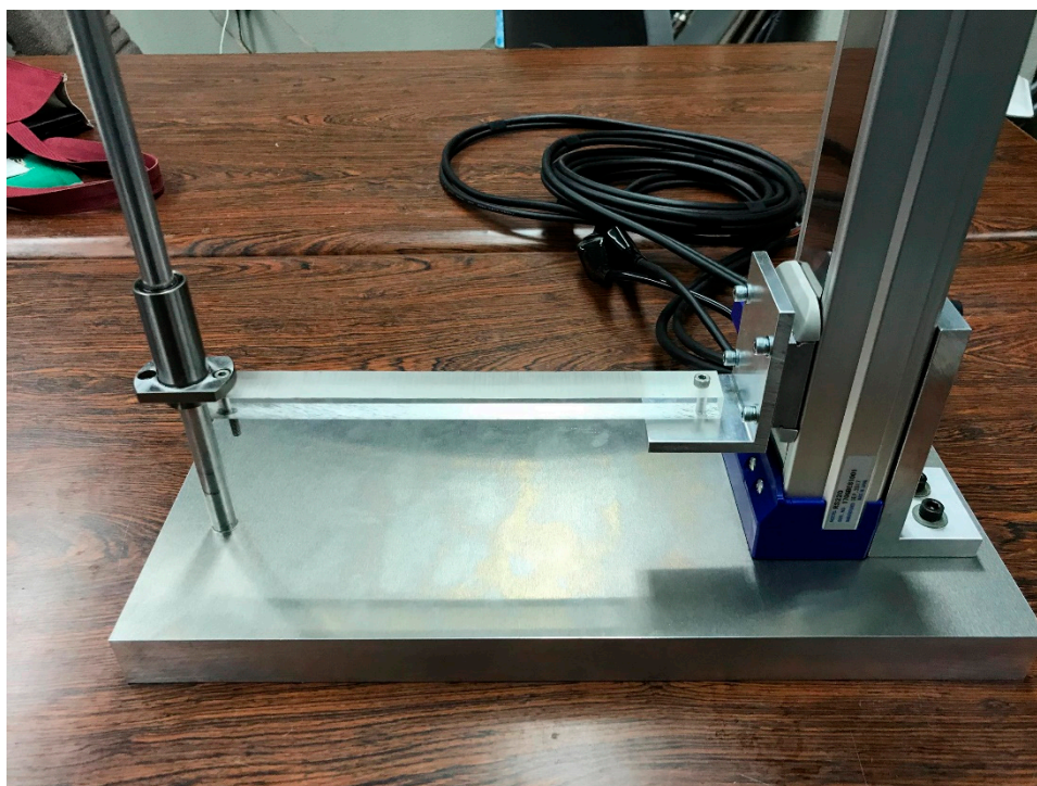
Figure S1. A photograph of the experimental setup for needlespinning.
