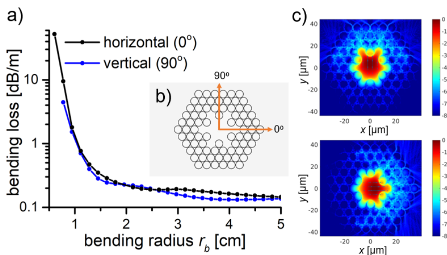
Figure 10. (a) Calculated bending losses of the fundamental modes for star structures for different bend orientation; (b) Bend-orientation scheme. The orange arrows indicate the direction of the—0° is horizontal, while 90° is vertical bend. (c) Modal field distribution, calculated for the fundamental mode at bending radius r_b = 1.3 \text{ cm} , for vertical (up) and horizontal (down) bend orientation. The color scale bar on the left defines the electromagnetic field intensity. The main reason of the higher bending losses is the coupling between the core and cladding modes, occurring in the direction of the bend.
