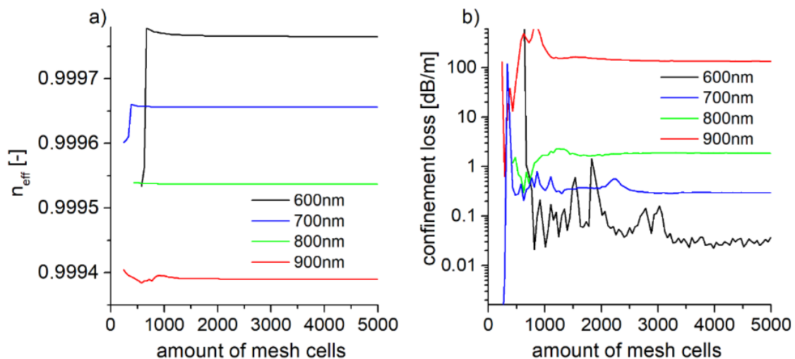
Figure 3. Calculated effective refractive index n_{eff} (a) and confinement loss (b) for the fundamental mode of the 7-cell structure, for different amount of mesh cells ( x direction) and different wavelengths. The appropriate amount of mesh cells in y direction can be calculated from Equation (3). The convergence is obtained if the number of mesh cells is greater than 3000.
