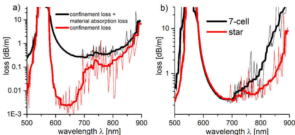
Figure 12. (a) Comparison of the loss (confinement loss + material absorption loss, black line) and confinement loss spectra (red line) of the star structure based on PMMA. The loss increase is visible, particularly in the 600–700 nm region, which suggests that the total loss here is influenced mainly by the PMMA material absorption. (b) Loss spectra of the PMMA-based 7-cell and star structures (black line and red line, respectively). In the 600–700 nm spectral region the influence of the material absorption loss is large enough to negate the confinement loss decrease of the star structure. As the wavelength increases, the latter again starts to outperform the 7-cell one.
