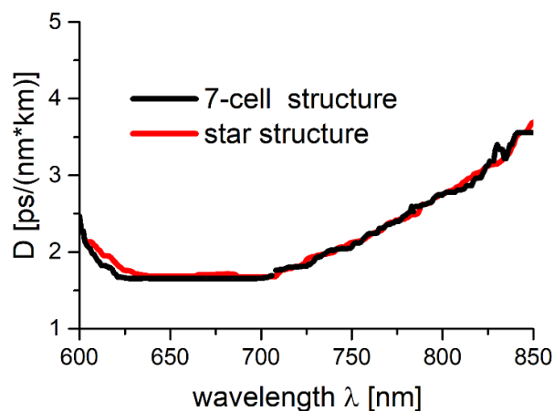
Figure 6. Calculated dispersion parameters D for 7-cell and star structures, using Equations (6) and (7). The curves are almost identical in the 600–800 nm range.
