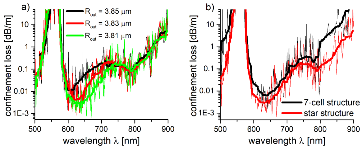
Figure 7. (a) Confinement loss of the fundamental modes for star structure, for different values of R_{out} . (b) Confinement loss of the fundamental modes for 7-cell and star structure for R_{out} = 3.81 \mu\text{m} .
