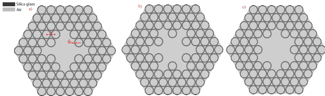
Figure 2. Modified hollow-core fiber structures, based on the 7-cell one (a) xy structure, (b) star structure, and (c) a-star structure.
