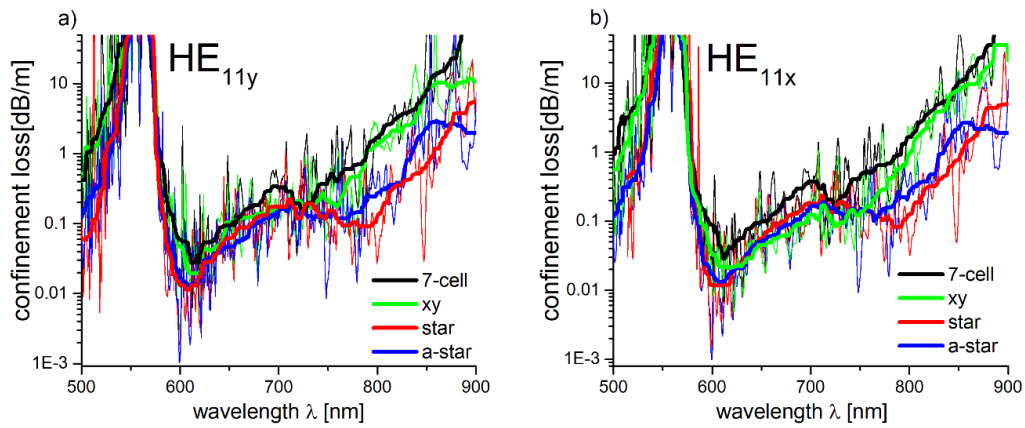
Figure 4. Calculated confinement loss spectra of the fundamental modes (a) HE_{11y} and (b) HE_{11x} for all simulated structures. In case of the modified structures, i.e., star and a-star, the loss values are clearly reduced for the wavelengths of 750 nm and longer. Additionally, the polarization of the mode (i.e., the x or y direction) has very little influence on the CL spectra of star and a-star structures.
