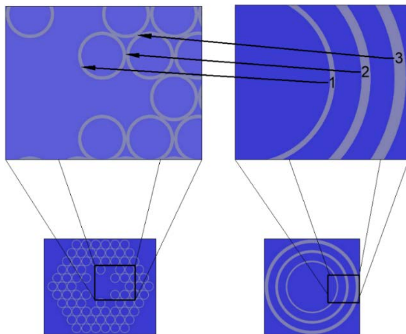
Figure 8. Star structure (bottom left) approximated by a triple ring structure (bottom right). Each of the glass rings has its wall thickness corresponding to the thickness of the glass element of the star structure, as pointed by the arrows. Consequently, 1 = d_0 = 0.54 \mu\text{m} , 2 = a = 0.98 \mu\text{m} and 3 = b = 1.24 \mu\text{m} , which corresponds to the outer radius ( R_{out} ) of a single glass capillary in the star structure being 3.85 \mu\text{m} .
