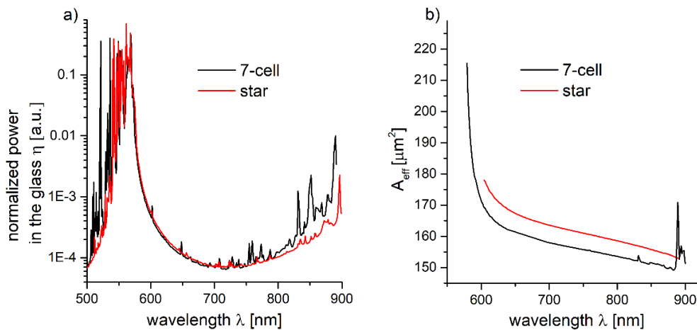
Figure 5. (a) Calculated power in the glass (in logarithmic scale), \eta , for the 7-cell and star structures. (b) Calculated effective modal areas ( A_{eff} ) of the fundamental mode. For both structures, A_{eff} decreases with the wavelength. The star structure's A_{eff} is, in general, slightly bigger in comparison to 7-cell one.
