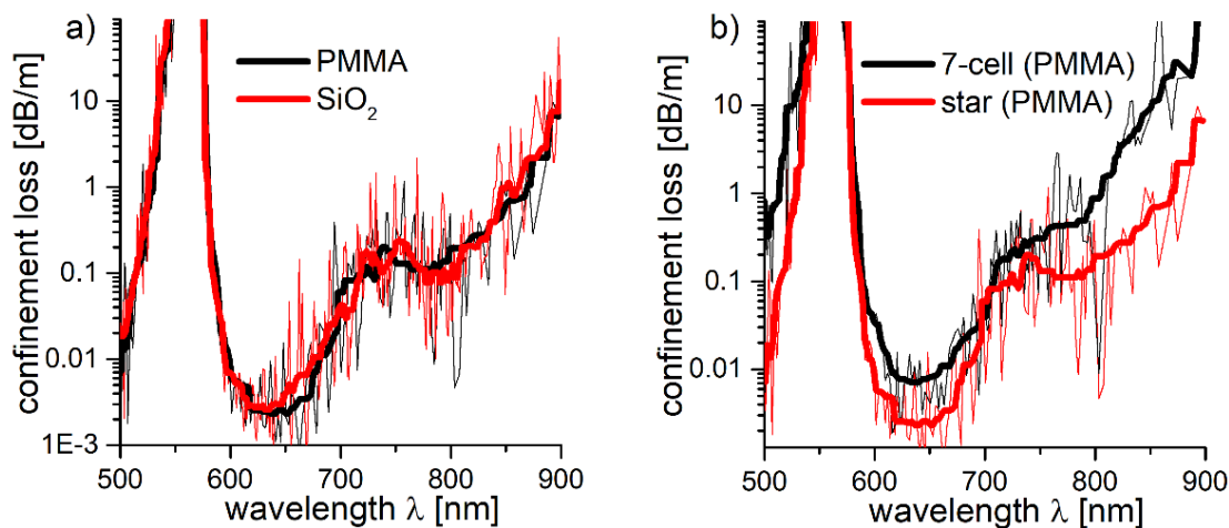
Figure 11. (a) Comparison of the confinement loss (CL) spectrum of the star structure, based on polymethylmethacrylate (PMMA, black line) and SiO 2 (silica glass, red line). The spectra are almost identical. (b) The CL spectrum for the PMMA-based 7-cell and star structures (black and red line, respectively). As in the case of their SiO 2 -based counterparts, a significant reduction of CL in the 750–800 nm spectral region is observed for the star structure.
