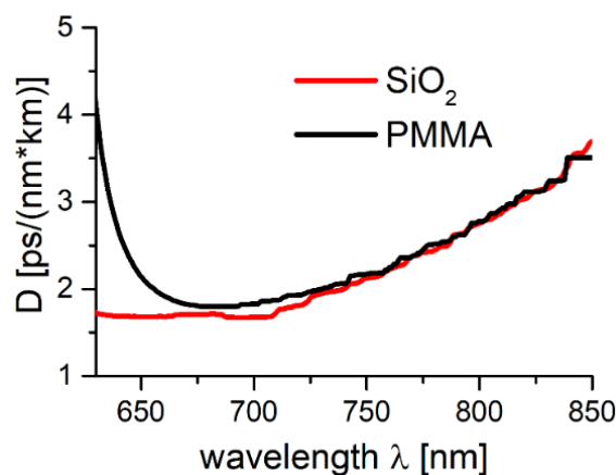
Figure 13. Dispersion parameter spectrum for the star structure made of PMMA and silica glass ( \text{SiO}_2 ). For the spectral range of \sim 675 to 800 nm, both dispersion curves are almost identical. As a result, both fibers can be considered suitable for ultrashort light pulse delivery.
