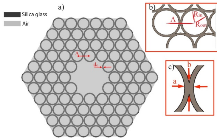
Figure 1. (a) Cross section of the designed Kagomé hollow-core fiber, (b,c) Depicted details of the construction: R_{in} , R_{out} , a , b —inner and outer radiuses of the glass capillaries, and dimensions of the struts, respectively.
