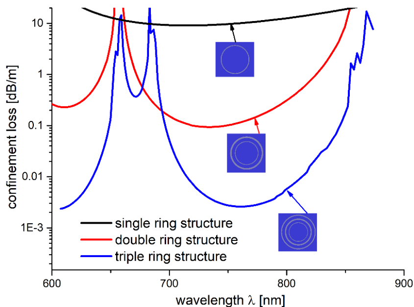
Figure 9. Confinement loss of the single- (black line), double- (red line), and triple- (blue line) ring structure. The innermost ring represents the capillary walls of the star structure, while rings 2 and 3 are a representation of the star structure's strut. To reflect the strut's different dimensions, rings 2 and 3 have their thicknesses set to 0.98 \mu\text{m} and 1.24 \mu\text{m} , which corresponds to the strut's width (dimension a ) and height (dimension b ), respectively. The appearance of three confinement loss peaks (for the triple ring structure), at the resonant wavelengths of \sim 650 , \sim 690 , and \sim 860 nm, is visible. These peaks correspond to the previously modeled CL of the star structure.
