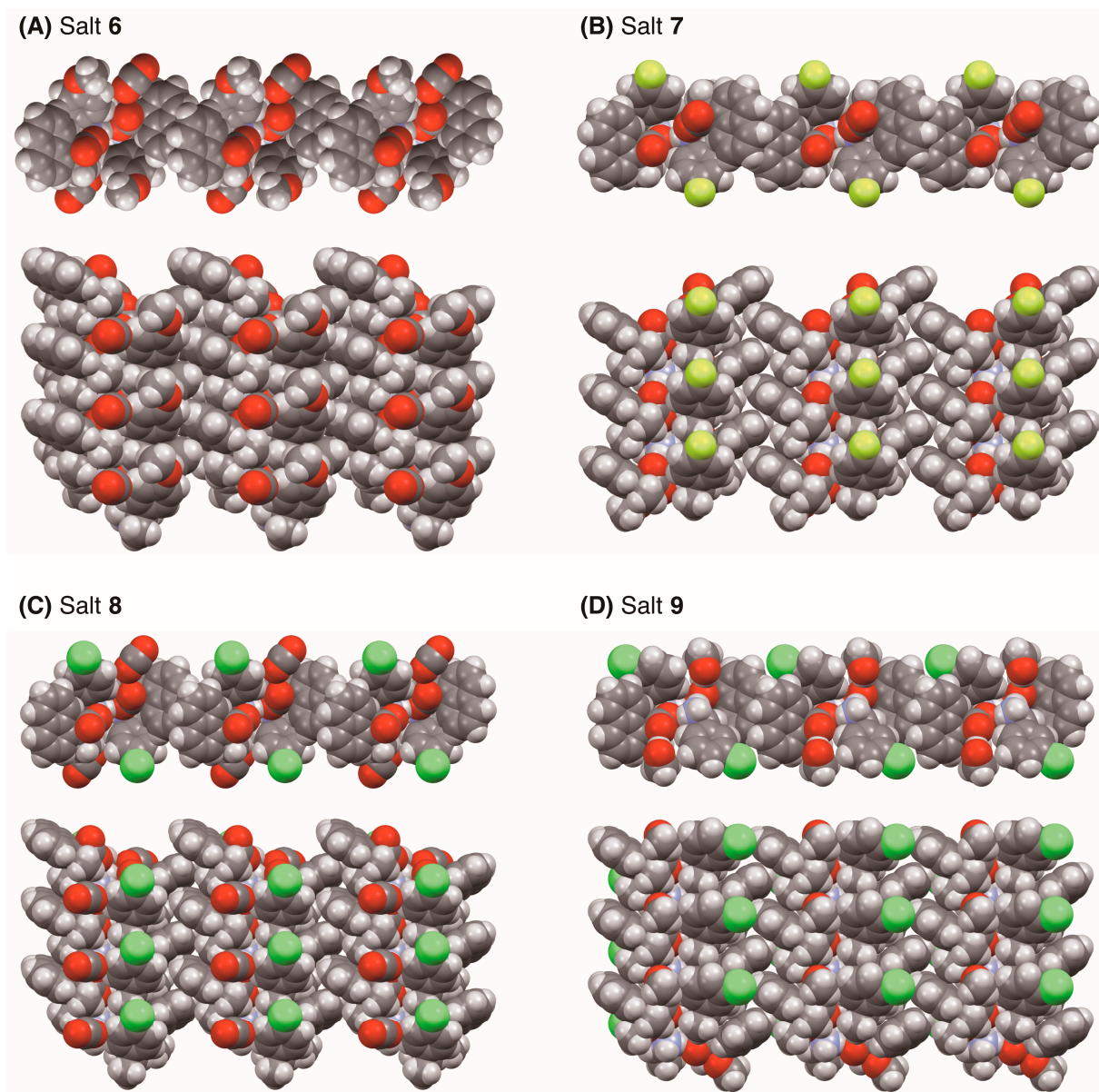
Figure S1. Top and side views of the sheet structures consisting of 2 1 columns in salts 6–9 (space-filling model).
