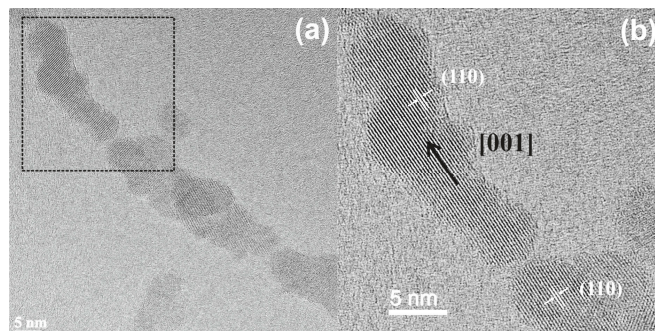
Figure 4. High-resolution TEM images of the hematite nanoparticle sample with 2.5 mM NaCl. (a) Image of a chain of hematite particles with lattice planes of neighboring particles aligned; (b) Enlarged view of the selected area in (a). The spacing between the lattice fringes corresponds to the (110) d-spacing.
