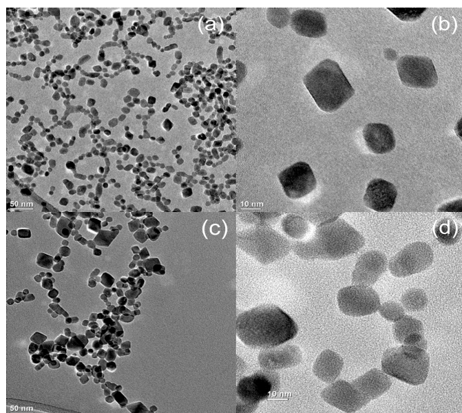
Figure 9. TEM micrographs of samples after hydrothermal treatment at 140 °C. (a,b) Sample without NaCl; (c,d) Sample with 2.5 mM NaCl.
