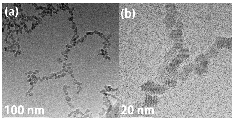
Figure 7. TEM micrographs of hematite nanoparticle sample with 0.75 mM \text{NaH}_2\text{PO}_4 . (a) Image of aggregated of hematite particles; (b) High-resolution image of aggregated particles.
