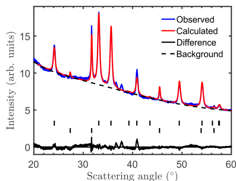
Figure 10. XRD patterns of the 2.5 mM NaCl sample after hydrothermal treatment at 140 °C. The upper tick marks correspond to the hematite structure, the lower to the NaCl structure.
