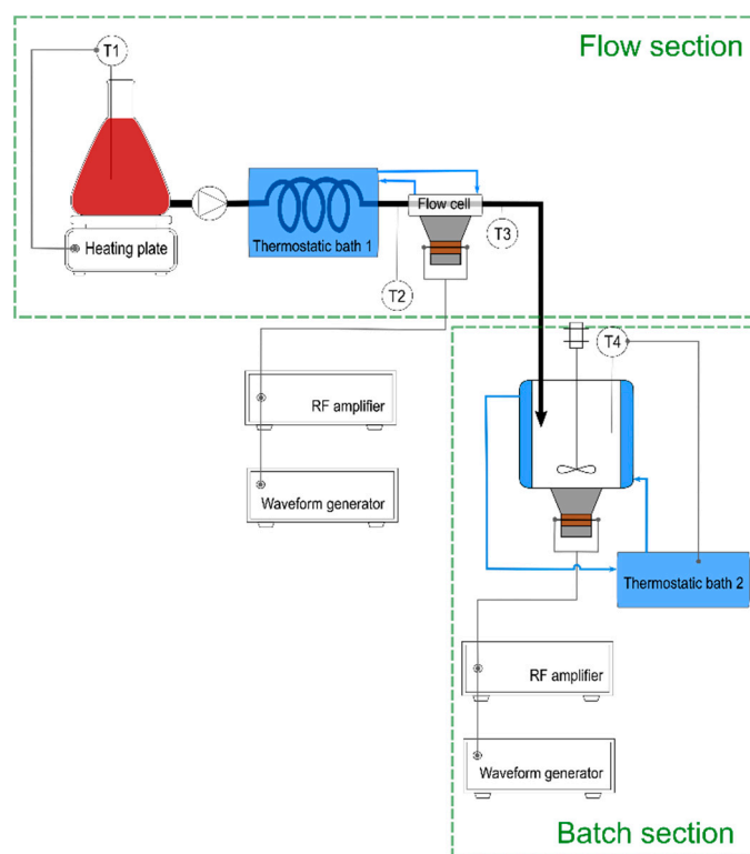
Figure S4. Continuous mode 4.
