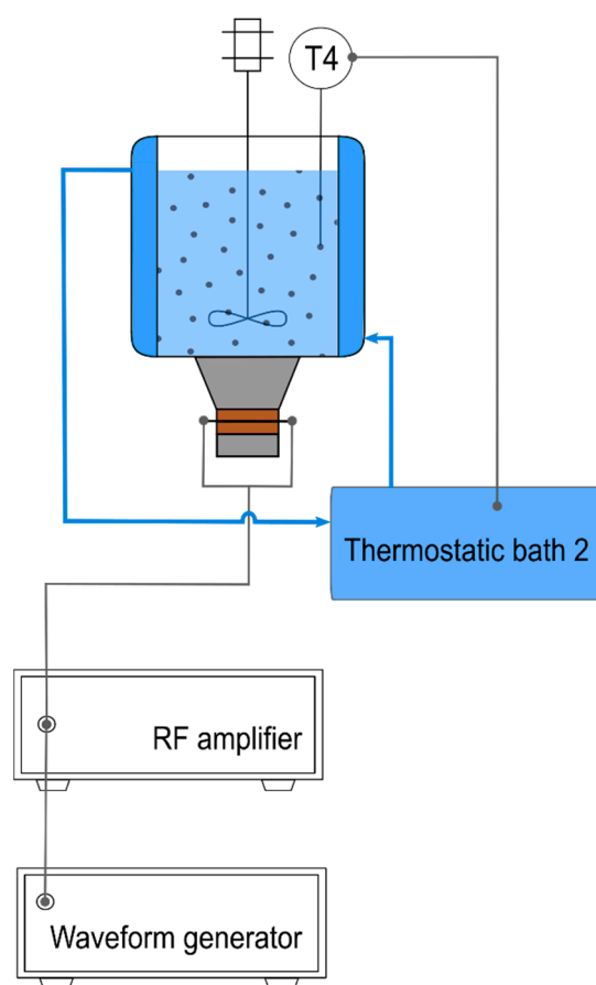
Figure S5. Batch mode.
