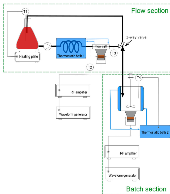
Figure S1. Continuous mode 1.
