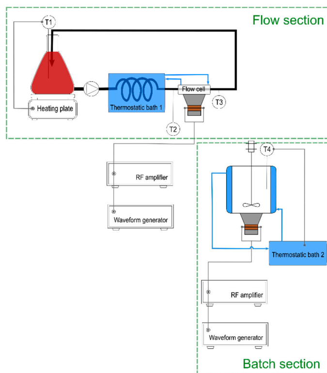
Figure S2. Continuous mode 2.
