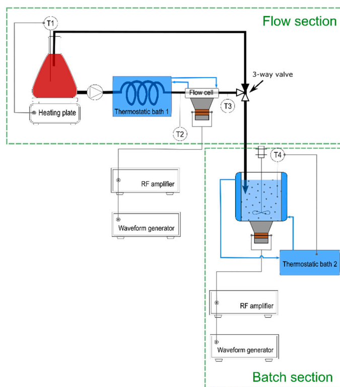
Figure S3. Continuous mode 3.
