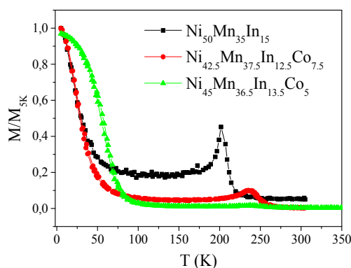
Figure 40. Temperature dependence of M/M_{5K} of as-prepared \text{Ni}_{50}\text{Mn}_{35}\text{In}_{15} , \text{Ni}_{42.5}\text{Mn}_{37.5}\text{In}_{12.5}\text{Co}_{7.5} and \text{Ni}_{45}\text{Mn}_{36.5}\text{In}_{13.5}\text{Co}_5 microwires. Reproduced from reference [114], Figure 1b.
