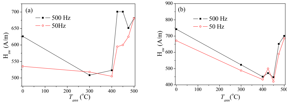
Figure 12. Dependence of the switching field on the annealing temperature of samples with \rho = 0.41 (a) and \rho = 0.6 (b) measured at f = 50 and 500 Hz. Reproduced from reference [70], Figure 5.
