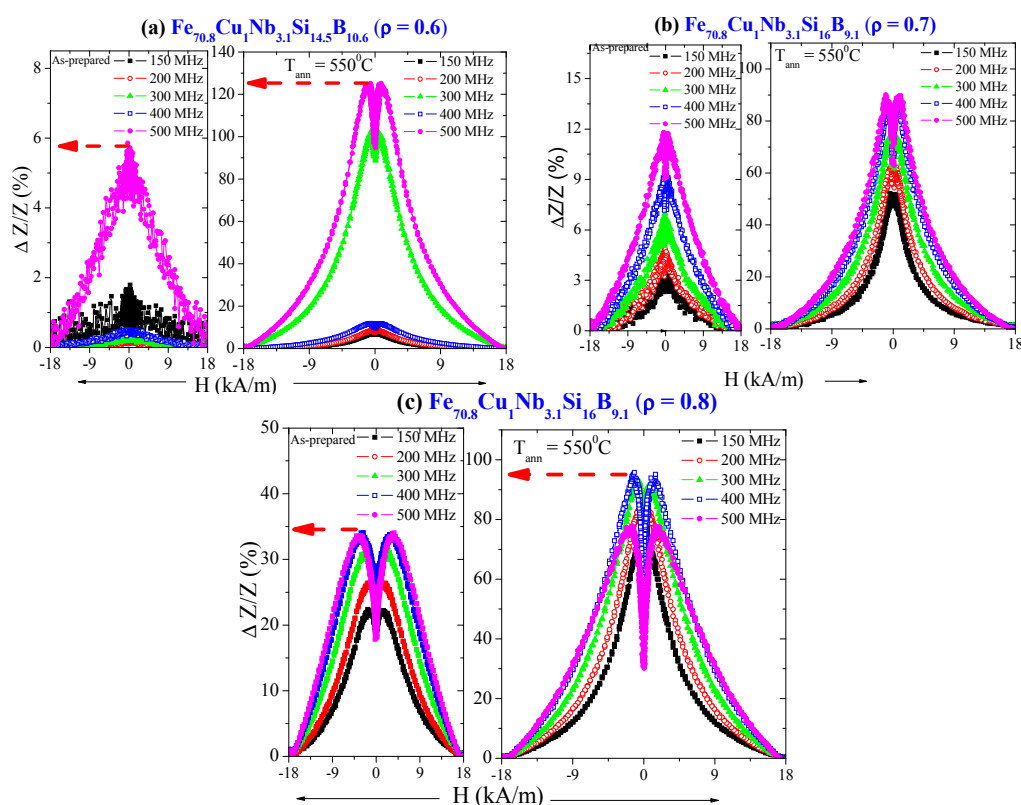
Figure 9. \Delta Z/Z (H) of as-prepared and annealed \text{Fe}_{70.8}\text{Cu}_1\text{Nb}_{3.1}\text{Si}_{14.5}\text{B}_{10.6} at T_{\text{ann}} = 550^\circ\text{C} of for \rho -ratio = 0.6 (a); \Delta Z/Z (H) of \text{Fe}_{70.8}\text{Cu}_1\text{Nb}_{3.1}\text{Si}_{16}\text{B}_{9.1} for \rho -ratio = 0.7 (b); and \rho -ratio = 0.8 (c). Driving frequencies are provided in each figure. Reproduced from reference [47], Figure 6.
