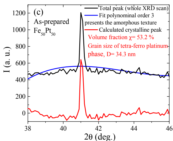
Figure 36. XRD of as-prepared Fe 33.3 Pt 64.7 B 2 (a), Fe 50 Pt 50 (b) microwires, and analysis of XRD spectra for average grain size and volume fraction of Fe 50 Pt 50 microwire (c). Reproduced from reference [48], Figure 3.
