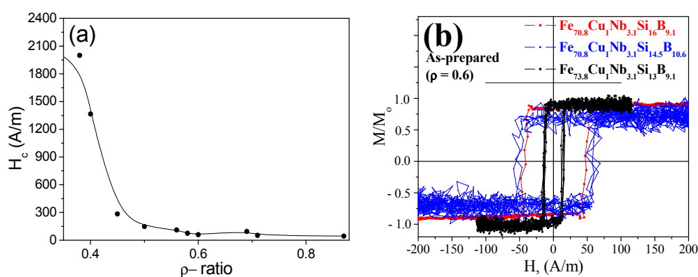
Figure 4. Coercive field dependence on \rho -ratio for as-prepared \text{Fe}_{70.8}\text{Cu}_1\text{Nb}_{3.1}\text{Si}_{16}\text{B}_{9.1} glass-coated microwires (a), hysteresis loops of as-prepared \text{Fe}_{70.8}\text{Cu}_1\text{Nb}_{3.1}\text{Si}_{16}\text{B}_{9.1} , \text{Fe}_{70.8}\text{Cu}_1\text{Nb}_{3.1}\text{Si}_{14.5}\text{B}_{10.6} , and \text{Fe}_{73.8}\text{Cu}_1\text{Nb}_{3.1}\text{Si}_{13}\text{B}_{9.1} Finemet glass-coated microwires with the same \rho -ratio = 0.6 (b). Reproduced from reference [47] Figure 1.
