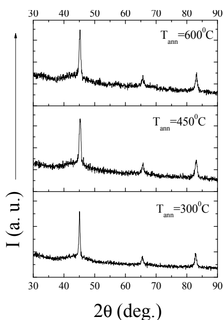
Figure 10. XRD patterns of Hitperm \text{Fe}_{38.5}\text{Co}_{38.5}\text{B}_{18}\text{Mo}_4\text{Cu}_1 microwire ( \rho \approx 0.6 ) annealed at different temperatures for 1 h. Reproduced from reference [10], Figure 7.
