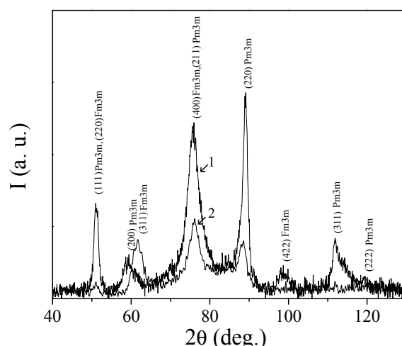
Figure 45. X-ray diffraction patterns of \text{Ni}_{63.8}\text{Mn}_{11.1}\text{Ga}_{25} samples annealed at T = 500\text{ }^{\circ}\text{C} for 30 min. 1—glass-coated samples; 2—uncoated samples. Reproduced from reference [128], Figure 2.
