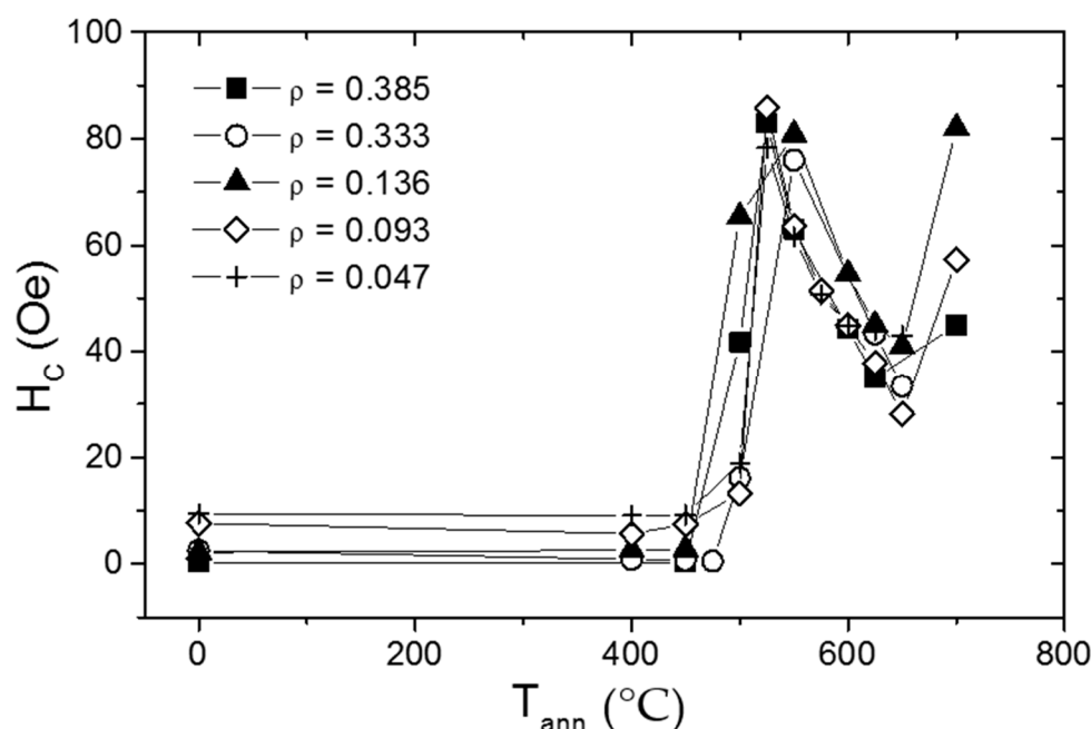
Figure 30. Effect of the annealing temperature on the coercivity of \text{Fe}_{72.3}\text{Cu}_1\text{Nb}_{3.1}\text{Si}_{14.5}\text{B}_{9.1} microwire. Reproduced from reference [96], Figure 2.
