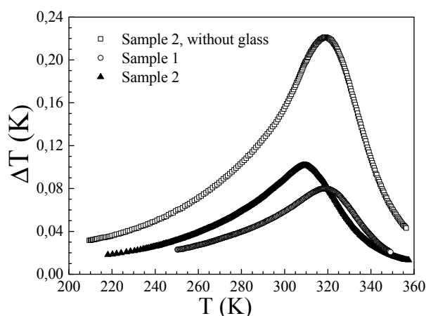
Figure 46. Temperature dependence of the magnetocaloric effect, \Delta T , in Heusler-type Ni-Mn-Ga glass-coated microwires annealed at 823 K for \Delta H = 18 kOe. Reproduced from reference [26], Figure 5.
