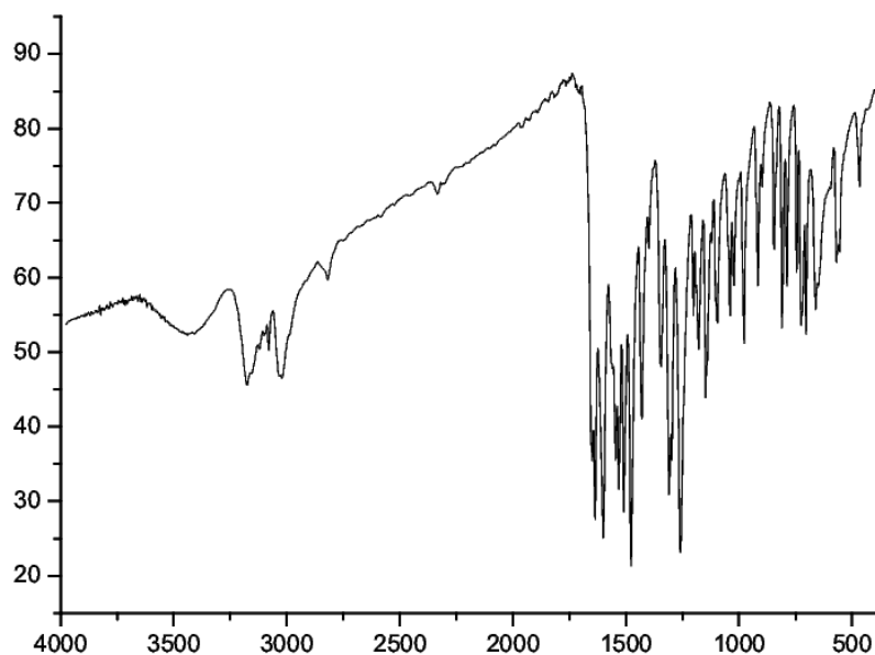
Figure S1. The IR spectrum of compound 1.
