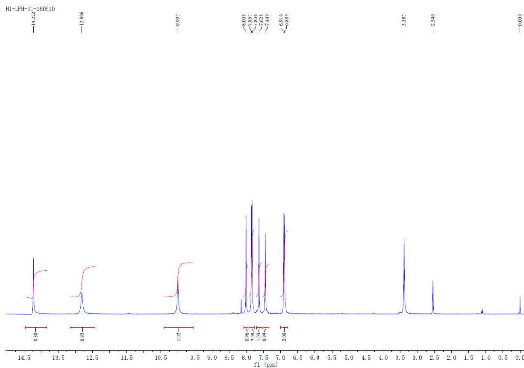
Figure S3. ^1\text{H} NMR spectrum of compound 1.
