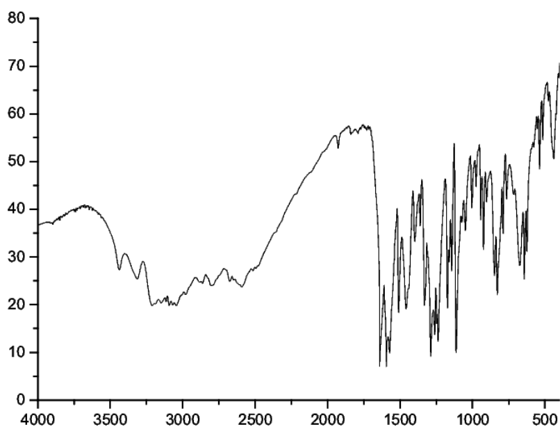
Figure S2. The IR spectrum of compound 2.
