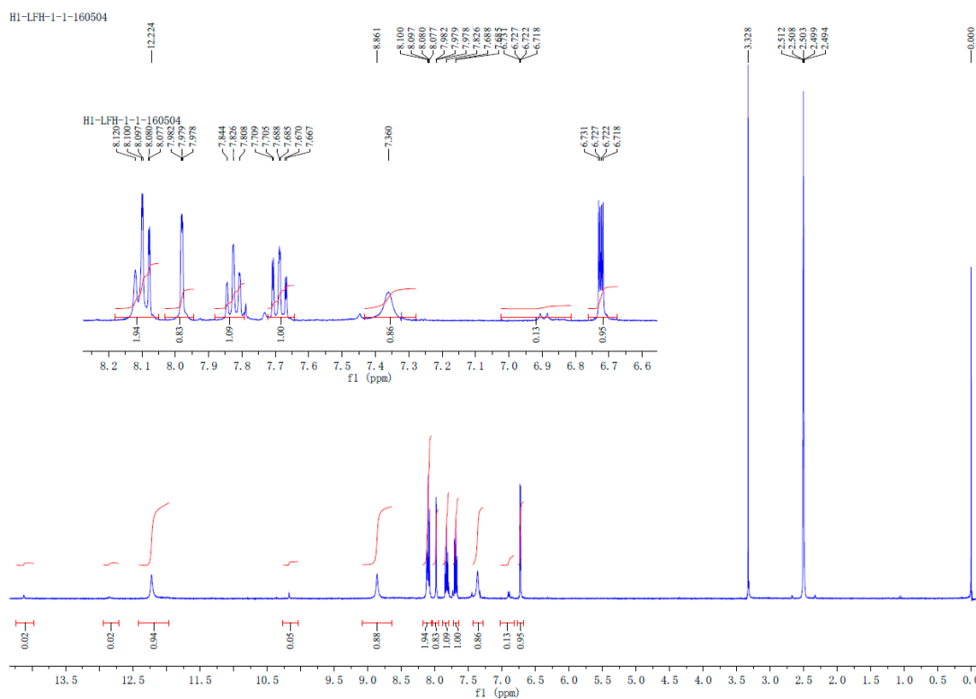
Figure S4. ^1\text{H} NMR spectrum of compound 2.
