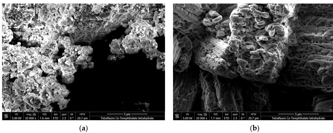
Figure 14. SEM pictures of Tetrafluoro Ca-terephthalate tetrahydrate (5e) after preparation (a) and one full cycle (b), both at a magnification of 10,000×.
