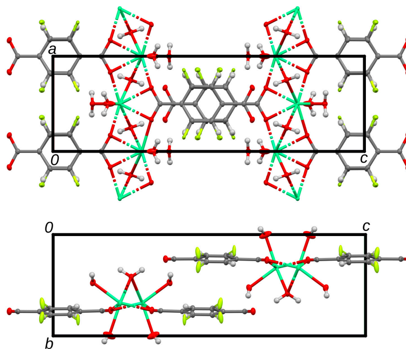
Figure 7. Crystal structure of 2-fluoro calcium terephthalate viewed along ( top ) [010] and ( bottom ) [100]. Ca (green), F (yellow), O (red), and C (grey) atoms are represented by ellipsoids drawn at the 50% probability levels; H atoms are represented by spheres of arbitrary radius.
