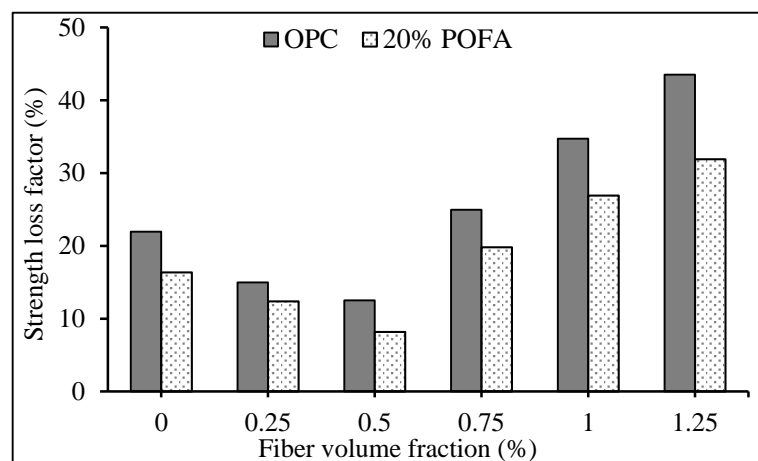
Figure 10. Strength loss factors of concrete mixes exposed to \text{MgSO}_4 solution at 365 days.
