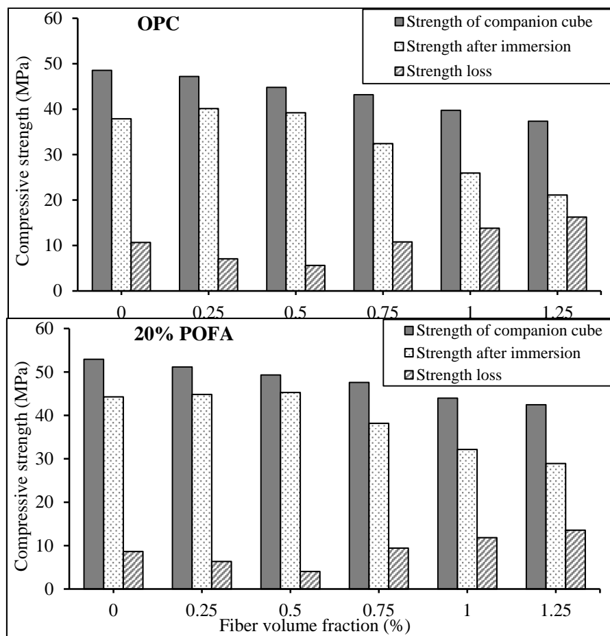
Figure 9. Effect of WMP fibres on the compressive strength of water-cured specimens and those exposed to \text{MgSO}_4 solution after 365 days.
