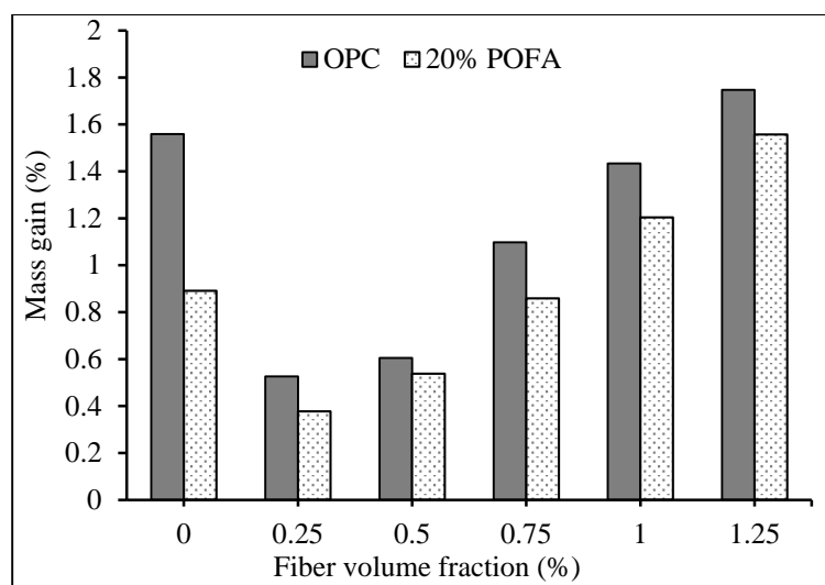
Figure 8. Effect of WMP fibre on the mass gain of concrete specimens exposed to \text{MgSO}_4 solution.
