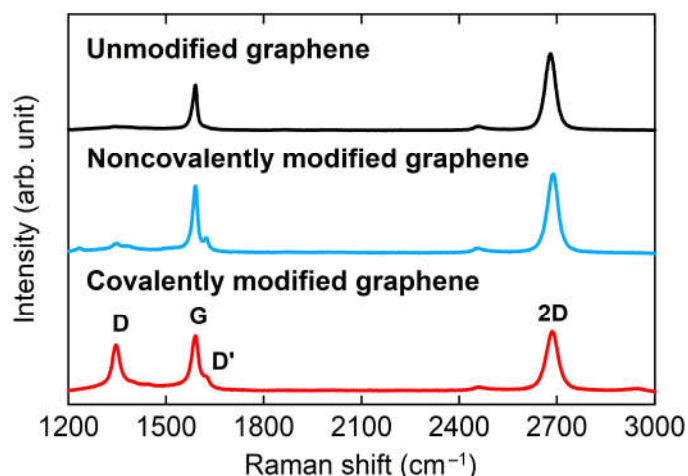
Figure 7. Raman spectra of unmodified, and noncovalently and covalently modified graphene on \text{SiO}_2/\text{Si} substrate.
