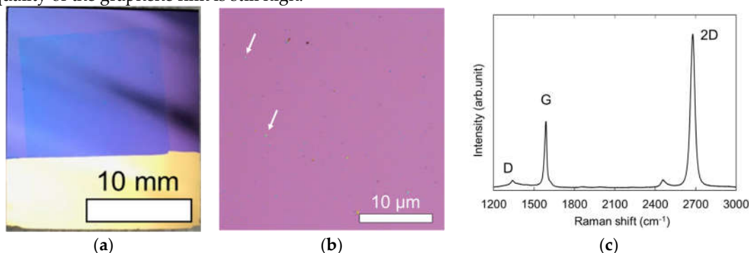
Figure 4. Characterization of the chemical vapor deposition (CVD)-grown graphene film on SiO 2 /Si substrate. (a) Optical image after deposition of the Au /Ni (50 nm/10 nm). (b) Optical micrograph. Arrows indicate poly-methyl methacrylate (PMMA) residues. (c) Raman spectrum.
