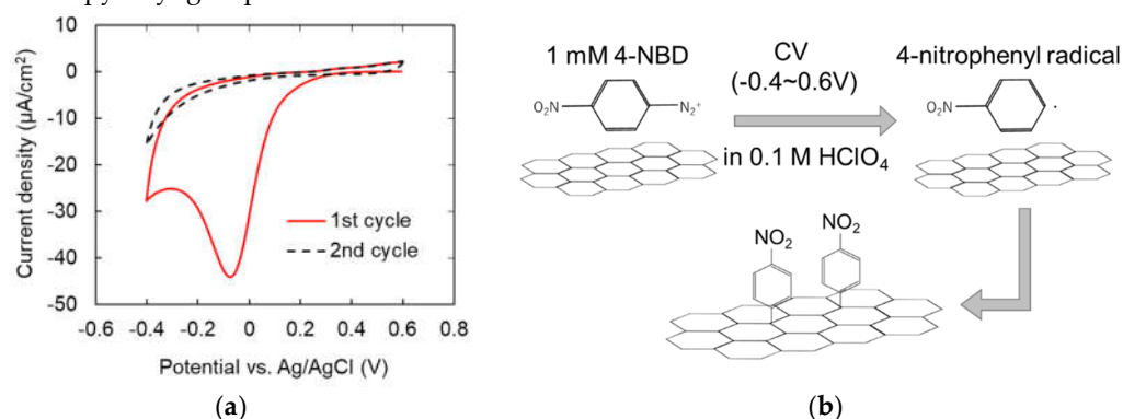
Figure 6. (a) CVs during covalent modification of CVD-grown graphene using 1 mM 4-Nitrobenzenediazonium tetrafluoroborate in 0.1 M \text{HClO}_4 at scan rate of 50 mV/s. (b) The schematic diagram of electrochemical covalent modification to the graphene surface.
