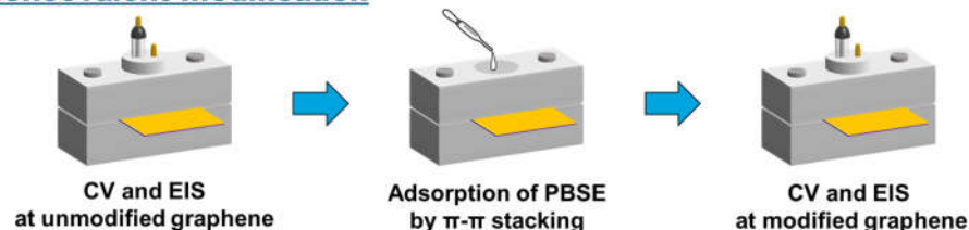
Figure 3. The measurement and modification schemes for evaluating influences of the covalent and noncovalent modifications on electrochemical properties of the graphene electrodes. The graphene electrodes were not dismantled from the cells in the whole process.
