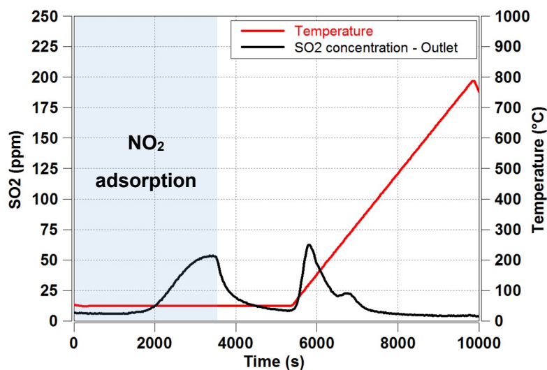
Figure S1. SO 2 desorption profile during TPD2 for Pt/Al 2 O 3 .
