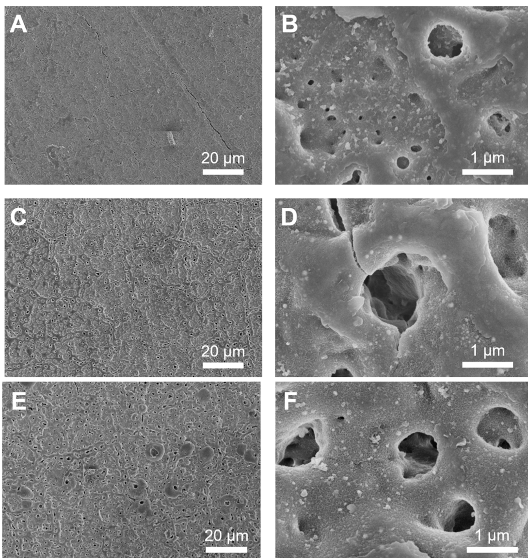
Figure 1. SEM images of Pd/MgO catalysts prepared by different applied voltages (a)(b) 300 V, (c)(d) 400 V, (e)(f) 500 V, respectively.
