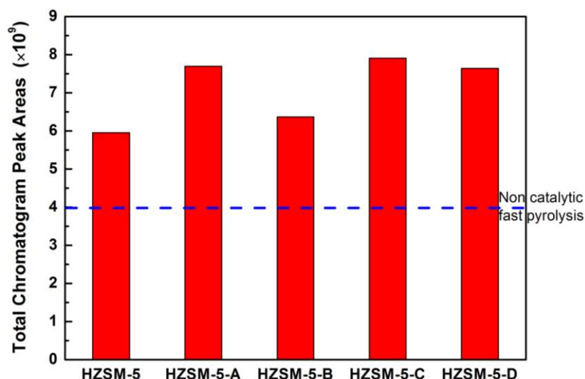
Figure 8. The total yield of the condensable volatiles from catalytic fast pyrolysis of Kraft lignin over parent HZSM-5 and the hierarchical HZSM-5 obtained by different post-treatment methods. Experimental conditions: pyrolysis temperature of 500 °C, Kraft lignin 0.3 mg, catalyst-to-lignin ratio of 10:1.
