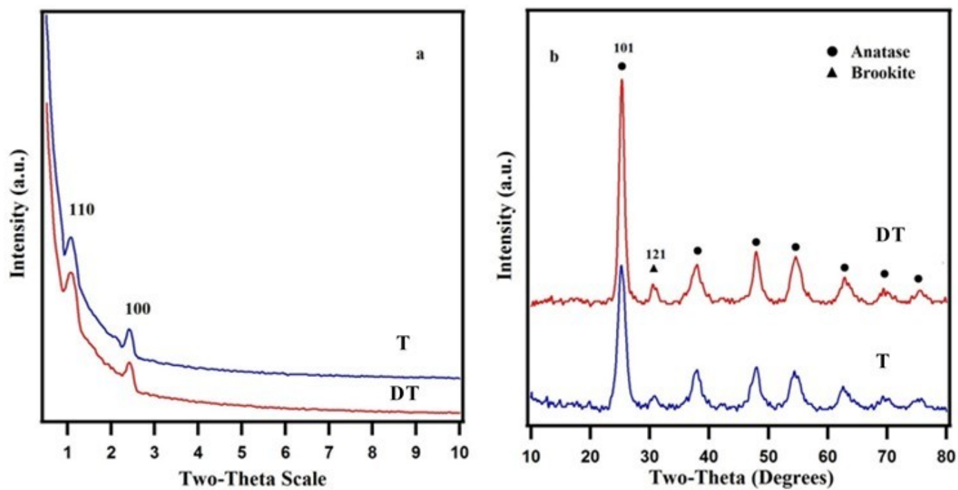
Figure S3. (a) Low angle XRD patterns and (b) Wide angle XRD patterns for the T and DT samples.
