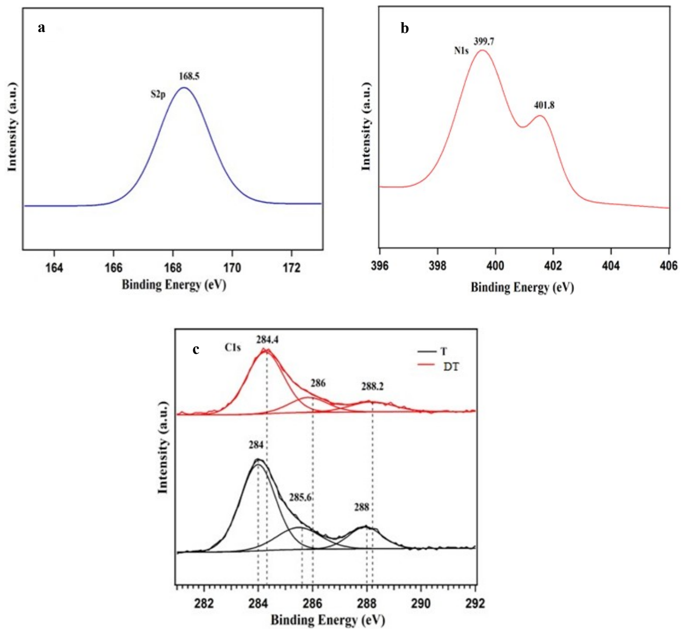
Figure S2. XPS detailed scans in the energy regions of (a) S2p, (b) N1s and (c) C1s for DT sample.
