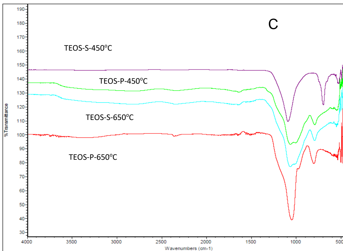
Figure S1: FTIR spectra of : (A) SiO 2 and treated with sulfuric acid SiO 2 -S and phosphoric acid SiO 2 -P, (B) TiO 2 and its treatment with sulfuric acid TiO 2 -S and phosphoric acid TiO 2 -P, and (C) silica prepared from TEOS treated with sulfuric and phosphoric acid calcined at 450 and 650°C.
