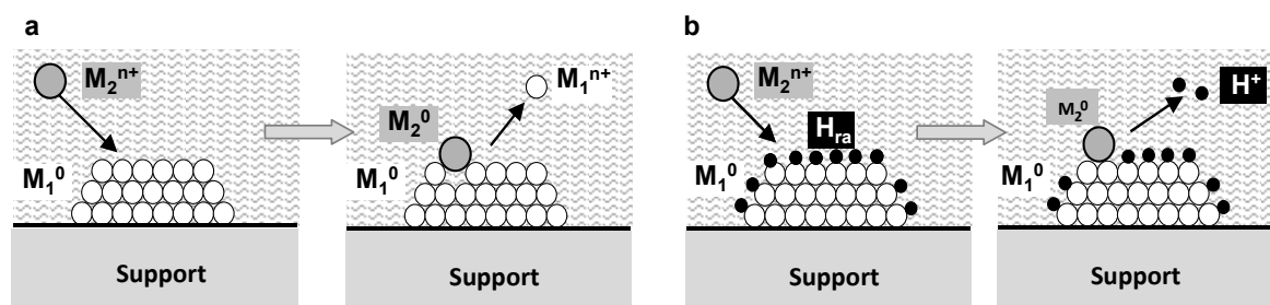
Figure 8. Schematic illustration of the surface redox methods: (a) Direct reduction of \text{M}_2^{n+} ions by \text{M}_1^0 metal particle, also called galvanic replacement reaction; (b) Reduction of \text{M}_2^{n+} ion by active H adsorbed on \text{M}_1^0 metal particle resulting from \text{H}_2 dissociation or activation of a reducing agent on \text{M}_1^0 .
