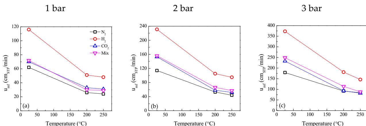
Figure 3. Evolution of minimum fluidization velocity with an increase in temperature. Solid: \alpha 13X; fluidizing agent: either N 2 , CO 2 , H 2 , or mixture; absolute pressure: (a) 1 bar, (b) 2 bar, and (c) 3 bar.
