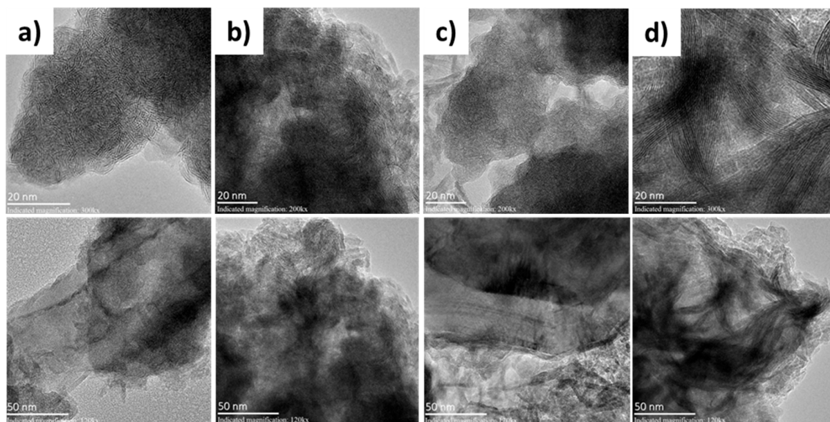
Figure 2. HR-TEM images of spent samples at (up) 20 nm and (down) 50 nm of (a) CoMoS/CNF-ox, (b) CoMoS/PANI, (c) CoMoS/r-GO and (d) CoMoS/g-C 3 N 4 composites after catalytic tests.
