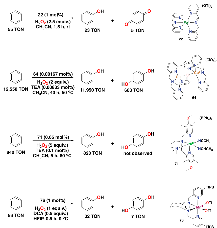
Figure 41. The best-performing catalysts per metal covered in this review are for the oxidation of benzene to phenol. Catalyst performance is expressed in terms of turnover numbers.
