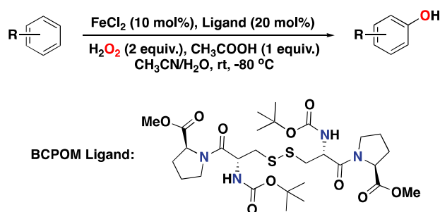
Figure 24. Arene oxidation reaction catalyzed by \text{FeCl}_2 , the L-cystine-derived BCPOM ligand, and \text{H}_2\text{O}_2 as an oxidant.
