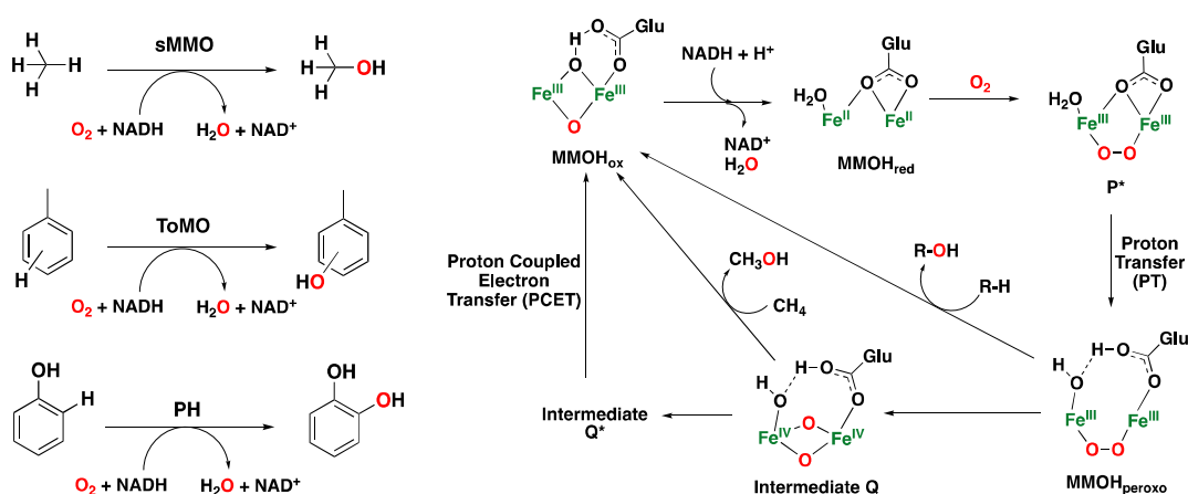
Figure 6. Left: Hydroxylation reactions catalyzed by some of the most representative bacterial multicomponent monooxygenases [14,121]. Right: catalytic mechanism of sMMO for dioxygen activation and substrate oxidation, involving the MMOH ox , MMOH red , intermediate P*, MMOH peroxo , and intermediate Q species [14,121,133].
