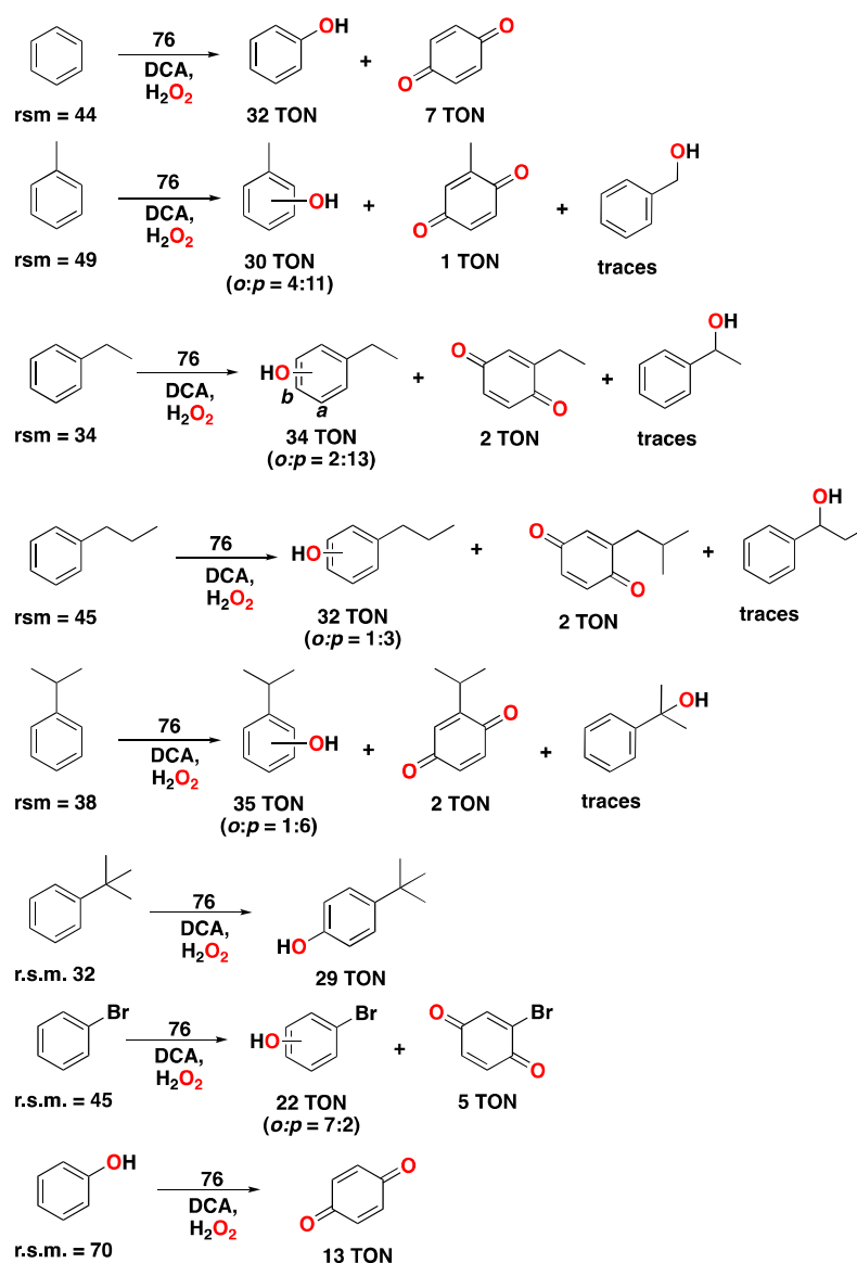
Figure 40. Reaction products of the catalytic oxidation of benzene and benzene derivatives catalyzed by complex 76 with \text{H}_2\text{O}_2 as an oxidant and DCA as a carboxylic acid additive. Reaction conditions: complex 76 (1 mol%), substrate, \text{H}_2\text{O}_2 (1.0 equiv., slow addition in 30 min), and DCA (0.5 equiv.) in HFIP at 0 °C for 0.5 h. See the corresponding reference for further details on the oxidation of other alkylbenzene substrates [316]. rsm = remaining starting material (%).
