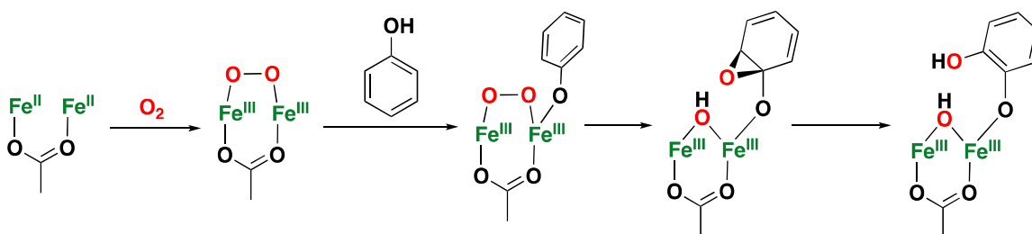
Figure 7. Schematic representation of the mechanism of PH for dioxygen activation and phenol hydroxylation. A similar mechanism is postulated for toluene hydroxylation; however, substrate oxidation is controlled by residues of the active site rather than by coordination with the diiron core [140].
