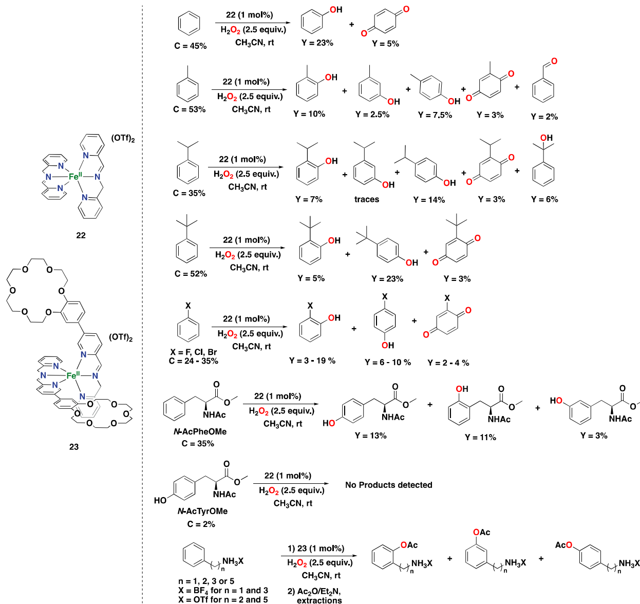
Figure 18. Reaction products of the catalytic oxidation of benzene, benzene derivatives, and aromatic amino acids catalyzed by iminopyridine iron(II) complexes 22 and 23 with H 2 O 2 as an oxidant [214–216]. C: substrate conversion. Y: product yield.
