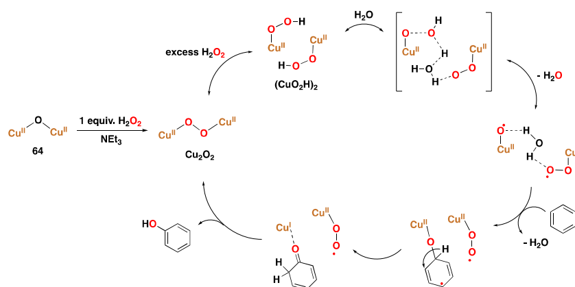
Figure 31. Proposed mechanism for the activation of \text{H}_2\text{O}_2 and hydroxylation of benzene to phenol catalyzed by complex 64 supported by the 6-hpa ligand [285].
