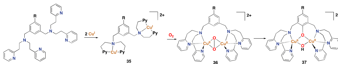
Figure 26. Representative synthetic copper complex 35 inspired by tyrosinase oxidase, reported by Karlin et al. [246–248]. Upon complexation of copper with the dinucleating aminopyridine ligand, reaction with dioxygen leads to a side-on (μ-η 2 :η 2 ) peroxo copper intermediate that can perform an intramolecular aromatic hydroxylation. Py = pyridine; R = H, MeO, t Bu, F, CN, NO 2 .
