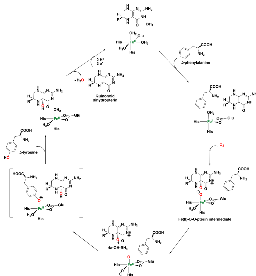
Figure 9. Proposed catalytic mechanism for phenylalanine hydroxylases (PheOH) [23,34].
