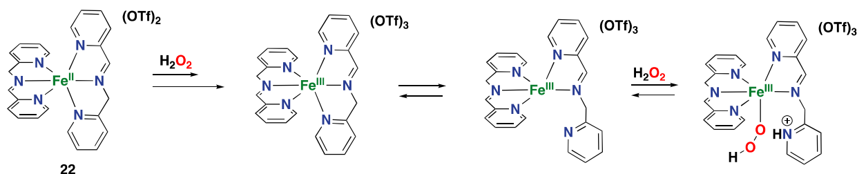
Figure 19. Proposed mechanism for H 2 O 2 activation with iminopyridine iron(II) complex 22 [220].
