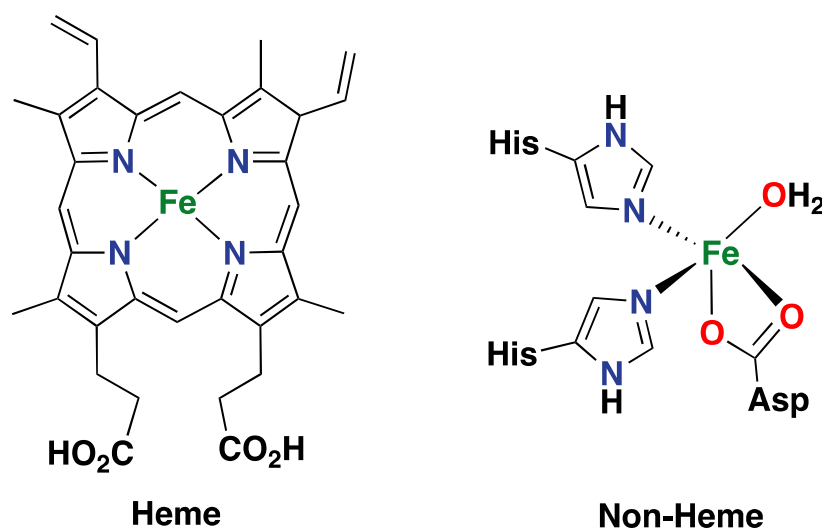
Figure 3. Schematic diagram of the typical heme prosthetic group (iron protoporphyrin IX) found in the active site of heme enzymes ( left ) [69,70] and of the 2-His-1-carboxylate facial triad active site found in the mononuclear non-heme enzyme naphthalene dioxygenase (NDO; right ) [26,34,71,72].
