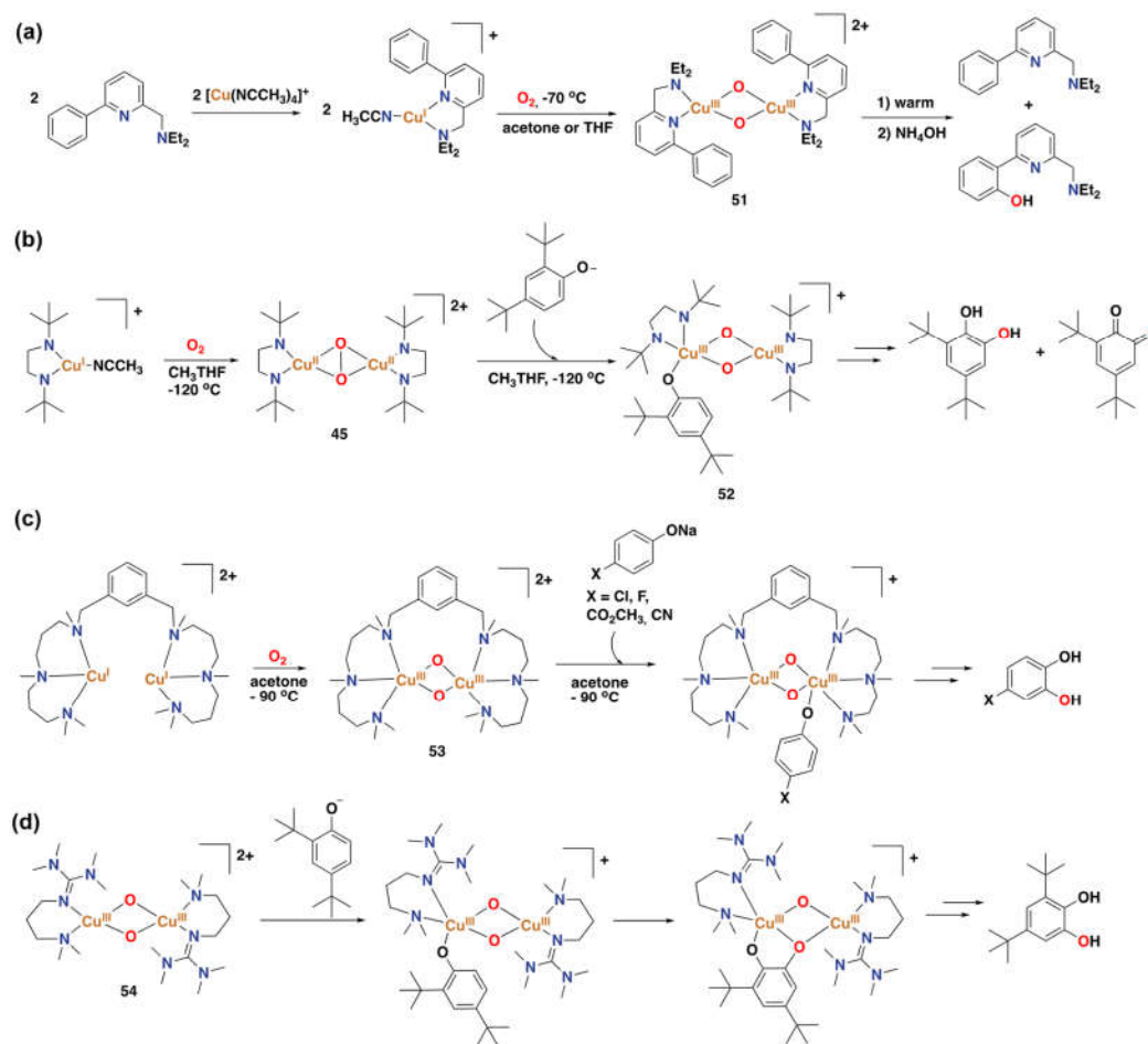
Figure 28. (a) Synthesis of a copper(I) complex that performs the hydroxylation of an arene of the ligand upon reaction with dioxygen through the bis( \mu -oxo)dicopper(III) intermediate 51 [276]. (b) Mechanism of phenolate oxidation by a mononuclear copper(I) complex, involving the formation of intermediates 45 and 52 [269]. (c) Mechanism of phenolate oxidation by a dinuclear copper(I) complex, involving a bis( \mu -oxo)dicopper(III) intermediate 53 [263]. (d) The reaction of bis( \mu -oxo)dicopper(III) complex 54 with phenolates to afford catechol products [277].
