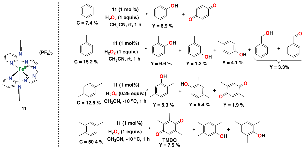
Figure 16. Reaction products of the catalytic oxidation of benzene and benzene derivatives catalyzed by NHC-based iron complex 11 , with H 2 O 2 as the oxidant [207,211]. C: substrate conversion. Y: product yield.
