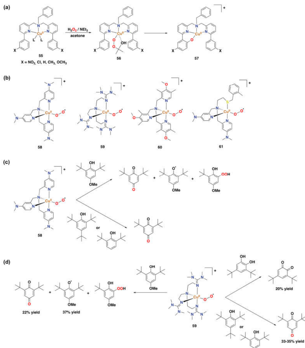
Figure 29. (a) Aromatic hydroxylation reactivity of a mononuclear copper(II)-alkylperoxo complex [279,280]. (b) Selected end-on bound superoxo copper(II) complexes [250,251,253,254]. (c) Reactivity of complex 58 towards phenol substrates [250]. (d) Reactivity of complex 59 towards phenol substrates [251].
