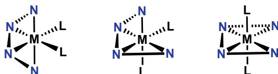
Figure 10. Different topologies for complexes with linear tetradentate aminopyridine ligands. L is an open coordination site.
