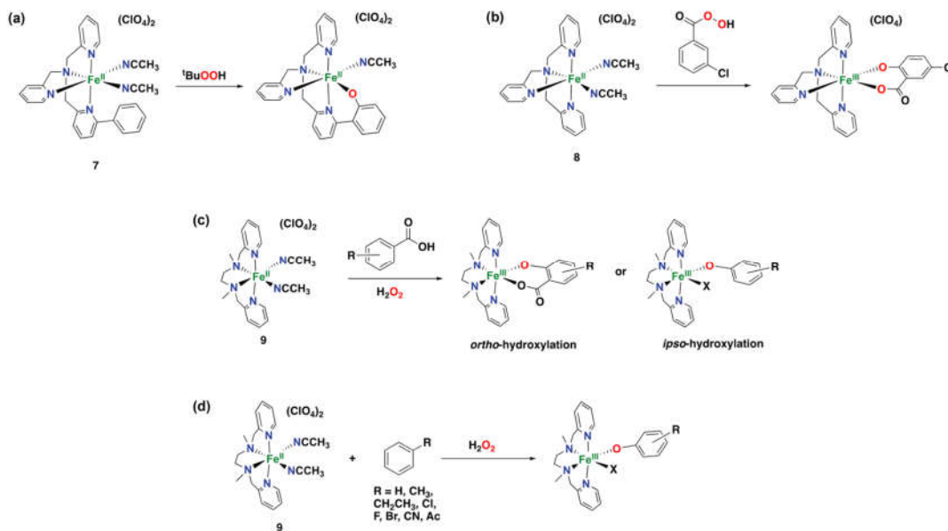
Figure 14. Iron(II) complexes are capable of performing arene hydroxylation reactions with different oxidants, generating phenolate or salicylate species. (a) Intramolecular hydroxylation of a monomeric iron complex supported by a modified tpa ligand. (b) Oxidation of perbenzoic acid with an iron-tpa complex complex. (c) Oxidation of benzoic acids with an iron-bpmen complex. (d) Oxidation of aromatic substrates without directing groups with an iron-bpmen complex.
