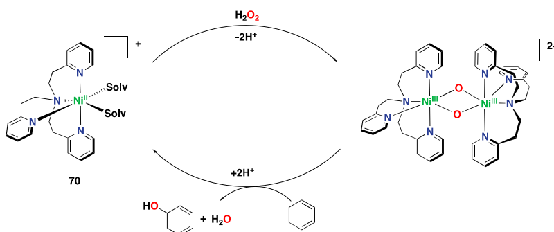
Figure 36. Proposed catalytic mechanism for the direct hydroxylation of benzene to phenol catalyzed by nickel(II) complex 70 supported by a tripodal tetradentate aminopyridine ligand and involving a bis( \mu -oxo)dinickel(III) intermediate [301].
