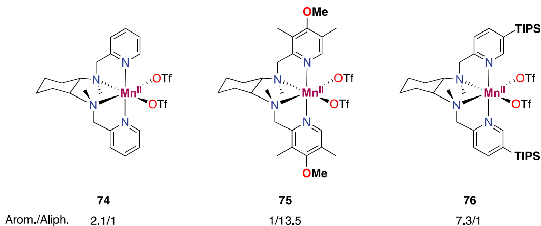
Figure 39. bpmcn-based Mn-complexes studied in the oxidation of propylbenzene [314]. Ratio Arom./Aliph. represents the ratio between aromatic and aliphatic oxidation products.
