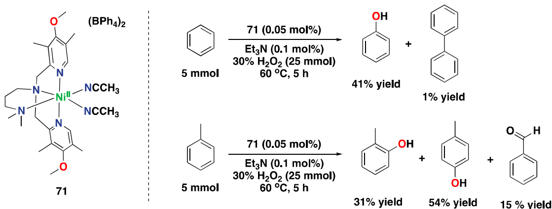
Figure 37. Reaction products of the catalytic oxidation of benzene and toluene catalyzed by nickel(II) complex 71 with \text{H}_2\text{O}_2 as an oxidant and triethylamine as an additive.
