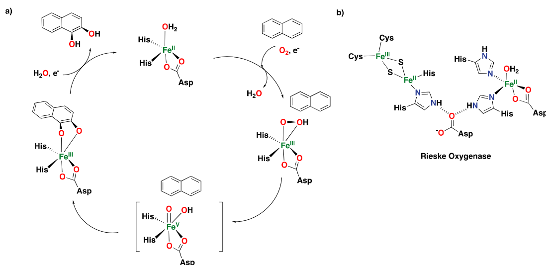
Figure 5. (a) Proposed catalytic cycle for the oxidation of naphthalene catalyzed by Rieske dioxygenases, involving the generation of an Fe(V)(O)(OH) species. (b) Active site of naphthalene 1,2-dioxygenase (NDO), showing the Rieske [2Fe:2S] cluster (reductase component) and the catalytic iron center (oxygenase component) [113].
