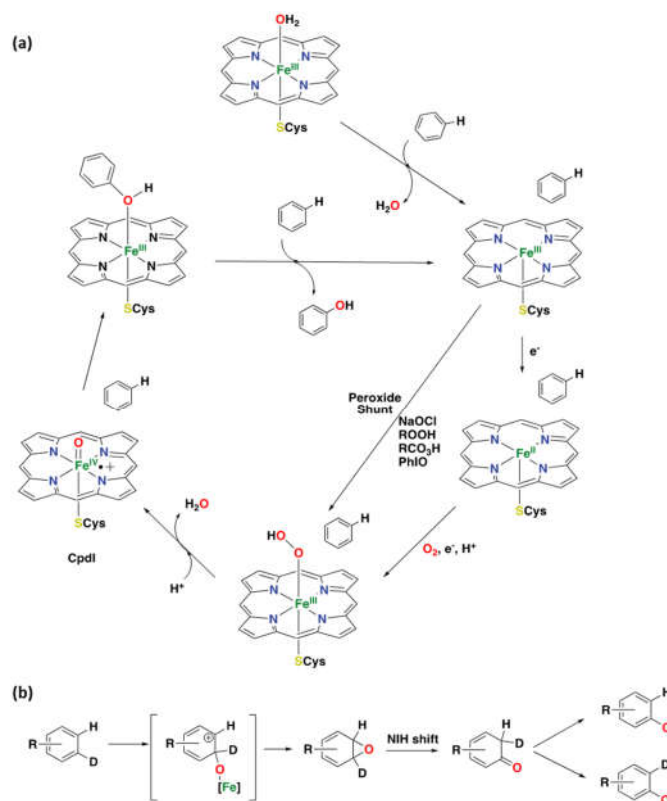
Figure 4. (a) Established catalytic cycle for arene oxidation is catalyzed by cytochrome P450 [73,94,106–108]. (b) Oxidation of deuterated aromatic compounds catalyzed by cytochrome P450, illustrating the “NIH shift” process [106,109].
