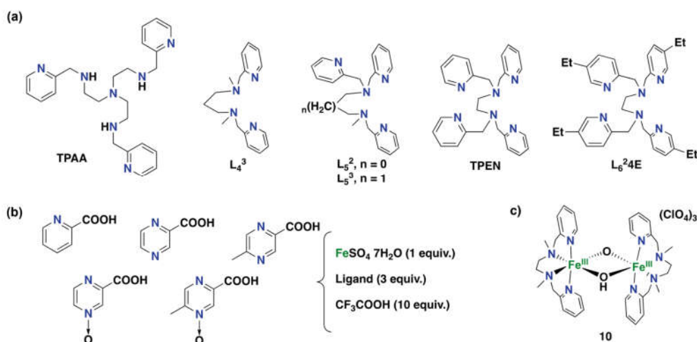
Figure 15. (a) Aminopyridine ligands were studied in iron-mediated arene hydroxylation reactions under substrate-excess conditions in the presence of a reductant [200–202]. (b) Three-component system for the hydroxylation of aromatics using a biphasic reaction medium under substrate-excess conditions [203–205]. (c) Example of a diiron complex that mimics the reactivity of toluene monooxygenases [206].
