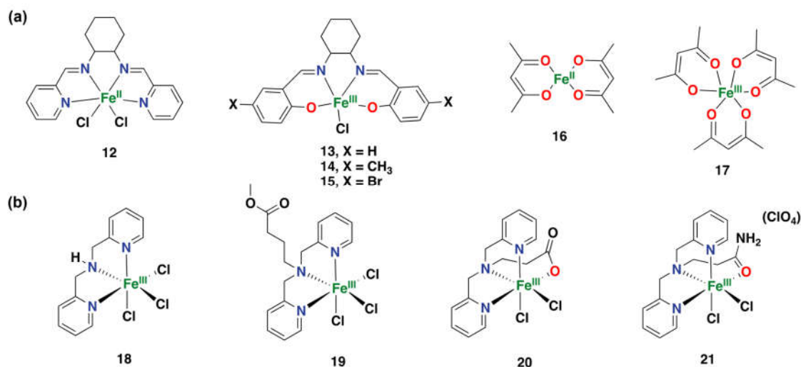
Figure 17. (a) Iron complexes supported by acetylacetonate and Schiff base ligands were tested for the direct aromatic hydroxylation of benzene to phenol with H 2 O 2 [42]. (b) Iron(III) complexes were tested for the hydroxylation of toluene with H 2 O 2 as an oxidant [212].
