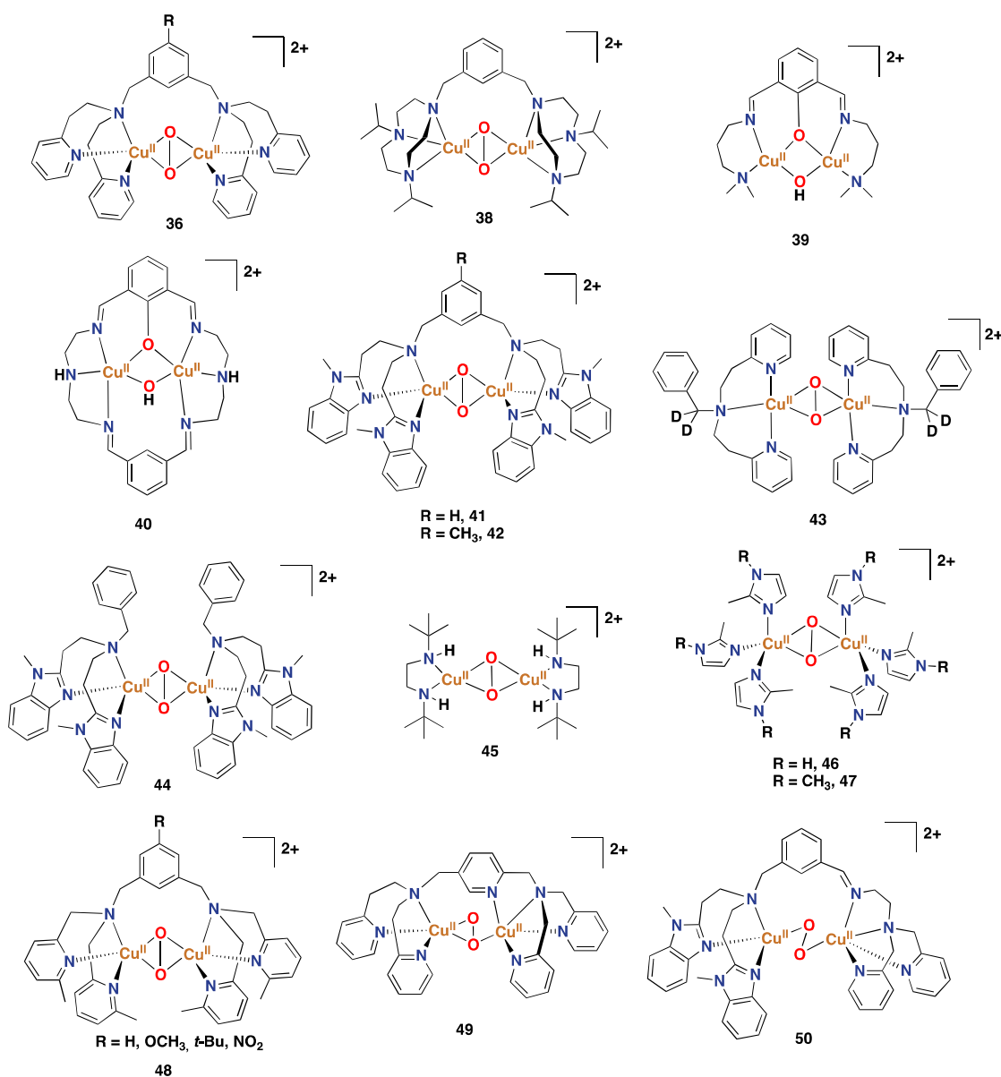
Figure 27. Selected examples of dicopper(II) dioxygen complexes (supported by mono- and dinucleating ligands as well as non-symmetrical dinucleating ligands) that mimic the activity of tyrosinase [255–266].
