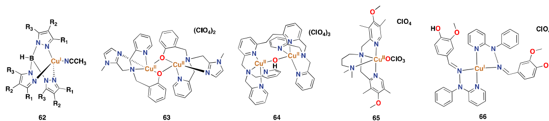
Figure 30. Synthetic copper complexes display catalytic activity for the hydroxylation of aromatic substrates through a metal-based mechanism [282,284–286,288].
