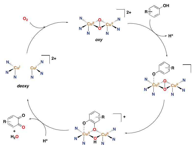
Figure 25. Oxidation of monophenols to o -quinones catalyzed by tyrosinase oxidase [14,106,241,242,245].
