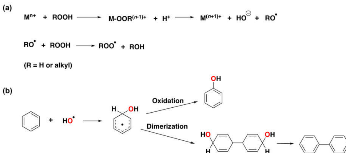
Figure 2. (a) Generation of free diffusing oxygen-centered radicals via the initial Fenton reaction. (b) Hydroxylation of benzene by addition of hydroxyl radicals to generate phenol and biphenyl.
