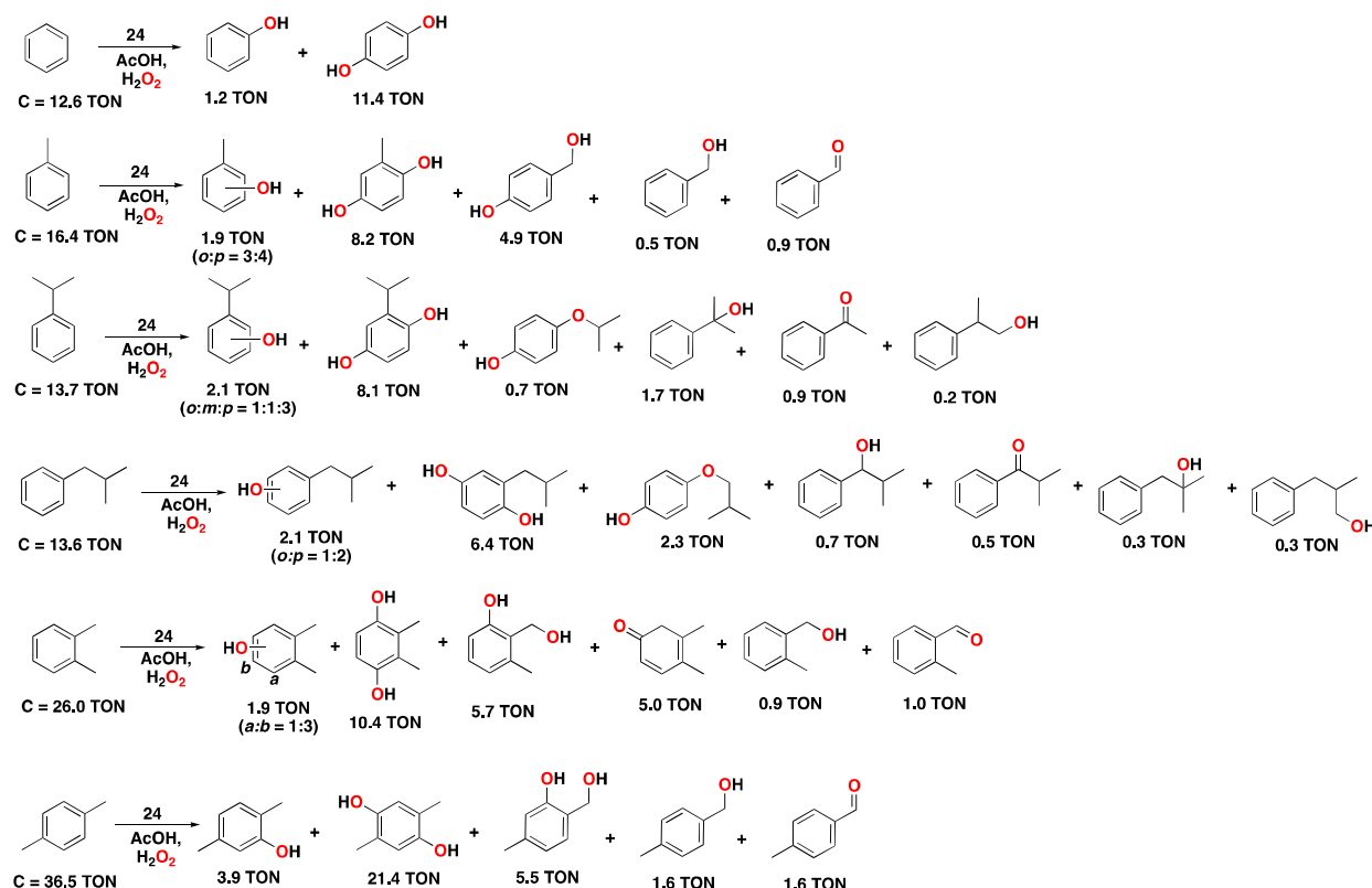
Figure 21. Reaction products of the catalytic oxidation of benzene and benzene derivatives catalyzed by diferric complex 24 as catalyst with \text{H}_2\text{O}_2 as an oxidant and AcOH as a carboxylic acid additive. Reaction conditions: complex 24 (0.62 mol% cat./1.24 \mu\text{mol} Fe), substrate (100 \mu\text{mol} ), \text{H}_2\text{O}_2 (400 \mu\text{mol} ), and AcOH (1000 \mu\text{mol} ) in \text{CH}_3\text{CN} at 0 °C for 1.5 h. See the corresponding reference for further details on the oxidation of other alkylbenzene substrates [221].
