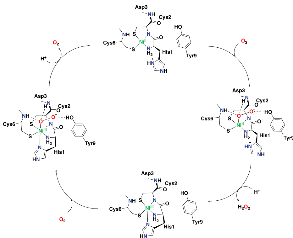
Figure 33. Catalytic cycle of nickel superoxide dismutase (NiSOD) [31].
