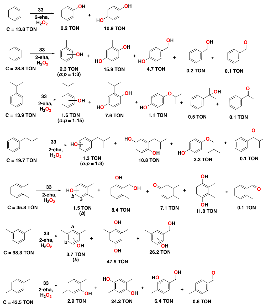
Figure 23. Reaction products of the catalytic oxidation of benzene and benzene derivatives catalyzed by complex 33 with \text{H}_2\text{O}_2 as an oxidant and 2-eha as a carboxylic acid additive. Reaction conditions: complex 33 (1.24 \mu\text{mol} Fe), substrate (100 \mu\text{mol} ), \text{H}_2\text{O}_2 (400 \mu\text{mol} ), and 2-eha (1000 \mu\text{mol} ) in \text{CH}_3\text{CN} at 0 ^\circ\text{C} for 1.5 h. See the corresponding reference for further details on the oxidation of other alkylbenzene substrates [229]. 2-eha = 2-ethylhexanoic acid.
