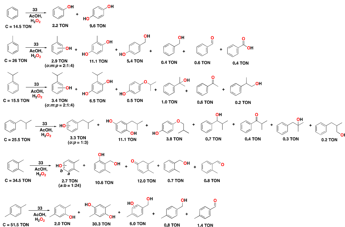
Figure 22. Reaction products of the catalytic oxidation of benzene and benzene derivatives catalyzed by complex 33 as catalyst with \text{H}_2\text{O}_2 as an oxidant and AcOH as a carboxylic acid additive. Reaction conditions: complex 33 (1.24 \mu\text{mol} Fe), substrate (100 \mu\text{mol} ), \text{H}_2\text{O}_2 (400 \mu\text{mol} ), and AcOH (1000 \mu\text{mol} ) in \text{CH}_3\text{CN} at 0^\circ\text{C} for 1.5 h. See the corresponding reference for further details on the oxidation of other alkylbenzene substrates [228].
