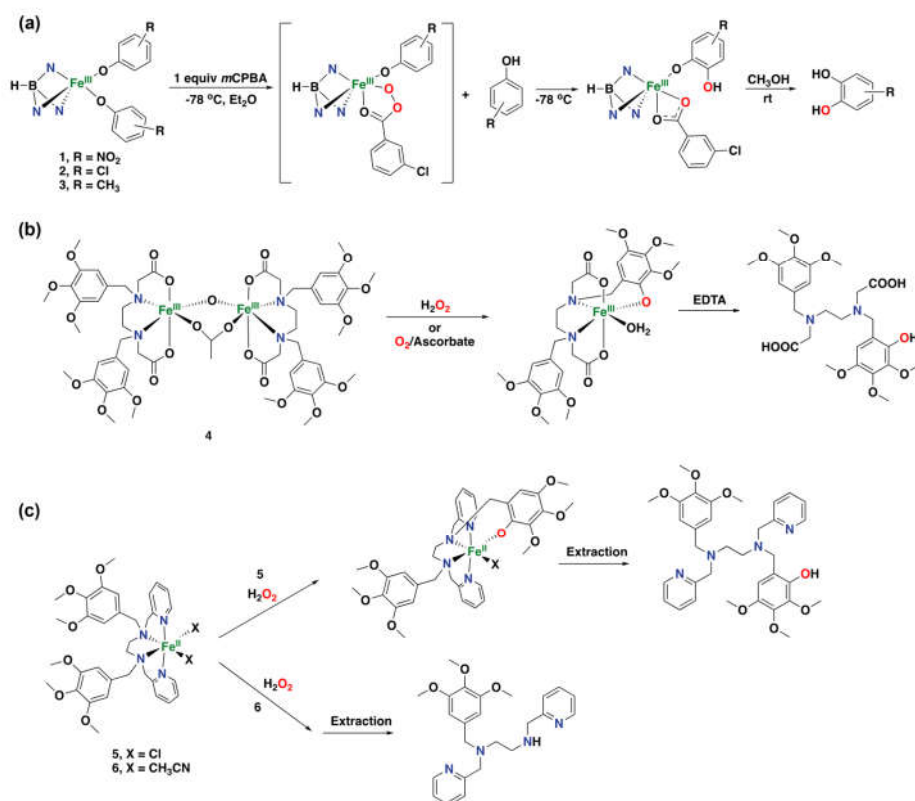
Figure 13. Early examples of iron complexes capable of intramolecular aromatic hydroxylation of the organic ligand. (a) Hydroxylation of trispyrazolylborate-based ferric bis-phenoxo complexes using mCPBA. (b) Intramolecular hydroxylation of a diiron complex to form a monomeric iron species. (c) Intramolecular hydroxylation of a series of iron complexes to yield the corresponding hydroxylated ligand.
