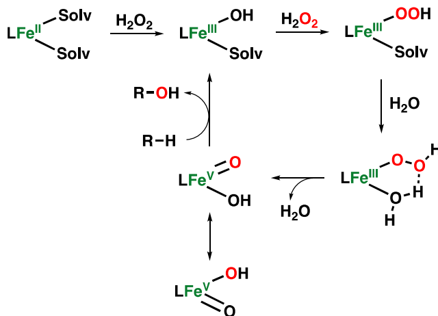
Figure 11. Water-assisted mechanism is proposed for the generation of an \text{Fe(V)(O)(OH)} species in hydroxylation reactions catalyzed by non-heme iron complexes supported by strong-field tetradentate aminopyridine ligands with two cis open sites.
