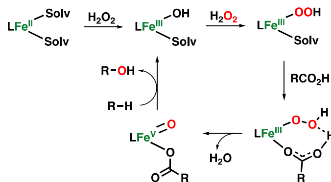
Figure 12. Carboxylic acid-assisted mechanism is proposed for the generation of an \text{Fe(V)}(\text{O})(\text{OCOR}) species in the hydroxylation reaction catalyzed by non-heme iron complexes supported by strong-field tetradentate aminopyridine ligands with two cis open sites.
