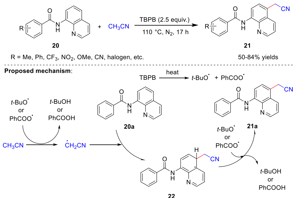
Scheme 6. Cyanomethylation with TBPB as the oxidant.
