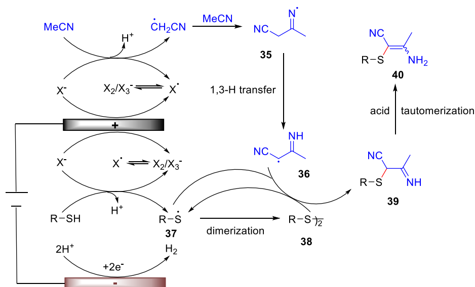
Scheme 13. Mechanism of electrochemical synthesis of tetrasubstituted olefins from acetonitrile and thiols.
