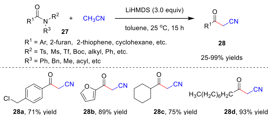
Scheme 9. Cyanomethylation of acetonitrile with amides.
