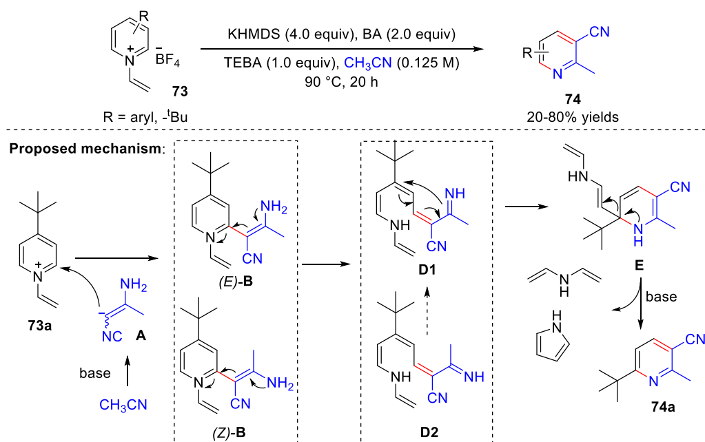
Scheme 18. Synthesis of 3-cyanopyridine.
