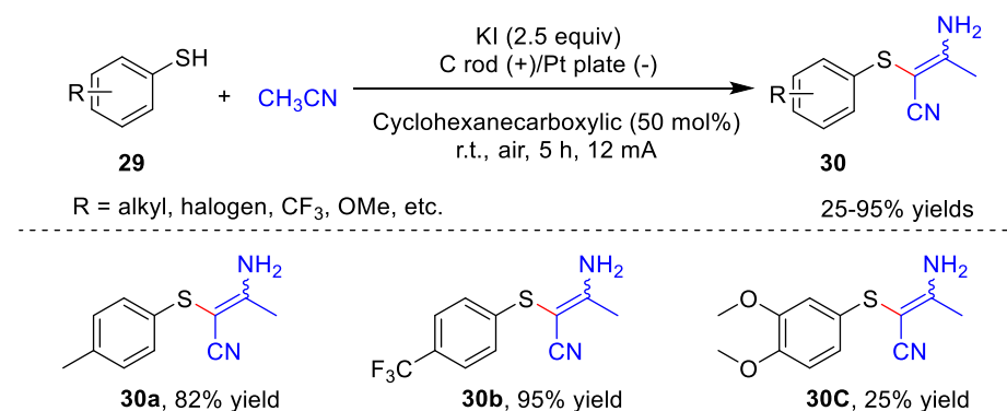
Scheme 10. Synthesis of tetrasubstituted olefins by thiophenol and acetonitrile.
