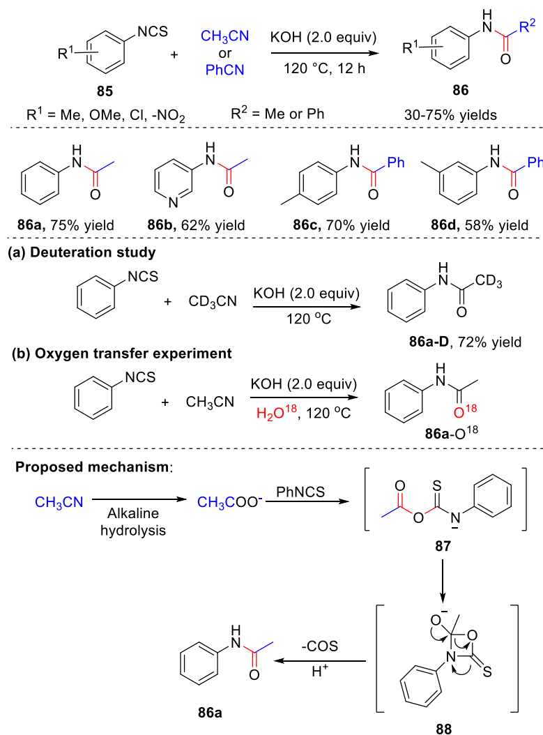
Scheme 20. Synthesis of amide by acetonitrile and isothiocyanate.
