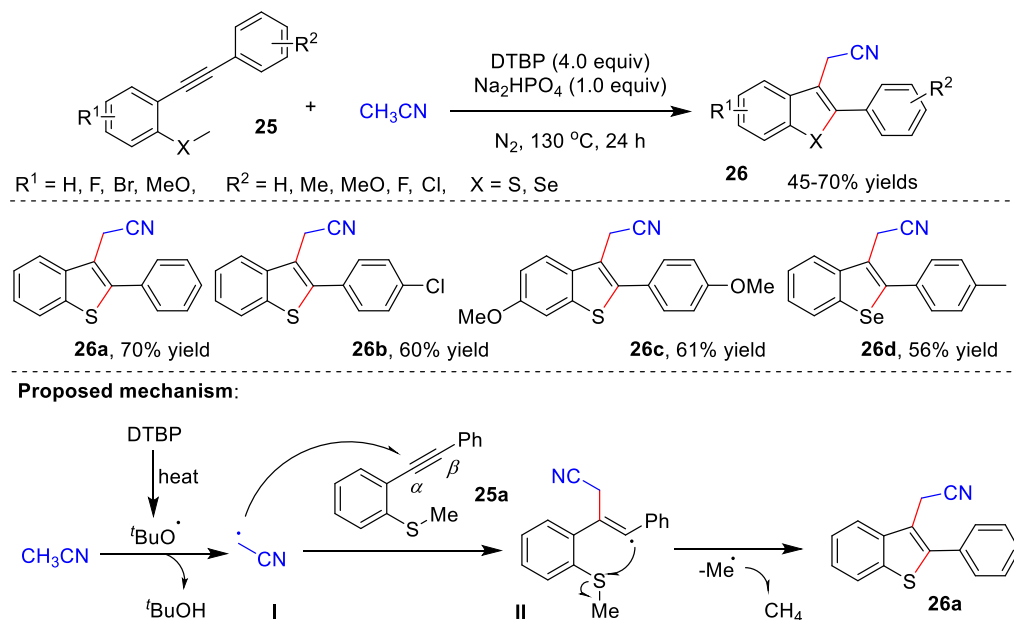
Scheme 8. Cascade radical cyclization of alkynes with acetonitrile.
