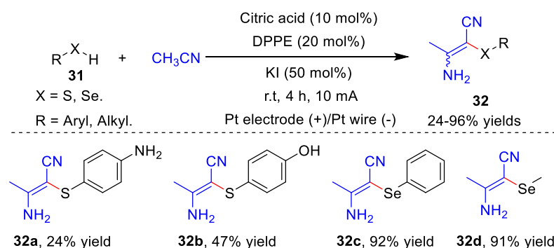
Scheme 11. Synthesis of tetrasubstituted olefins via thiophenol and acetonitrile.
