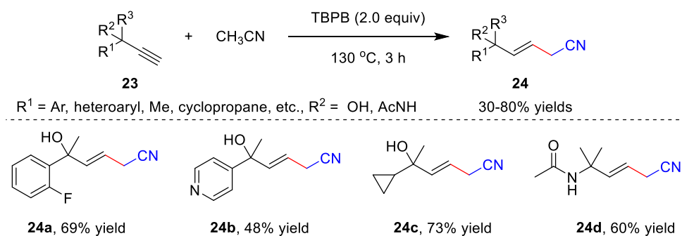
Scheme 7. Addition of acetonitrile to alkynes.
