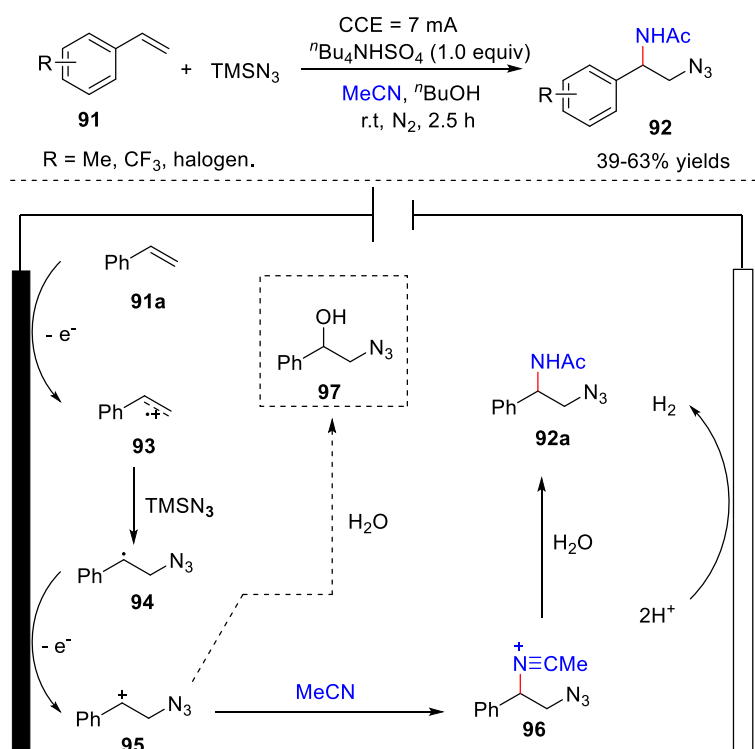
Scheme 22. Electrochemical synthesis of vicinal azidoacetamides.
