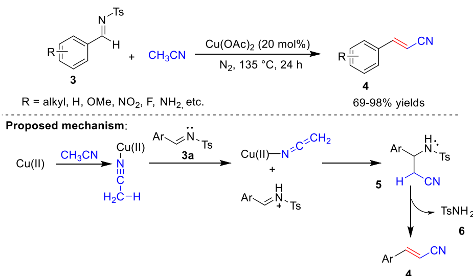
Scheme 2. Cu-catalyzed cyanomethylation.
