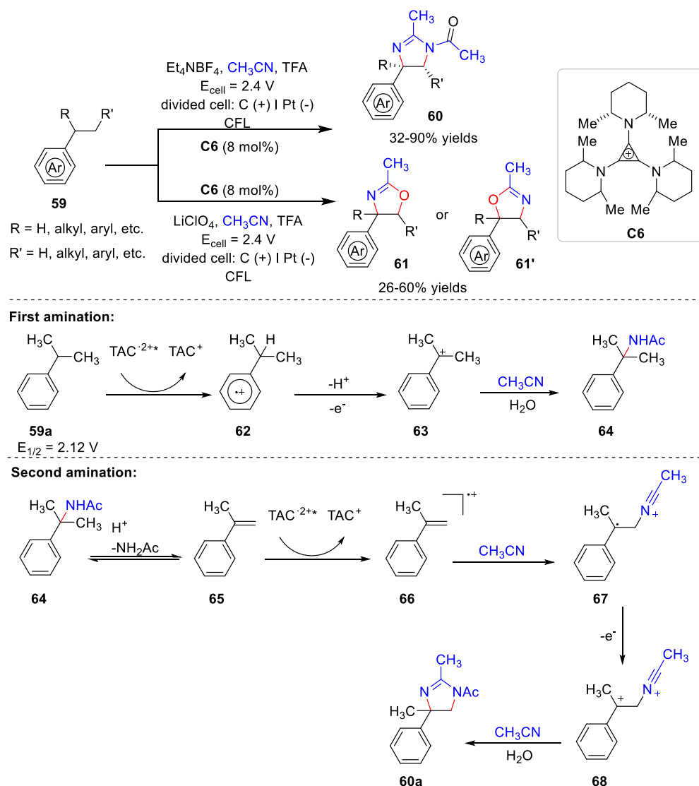
Scheme 16. Synthesis of dihydroimidazoles and 2-oxazolines.
