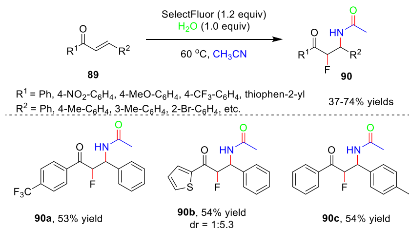
Scheme 21. Aminofluorination of \alpha,\beta -unsaturated ketones.
