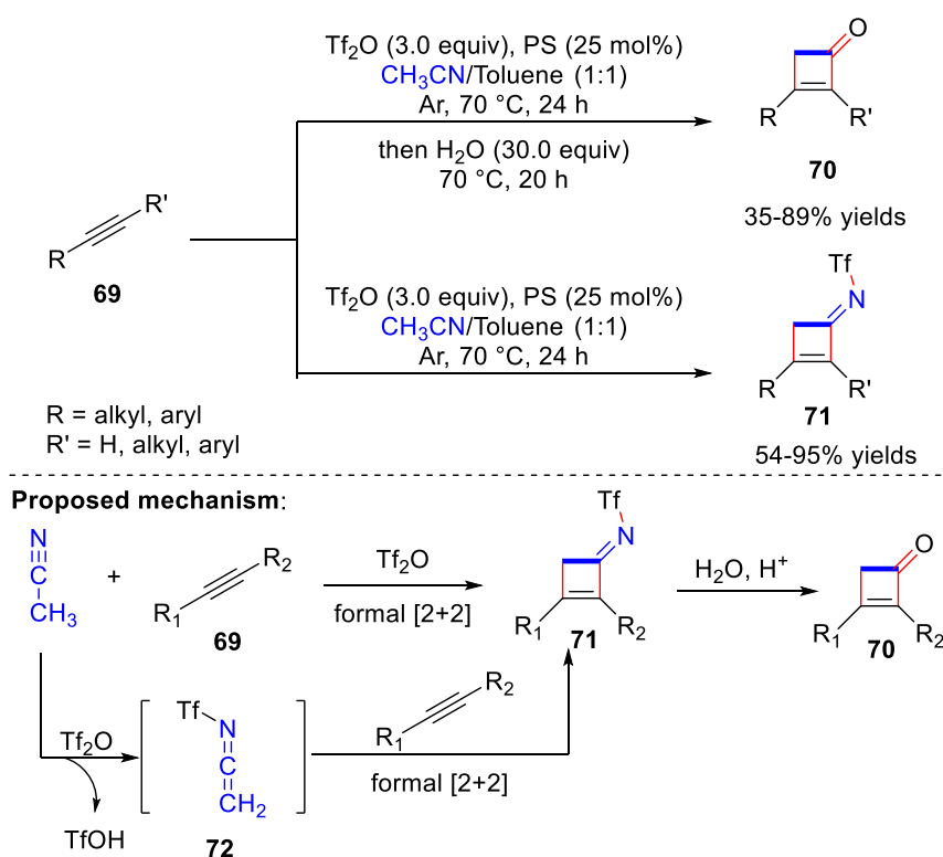
Scheme 17. Synthesis of cyclobutenone.
