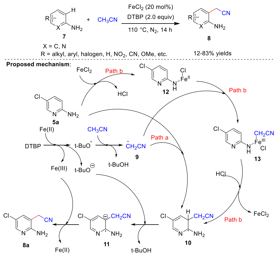
Scheme 3. Fe-catalyzed cyanomethylation.
