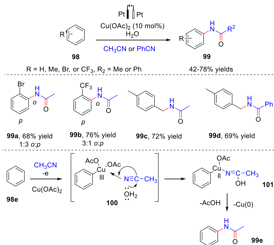
Scheme 23. Electrochemical synthesis of amides catalyzed by copper.
