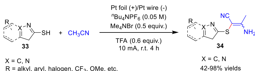
Scheme 12. Synthesis of tetrasubstituted olefins by acetonitrile and heteroaryl thiols.
