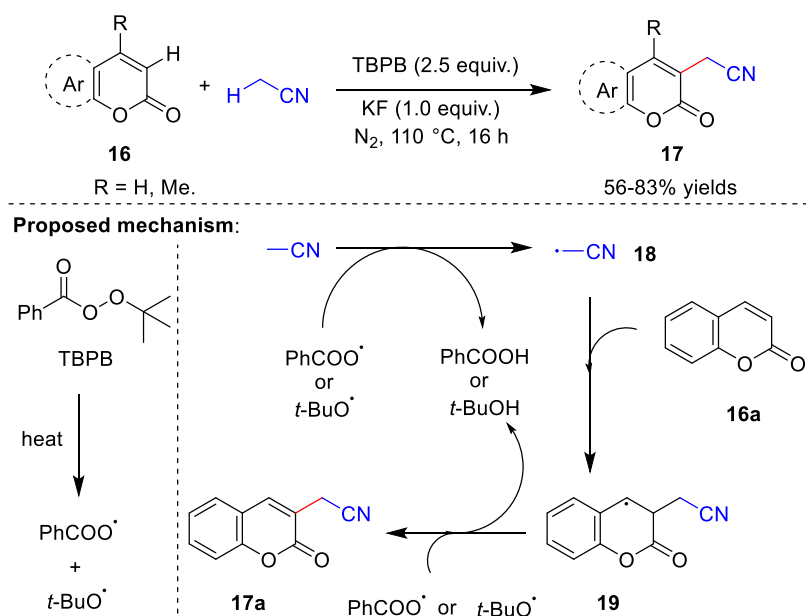
Scheme 5. Cyanomethylation with TBPB as the oxidant.
