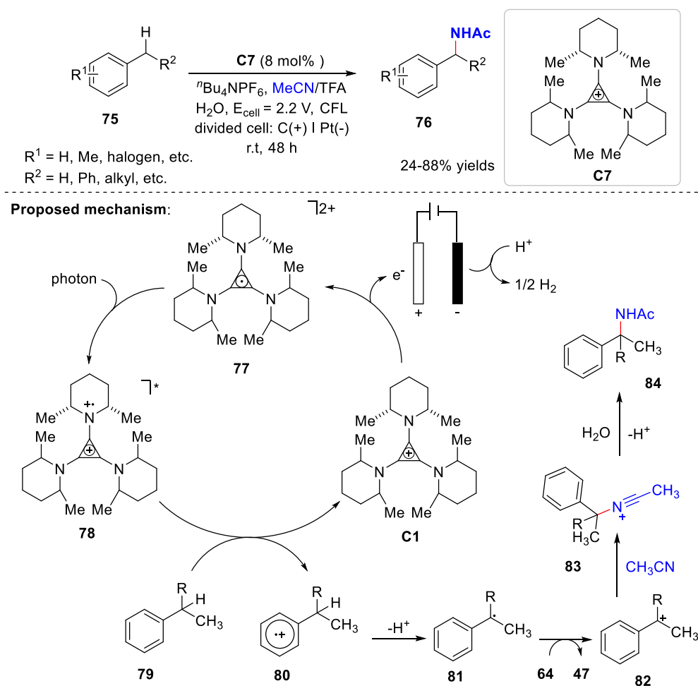
Scheme 19. Synthesis of amide by electrophotocatalytic reaction.
