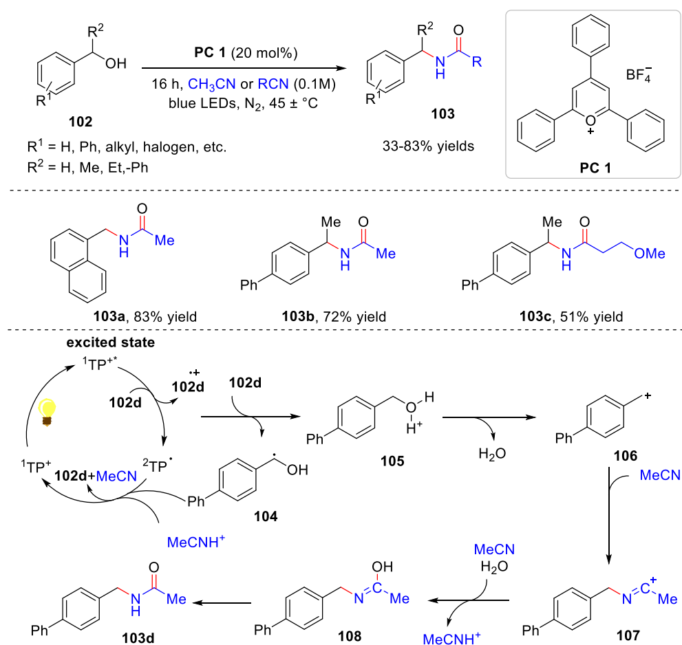
Scheme 24. Photocatalytic synthesis of amide.
