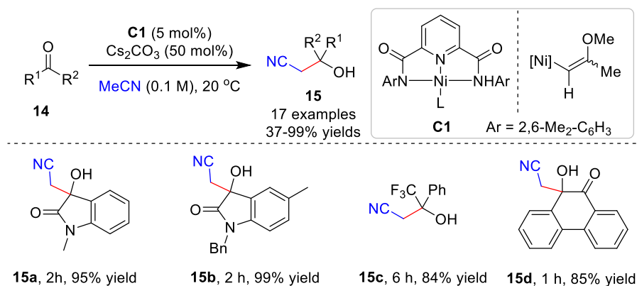
Scheme 4. Ni-catalyzed cyanomethylation.
