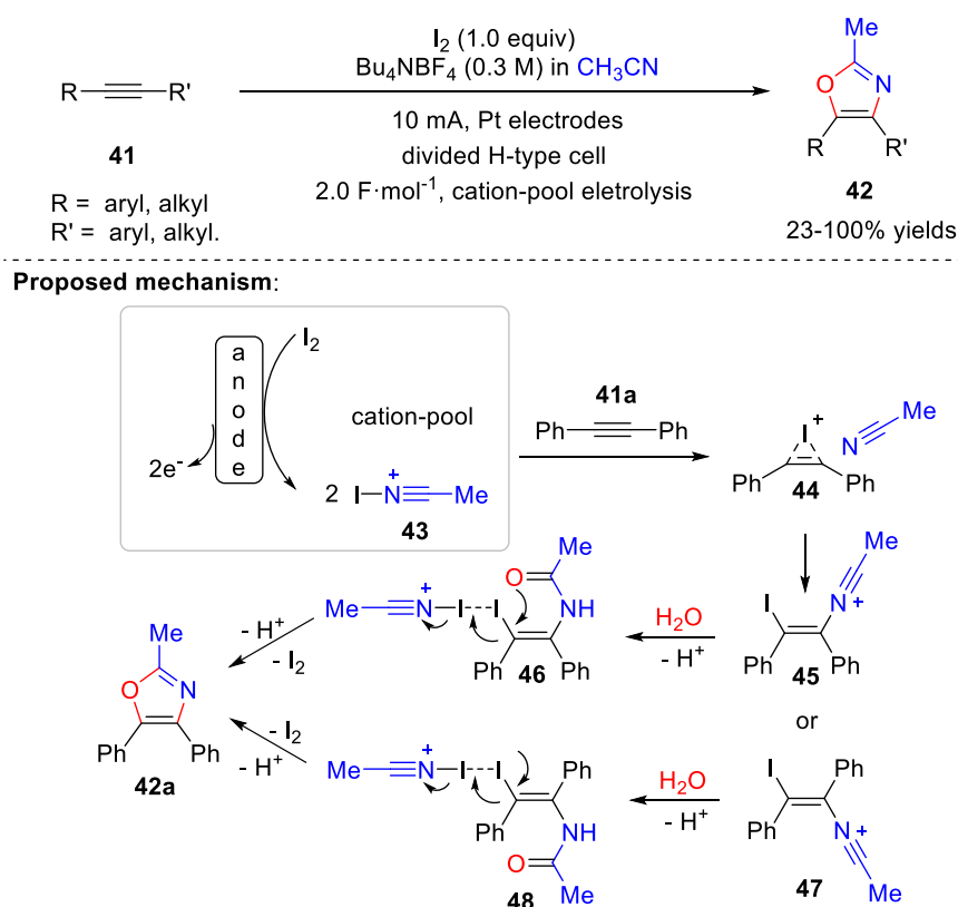
Scheme 14. Synthesis of 1,3-oxazoles from alkynes and acetonitrile.
