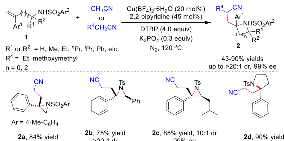
Scheme 1. Cu-catalyzed cyanoalkylative aziridination of N -sulfonyl allyl amines.
