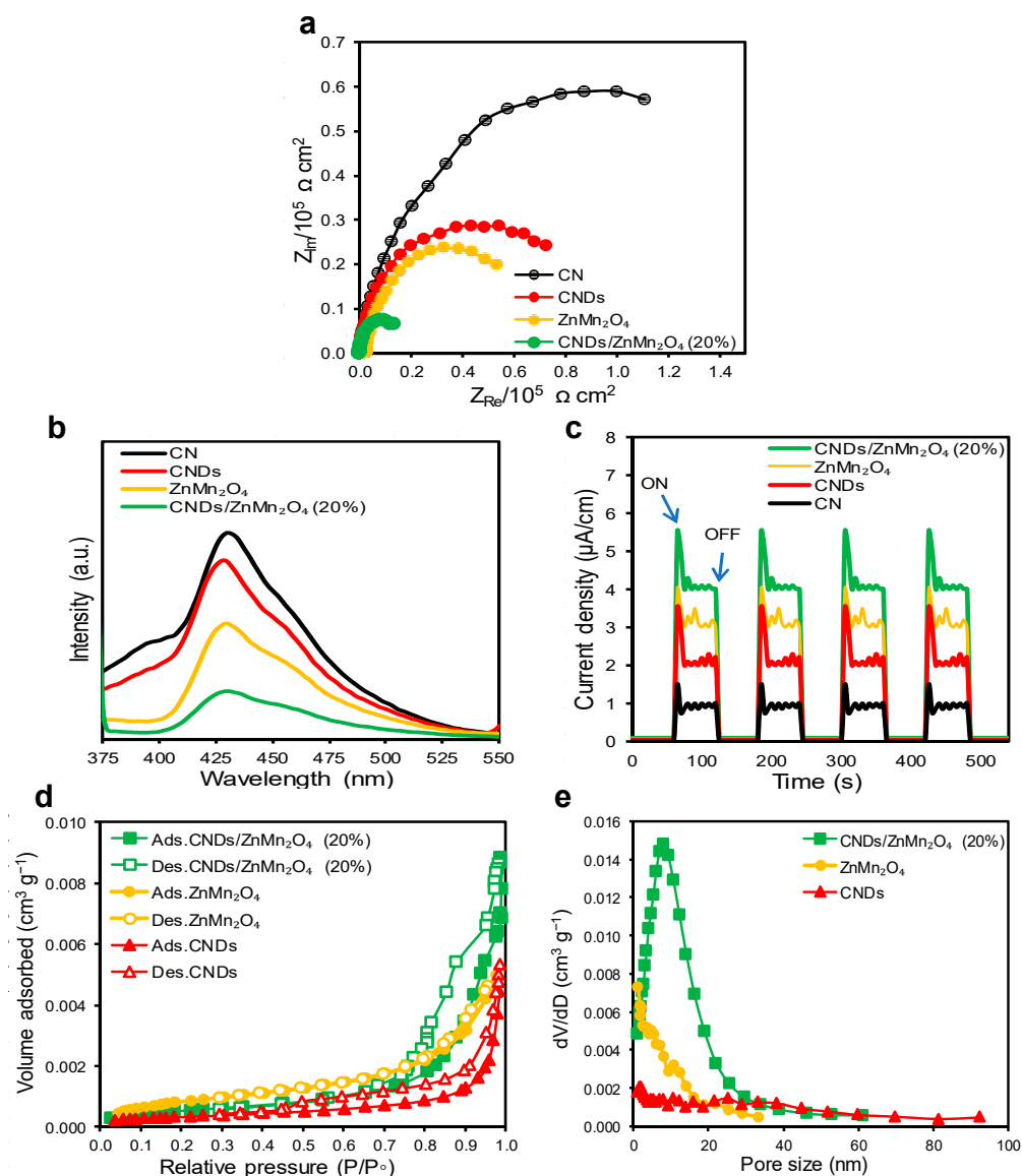
Figure 5. (a) EIS, (b) PL, and (c) Photocurrent of CN, CNDs, ZnMn 2 O 4 , and CNDs/ZnMn 2 O 4 (20%) photocatalysts. (d) N 2 sorption data and (e) pore-size distributions for CNDs, ZnMn 2 O 4 , and CNQDs/ZnMn 2 O 4 (20%) photocatalysts.
