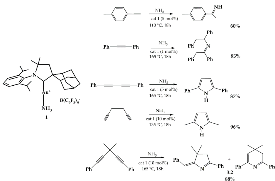
Scheme 3. Cationic gold-catalyzed hydroamination of alkynes with NH 3 .
