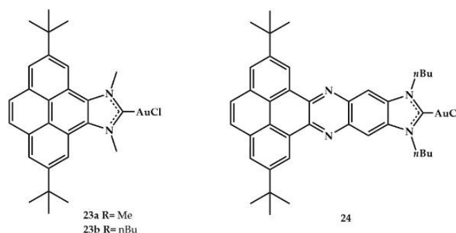
Figure 10. Gold(I) complexes with fused polycyclic aromatic hydrocarbons as ligands.
