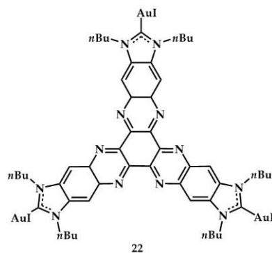
Figure 9. Gold complex with hexaazatriphenylene core.
