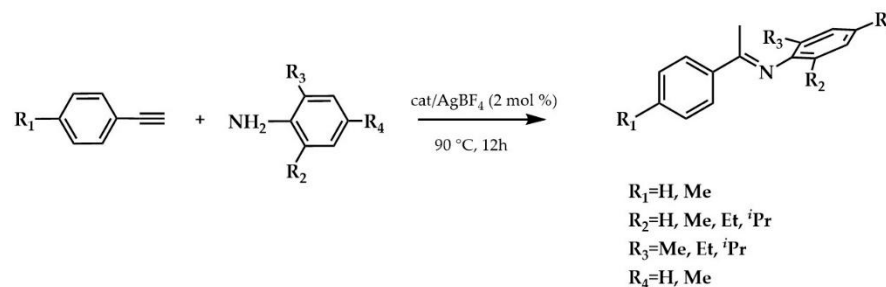
Scheme 4. Hydroamination reaction of o / p -substituted aryl amines with terminal alkynes.
