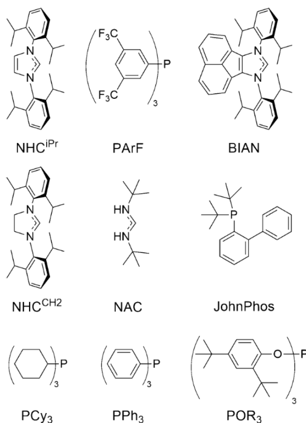
Figure 18. Structure of ligands used by Zuccaccia et al. Reprinted with permission from Ref. [60] Copyright 2016 American Chemical Society.
