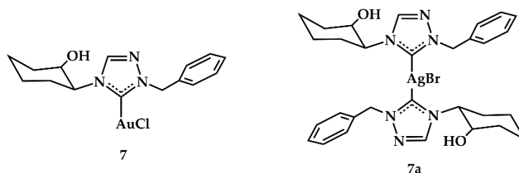
Figure 4. Gold and silver precatalysts of 1,2,4-triazole based NHCs synthesized from Ghosh et al. [17].
