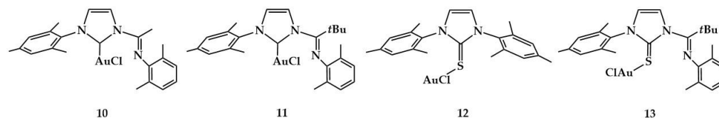
Figure 6. Complexes of Lavoie et al. [19].
