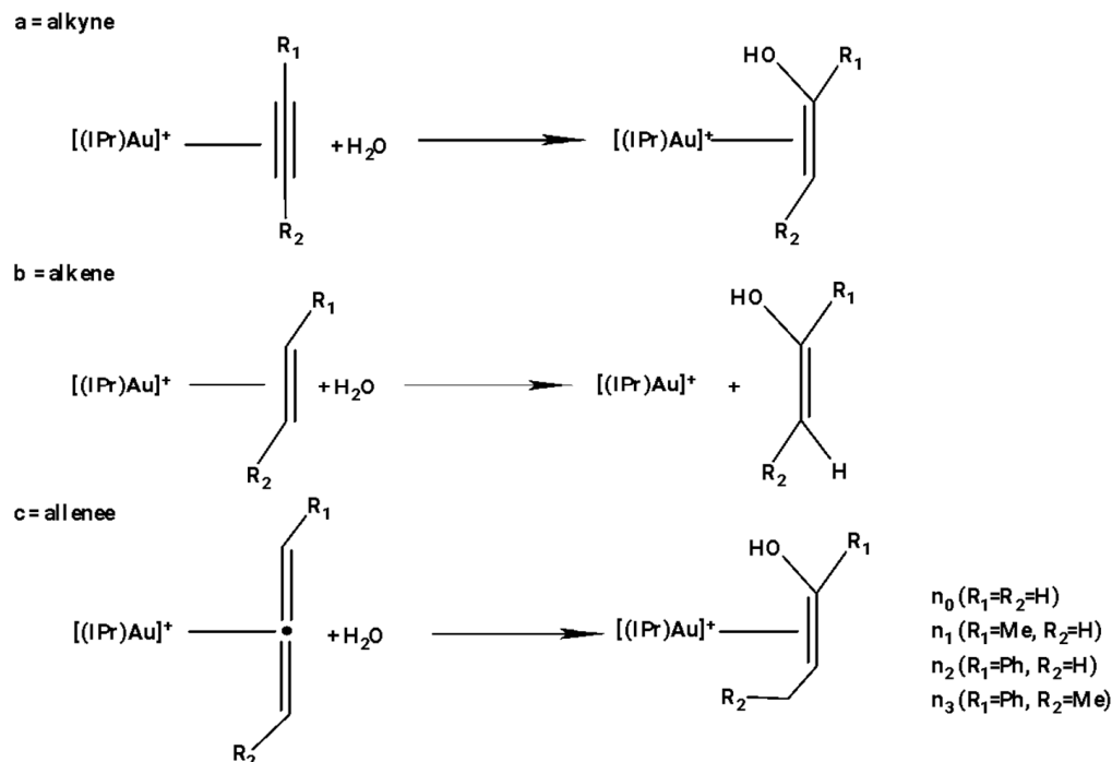
Scheme 14. IPrAu + -catalyzed hydration of alkynes, alkenes, and allenes.
