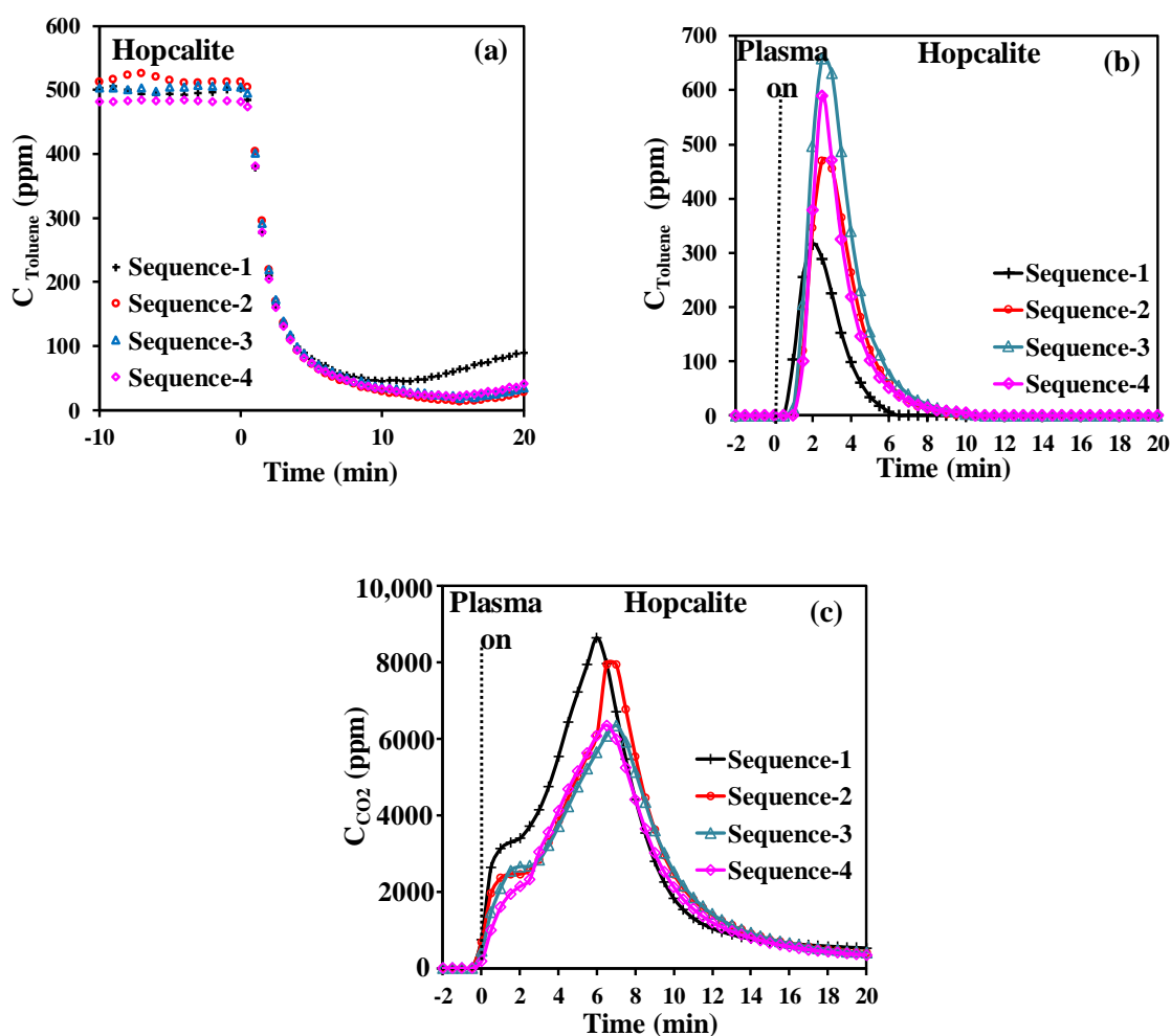
Figure 4. Temporal profiles of toluene during adsorption (a), desorbed toluene during NTP exposure (b), \text{CO}_2 evolution during NTP exposure, (c) over the 4 sequences.
