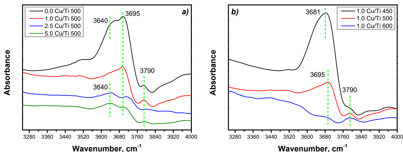
Figure 6. FTIR spectra for (a) X Cu/Ti, and (b) 1.0 Cu/Ti Y in the absorption band of hydroxyl species in the 3200–4000 \text{cm}^{-1} region from 25 up to 400 ^{\circ}\text{C} .
