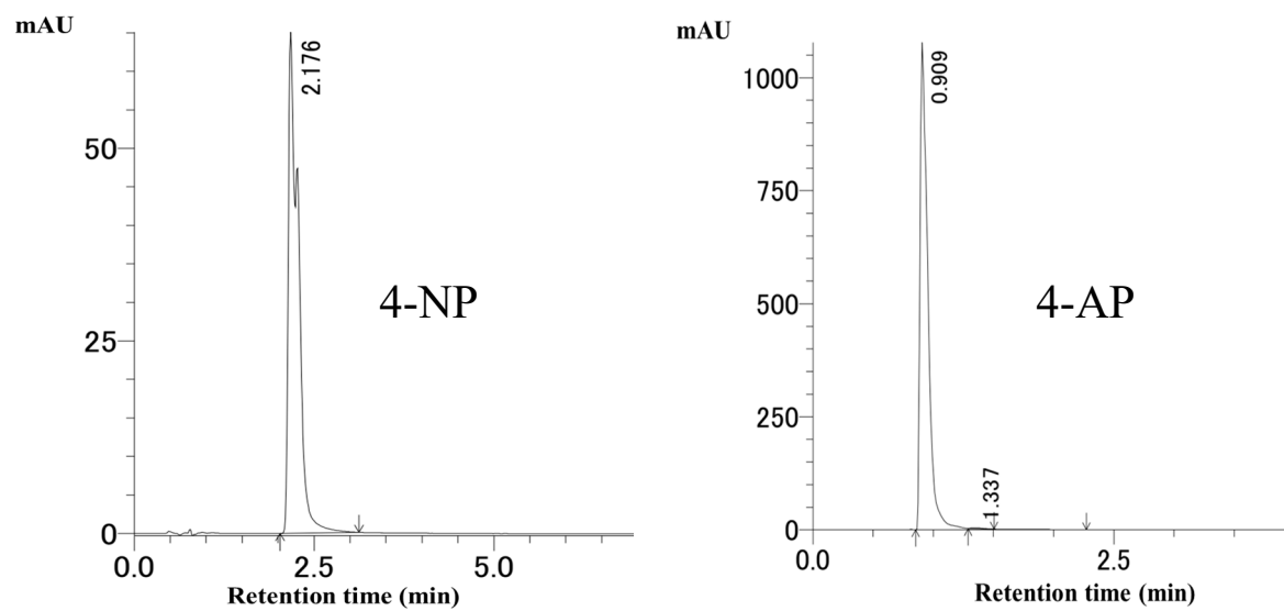
Figure S1: HPLC chromatograph of 4-nitrophenol (4-NP) and 4-aminophenol (4-AP)
