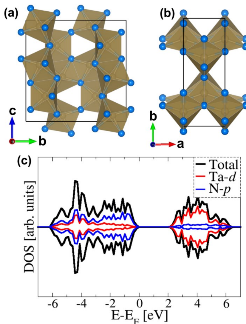
Figure 1. The orthorhombic crystal structure of \text{Ta}_3\text{N}_5 in terms of \text{TaN}_6 octahedra viewed in the (a) c - b and (b) b - a planes. (c) The electronic density of state of \text{Ta}_3\text{N}_5 showing the total and projection on the Ta d states and N p states. (Colour scheme: Ta = pale olive and N = blue.)
