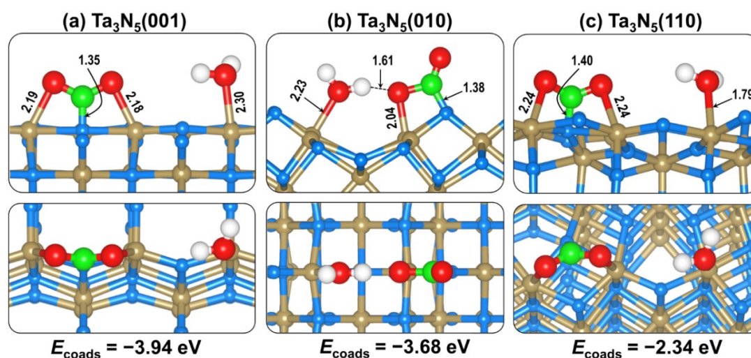
Figure 7. Lowest energy of coadsorption structures of \text{CO}_2 + \text{H}_2\text{O} on (a) (001), (b) (010), and (c) (110) \text{Ta}_3\text{N}_5 surfaces. (Atomic colour scheme: Ta = pale olive, N = blue, C = green, O = red, and H = white.)
