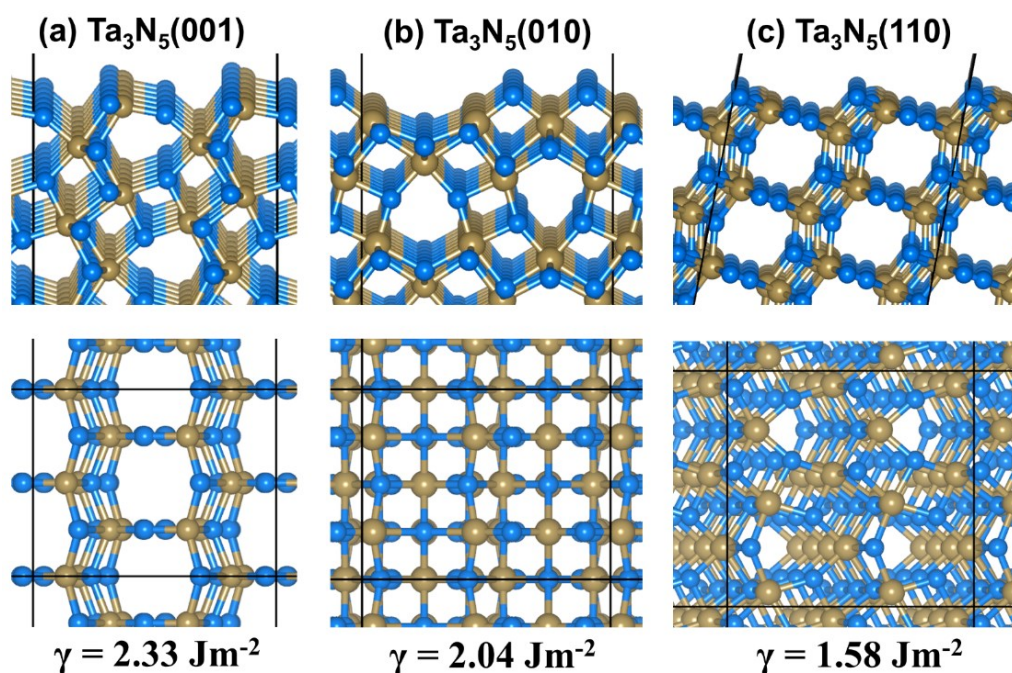
Figure 2. Optimized structures of the (a) {001}–(2 × 1), (b) {010}–(2 × 1), and (c) {110}–(1 × 1) surfaces of \text{Ta}_3\text{N}_5 , in top (top) and side (bottom) views. (Atomic colour scheme: Ta = pale olive and N = blue.)
