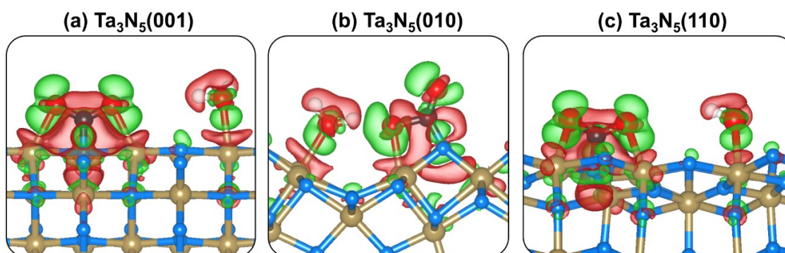
Figure 8. Differential charge density isosurface contours of the \text{CO}_2 + \text{H}_2\text{O} coadsorption on \text{Ta}_3\text{N}_5 (a) (001), (b) (010), and (c) (110) surfaces. The green contours denote electron density increase whereas the red contours denote electron density decrease by 0.02 \text{ e}/\text{\AA}^3 , respectively. (Atomic colour scheme: Ta = pale olive, N = blue, C = green, and O = red.)
