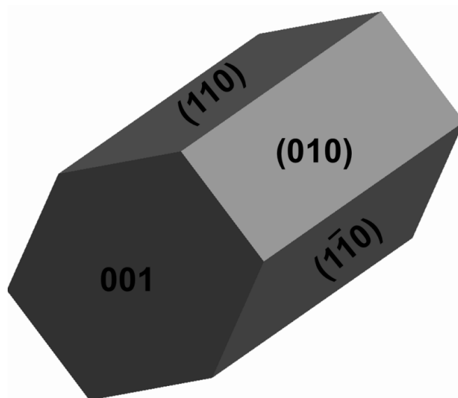
Figure 3. Equilibrium morphology of \text{Ta}_3\text{N}_5 nanocrystal derived from Wulff construction.
