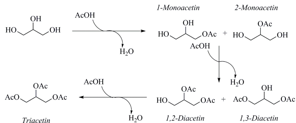
Figure 1. Esterification reaction pathways of glycerol to acetyl derivatives.
