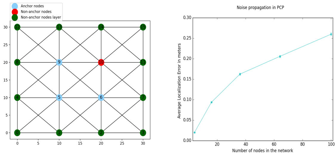
Figure 7. 16-node network example (left). Localization error against number of nodes (right).
