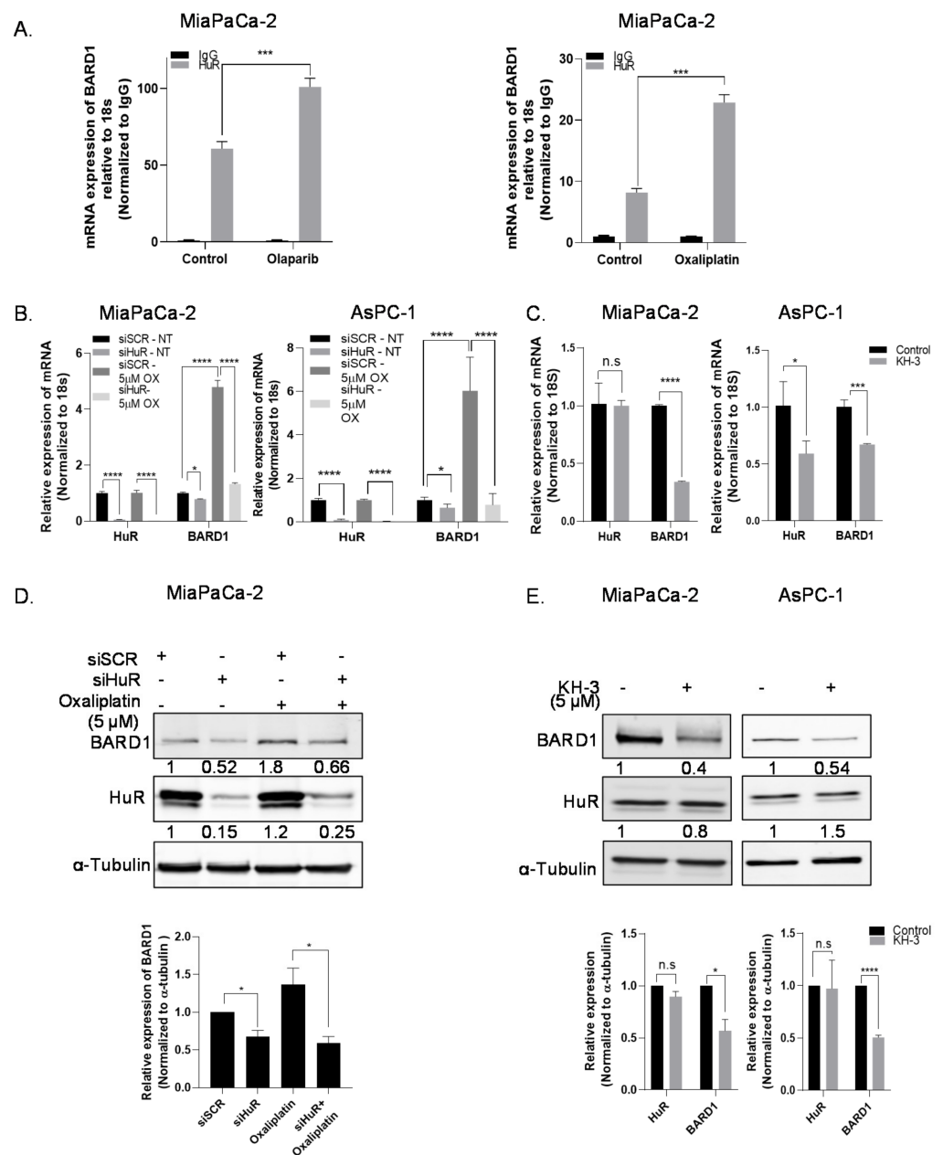
Figure 2. HuR regulates mRNA and protein expression of BARD1. (A) Independent HuR-RNP-IP was performed after treating cells with either olaparib (10 μM) or oxaliplatin (5 μM) and BARD1 mRNA expression was calculated relative to 18 s by RT-qPCR. Mean ± SEM, n = 3 . *** p < 0.001 (Student's t -test). (B) Relative mRNA expression of BARD1 in MiaPaCa-2 and AsPC-1 PDAC cells after treatment of cells with oxaliplatin and siHuR (siHuR#1) transfection. * p < 0.05 , **** p < 0.0001 . (C) Relative mRNA expression of BARD1 in MiaPaCa-2 and AsPC-1 cells treated with KH-3 (5 μM) for 48 h. Mean ± SEM, n = 3 . *** p < 0.001 , * p < 0.05 , n.s., non-significant. (Student's t -test). (D,E) Western blot analysis of the protein expression of BARD1, HuR, and α-tubulin in MiaPaCa-2 cells treated with oxaliplatin (5 μM) and transfected with siHuR (siHuR#1) for 48 h or treated with KH-3 for 72 h. Representative blots and graphs showing relative band intensities is shown. Mean ± SEM from n = 3 , * p < 0.05 , **** p < 0.0001 , n.s., non-significant. (Student's t -test).
