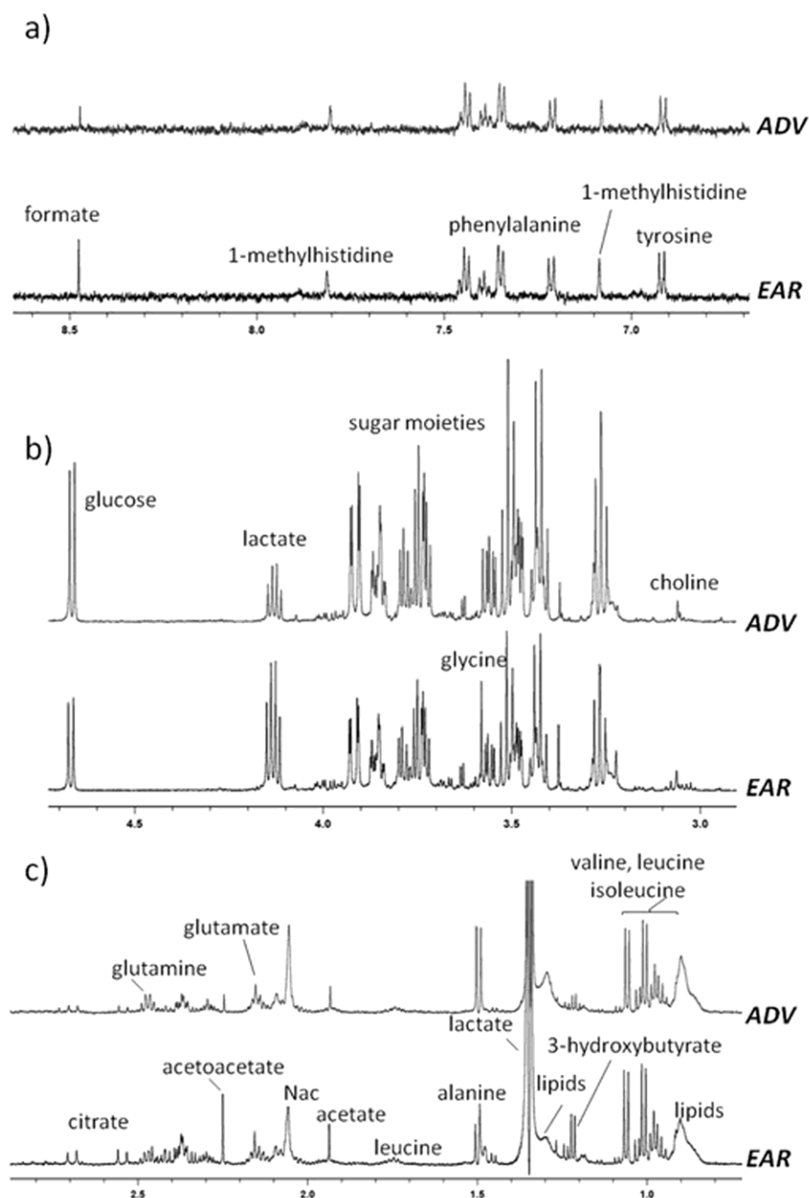
Figure 1. Typical proton Carr–Purcell–Meiboom–Gill nuclear magnetic resonance ( ^1\text{H} CPMG NMR) spectra in the (a) aromatic, (b) sugars and (c) aliphatic regions, with some identified metabolites for the different groups of advanced (ADV) and early (EAR) hepatocellular carcinoma (HCC) patients referred to the specific sample spectra in the figure.
