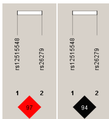
MSH3 (rs12515548 and rs26279)
