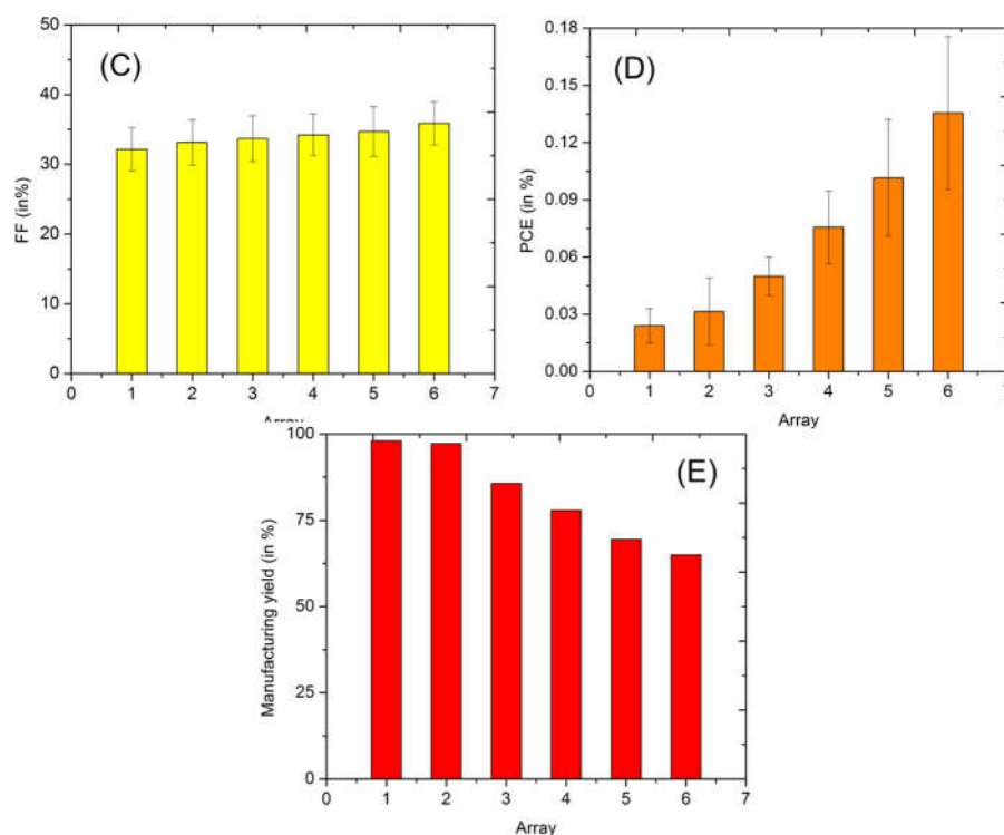
Figure 7. Graphs showing the statistics behind (A–D) the electrical properties and (E) the manufacturing yield of the all inkjet-printed OPV device arrays having 216 devices, with Arrays 1–6 having active areas of 5 mm 2 , 7.5 mm 2 , 10 mm 2 , 12.5 mm 2 , 17.5 mm 2 , and 20 mm 2 , respectively.
