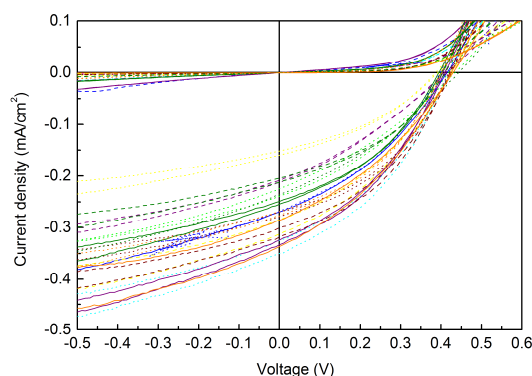
Figure 6. Graph showing the current versus voltage electrical characteristics of the all inkjet-printed OPVs with 17.5 mm 2 as an active area.
