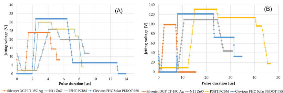
Figure 3. Images exhibiting the suitable jetting waveforms for the different inks implemented for depositing the functional layers of the OPV devices, using (A) DMP-2831 with DMC printheads; and (B) DMP-3000 with SE3 printheads.
