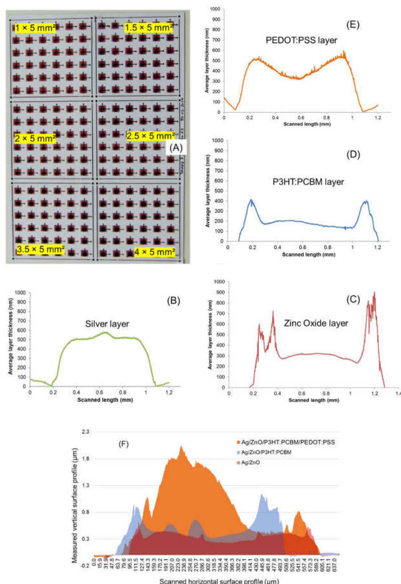
Figure 5. (A) Photograph showing OPV array with all six active areas printed using the DMP-3000 i.e., 5 \text{ mm}^2 , 7.5 \text{ mm}^2 , 10 \text{ mm}^2 , 12.5 \text{ mm}^2 , 17.5 \text{ mm}^2 , and 20 \text{ mm}^2 ; (B–E) average surface profiles of printed layers for Ag bottom electrode deposited using silverjet DGP LT-15C nanoparticle-based ink with 65 \mu\text{m} drop space, two electron transport layers using ZnO (N11) ink with 40 \mu\text{m} drop space, an active layer using P3HT:PCBM ink with 40 \mu\text{m} drop space, and a top electrode layer using PEDOT:PSS CLEVIOS™ F HC Solar ink with 35 \mu\text{m} drop space. In comparison, (F) shows the buildup of the actual OPV stack using the same deposition parameters.
