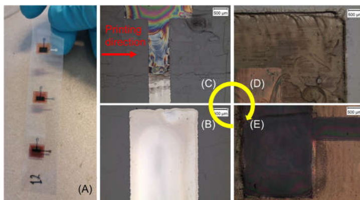
Figure 4. (A) Photo of all inkjet-printed OPVs of different active areas and microscopic images of the printed functional layer corresponding to (B) the bottom Ag cathode electrode, (C) the ZnO ETL layer, (D) the P3HT:PCBM bulk heterojunction or photoactive layer, and (E) the top PEDOT:PSS anode electrode layer, shown exemplarily for 2.5\text{ mm} \times 5\text{ mm} .
