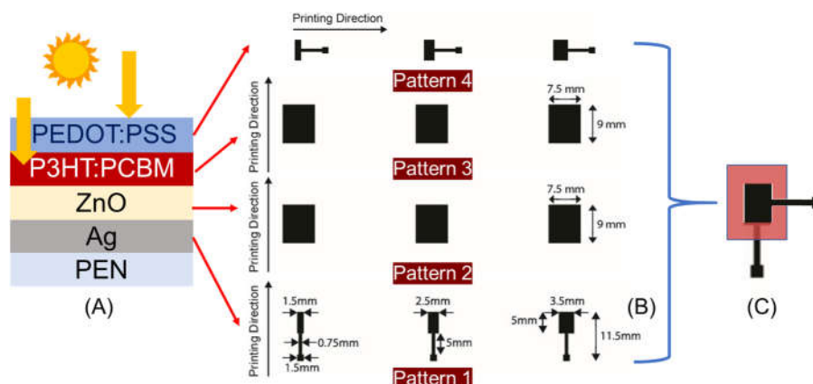
Figure 1. Image showing a (A) conventional OPV device architecture, (B) an overview of the designed digital patterns 1–4 with bottom Ag and top PEDOT:PSS electrode layers with different sizes and constant size of the electron transport layer (ETL) and bulk heterojunction (BHJ) layers, and (C) a top view of the intended OPV device.
