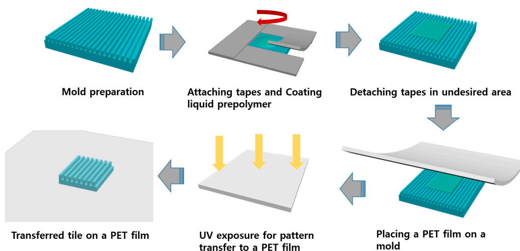
Figure S1. Experimental procedure using tape to define the tile shapes.
