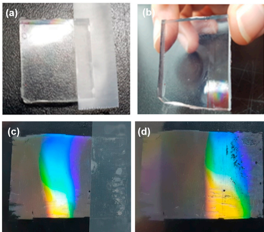
Figure S2. (a) A PDMS mold, with tape to remove the outside of the boundary. (b) The prepolymer, clearly removed by detaching the tape. (c) The PUA mold, adhered using tape. (d) The sticky residues remaining on the PUA mold.
