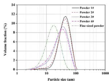
Figure 6. Particle size distribution of powder [44].
