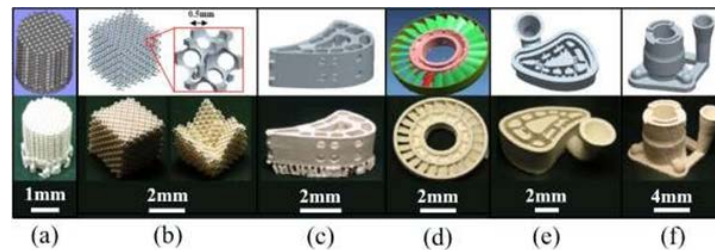
Figure 11. Advanced ceramic parts manufactured with SLM [91]: (a) porous bioceramic scaffolding; (b) photonic crystals; (c) hollow turbine blade; (d) impeller; (e–f) investment casting moulds.
