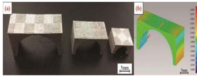
Figure 10. 316L Bridge model made by SLM: (a) A sample of a bridge-shaped structure; (b) the deformation diagram [76].
