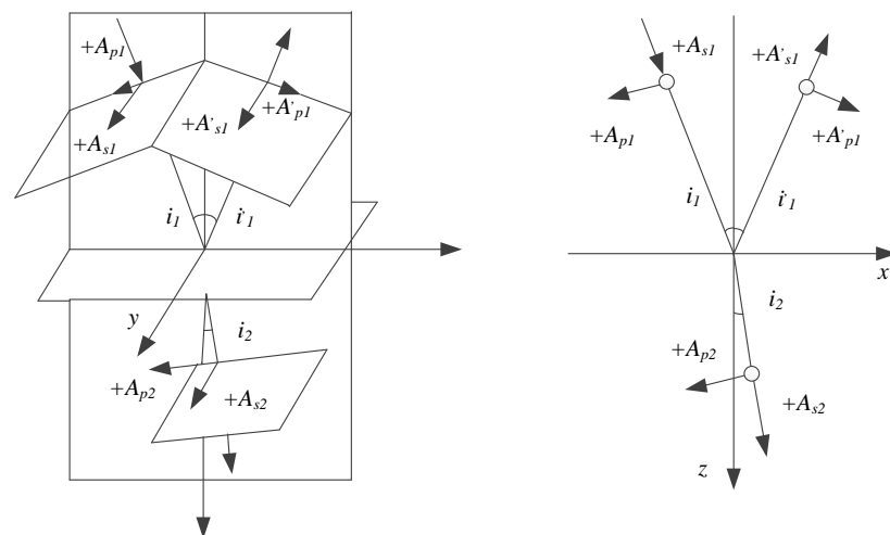
Figure 5. Reflection and its schematic diagram.
