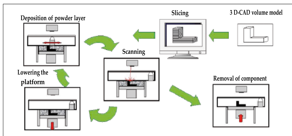
Figure 1. Principle of the SLM process [7].
