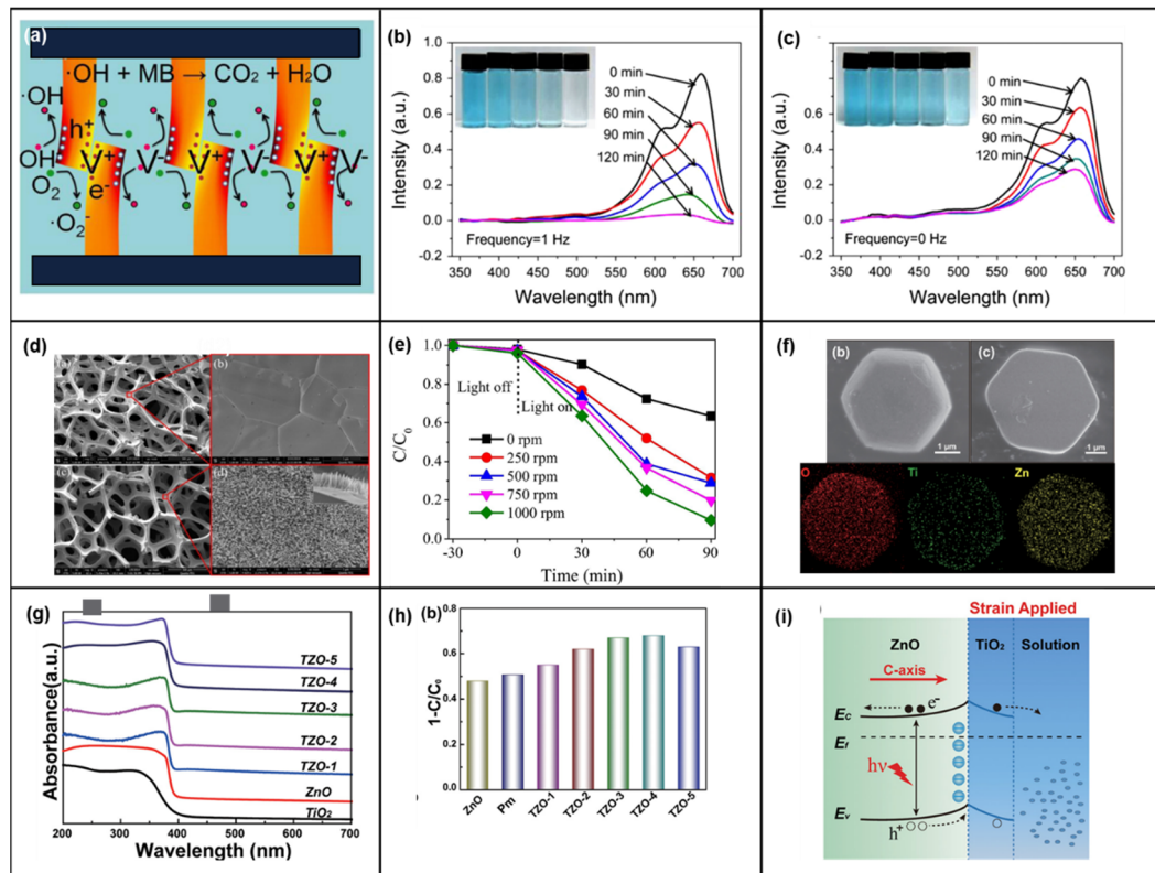
Figure 4. Schematic diagram of piezoelectric enhanced photocatalytic ZnO NW device and UV-Vis absorption spectroscopy. (a) Working mechanism of piezoelectric photocatalytic activity of ZnO nanowires. (b,c) UV-Vis absorption spectra after piezoelectric-assisted and non-piezoelectric-assisted photodegradation under different ultraviolet illumination times, respectively. Reproduced with permission from [54]. Copyright (2015) Nano Energy . SEM image of ZnO nanorod arrays/3D Ni foam and photocatalytic degradation of RhB on ZnO nanorod arrays/Ni foam. (d) On the left are Ni foam and ZnO nanorod arrays/Ni foam. The inset is the side-view SEM image. (e) Photocatalytic degradation yield of RhB on ZnO nanorod arrays/Ni foam at different stirring rates under UV light irradiation. Reproduced with permission from [122]. Copyright (2017) Materials Today . Structure, characteristics, and mechanism of the ZnO/TiO 2 hybrid photocatalysts. (f) SEM images of a single ZnO/TiO 2 hybrid sample and the corresponding mapping results. (g) Diffused reflectance UV spectra of the as-synthesized samples collected in the absorbance mode. (h) Degradation efficiency of MO in the presence of corresponding samples for 30 min. (i) The working mechanism of ZnO/TiO 2 hybrid photocatalysts. Reproduced with permission from [123]. Copyright (2016) American Chemical Society Nano .
