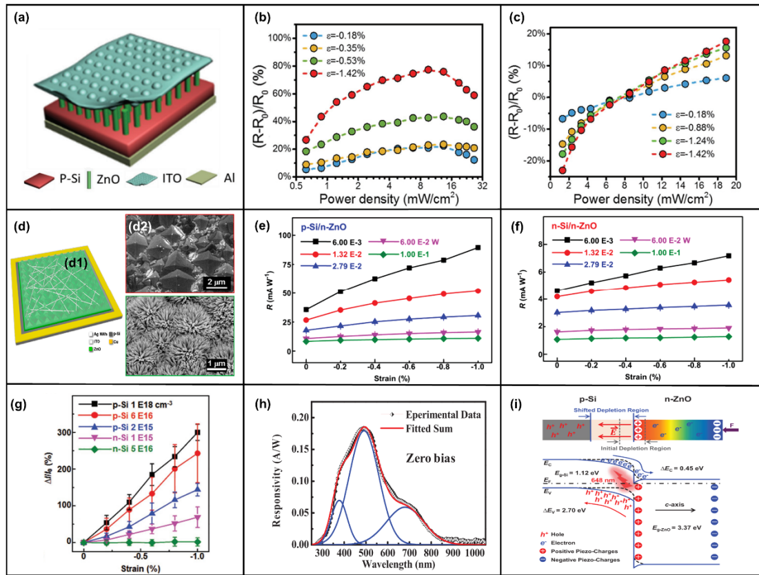
Figure 5. Device structure and characterization of Si/ZnO photodetector. (a) Device structure of p-Si/n-ZnO NWs photodetectors. (b,c) Relative changes of photoresponsivity of the device under different strains and illumination of 442 nm and 1060 nm at -2 V, respectively. Reproduced with permission from [159]. Copyright (2017) Advanced Materials . (d) Schematic structure of a p-Si/n-ZnO NW hybridized photodetector etched by KOH. Reproduced with permission from [160]. Copyright (2014) American Chemistry Society Nano . (e,f) The photoresponsivity as a function of compressive strain under different optical powers for the p-Si/n-ZnO NWs (at -1 V) and the n-Si/n-ZnO NWs (at 1 V) heterojunction photodetectors. Reproduced with permission from [161]. Copyright (2018) Advanced Functional Materials . (g) The average relative changes in photocurrent as a function of external compressive strain under 1.90 \times 10^{-3} W laser power for the Si/ZnO heterojunction photodetectors with different doping types and concentrations of Si. Reproduced with permission from [162]. Copyright (2020) Advanced Functional Materials . (h) Deconvoluted spectral responsivity at zero bias ( 0 V). Reproduced with permission from [164]. Copyright (2017) Journal of Physics D-Applied Physics . (i) Schematic energy band diagrams of the p-Si/n-ZnO NWs without (dashed black line) and with (solid blue line) external compressive strain to 648 nm laser illumination. Reproduced with permission from [162]. Copyright (2020) Advanced Functional Materials .
