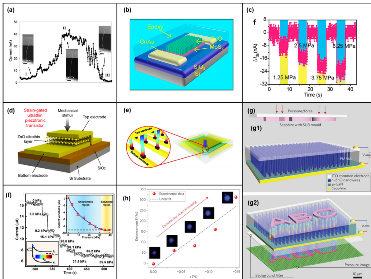
Figure 3. (a) The current value of the voltage-controlled NW transistor under the action of different forces. Reproduced with permission from [42]. Copyright (2006) Nano Letters . Structure and piezoelectric characteristics of pressure-gated field-effect transistors based on 2D MoS 2 . (b) Device structure. (c) Change of drain current at different pressures. Reproduced with permission from [115]. Copyright (2016) American Chemical Society Nano . (d) Schematic diagram of an ultra-thin transistor with a channel length of 2 nm. Reproduced with permission from [6]. Copyright (2018) American Chemical Society Nano . The structure diagram of the ZnO NW-based tactile sensing array is the current characteristic diagram. (e) A 3D piezo-gated transistor array schematic diagram and the individual device block diagram (enlarged schematic). (f) The current of a single tactile probe at different pressures corresponds to the current. Reproduced with permission from [119]. Copyright (2013) Science . Piezoelectric nanowire LED array structure diagram with pressure response of enhancement factor. (g) (g1) and (g2) are sensor arrays before and after strain is applied, respectively. (h) Pressure-response diagram of the LED enhancement factor and the corresponding emitted light image. Reproduced with permission from [37]. Copyright (2013) Nature Photonics .
