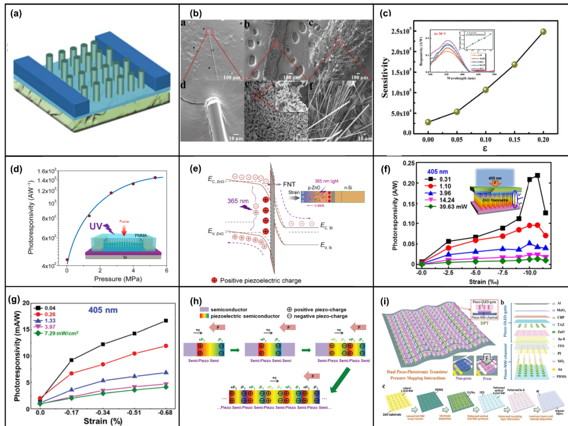
Figure 7. Device structure and characterization of the M-S-M and multilayer structure formed by ZnO NWs. (a) Schematic illustration of Ag-ZnO-Ag photodetector. Reproduced with permission from [197]. Copyright (2018) Royal Society of Chemistry Advances . (b) Field-emission scanning electron microscopy images of as-synthesized ZnO microarchitectures: ZnO microwire, ZnO coral-like microstrip, and ZnO fibril-like clustered microwire. Reproduced with permission from [199]. Copyright (2018) Small . (c) Sensitivity as a function of the tensile strain. Inset: responsivity spectra of the photodetector with different tensile strains under 30 V. Reproduced with permission from [200]. Copyright (2019) Advanced Materials Interfaces . (d) Photoresponsivity of ZnO photodetector as a function of applied pressure at M-S contact. Inset: device structure. Reproduced with permission from [203]. Copyright (2021) Nano Energy . (e) Schematic band diagrams of the piezo-phototronic effect in p-ZnO/Al 2 O 3 /n-Si junction. Reproduced with permission from [212]. Copyright (2021) Nano Energy . (f) The photoresponsivity at a bias of -2 V as a function of the compressive strain under different illuminant powers for 405 nm laser illuminations. Inset: 3D schematic device of the n-Si/n-ZnO/p-PEDOT: PSS tri-layer structure. Reproduced with permission from [30]. Copyright (2018) Nano Energy . (g) Photoresponsivity of the p-Si/i-ZnO/n-ZnO photodiode as a function of externally applied compressive strain. (h) Perspectives on piezo-charge engineering at multi-layer piezo-semi optoelectronic device interfaces. Reproduced with permission from [216]. Copyright (2020) Journal of Materials Chemistry C . (i) Schematic illustration and fabrication processes of the designed dual piezo-phototronic transistor pressure-mapping interaction system with the dual piezo-phototronic transistor array. Reproduced with permission from [217]. Copyright (2020) Advanced Functional Materials .
