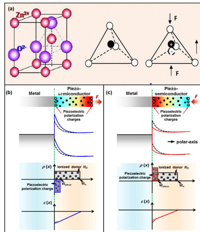
Figure 1. (a) Atomic model of the wurtzite-structured ZnO. Reproduced with permission from [40]. Copyright (2012) Advanced Materials . The energy band diagram, spatial charge distribution, and electric field schematics where (b) tensile strain is applied and (c) compressive strain is applied. Reproduced with permission from [61]. Copyright (2013) Nano Today .
