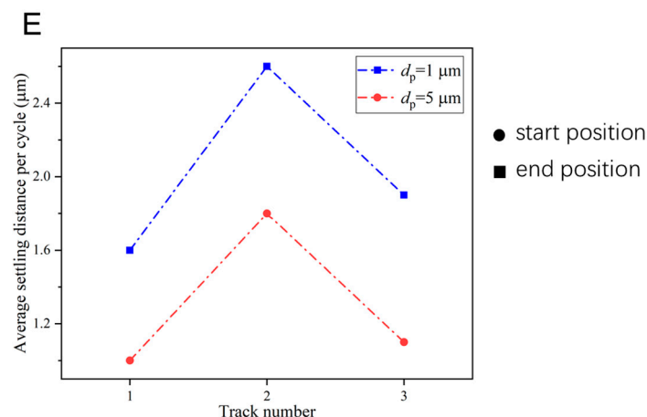
Figure 7. Comparison of settling rates of particles of different sizes in the alveolar chip of the 21st generation. (A) Tracked positions of 1 \mu\text{m} particles at end of each breathing cycle; (B) tracked positions of 5 \mu\text{m} particles at end of each breathing cycle; (C) 1 \mu\text{m} particles settling displacements along the gravitational direction; (D) 5 \mu\text{m} particles settling displacements along the gravitational direction; (E) average settling distance per breathing cycle of different size particles.
