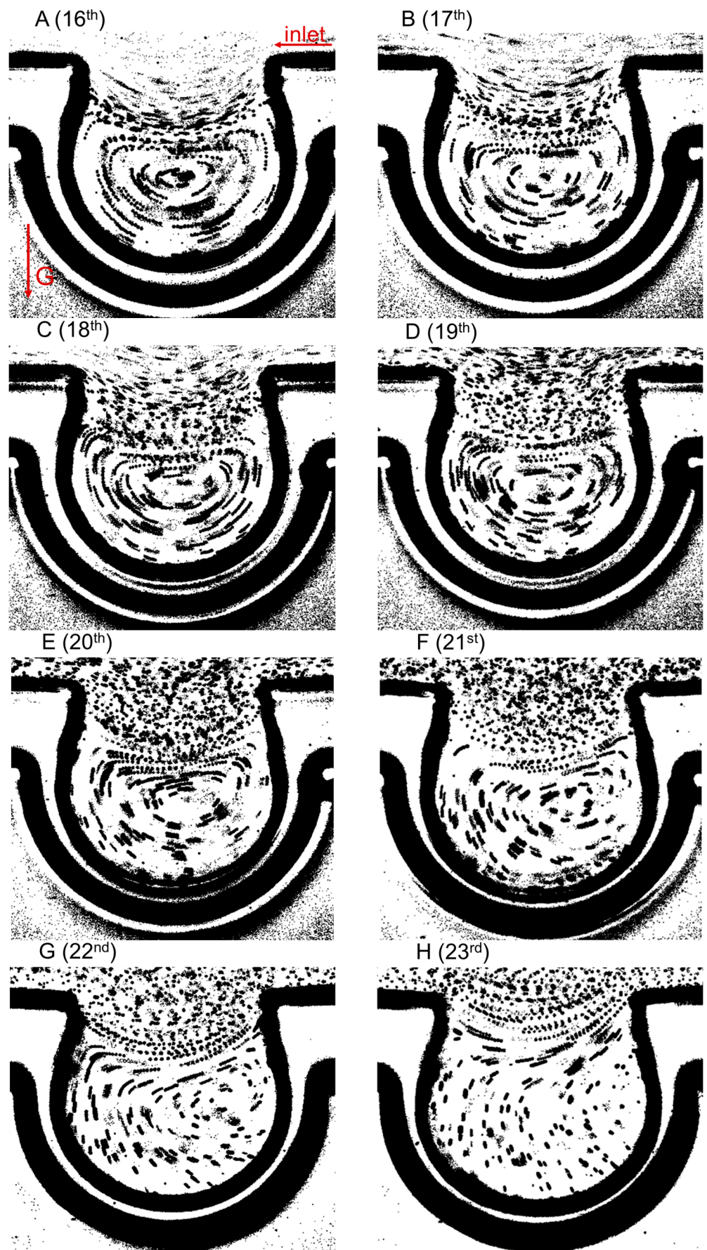
Figure 4. Visualized flow fields at t = T/4 (peak of inhalation) in the vertically placed chip. (A–H) are the measurements for the alveoli at the 16th to 23rd acinar generations, respectively.
