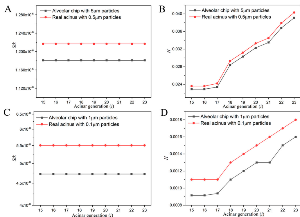
Figure 2. Comparison of dimensionless particle number at different acinar generations. (A) Stokes number of 5 \mu\text{m} silver particle. (B) Gravity number of 5 \mu\text{m} silver particle. (C) Stokes number of 1 \mu\text{m} silver particle. (D) Gravity number of 1 \mu\text{m} silver particle.
