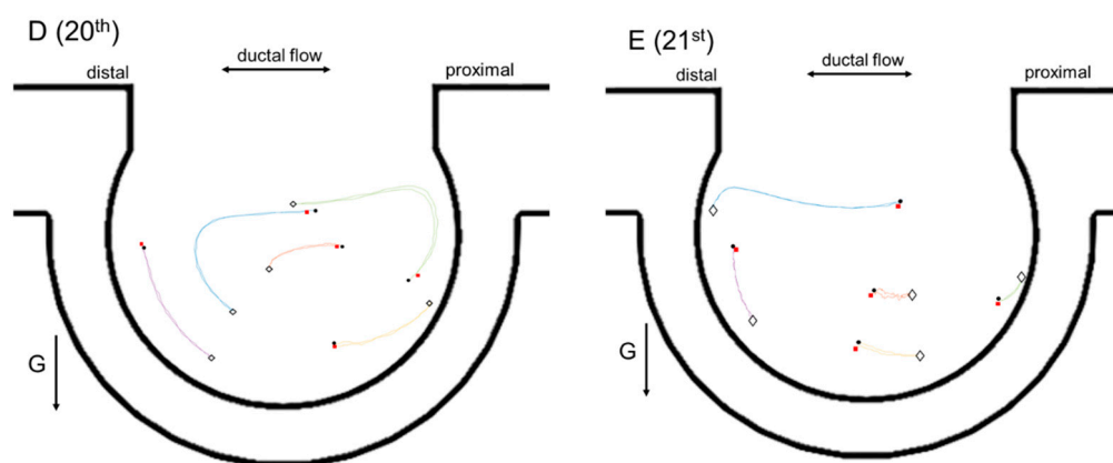
Figure 5. Particle trajectories at different acinar generations over one breathing cycle. (A–E) are particle tracks inside the alveoli at the 17th to 21st acinar generations, respectively.
