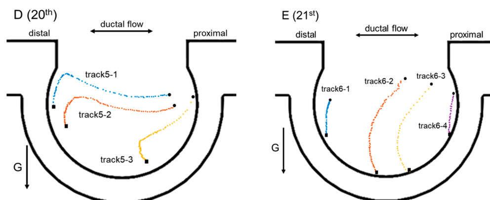
Figure 6. Particle positions at end of each cycle at different acinar generations. (A–E) are particle tracks inside the alveoli at the 17th to 21st acinar generations, respectively. Colors have no significance other than to differentiate between individual particles.
