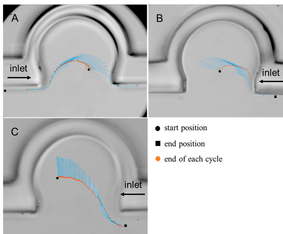
Figure 3. Trajectories of particles in horizontally placed chip. (A) A 5\ \mu\text{m} particle over 24\ T at the 21st generation. (B) A 1\ \mu\text{m} particle over 34\ T at the 21st generation. (C) A 1\ \mu\text{m} particle over 101\ T at the 23rd generation.
