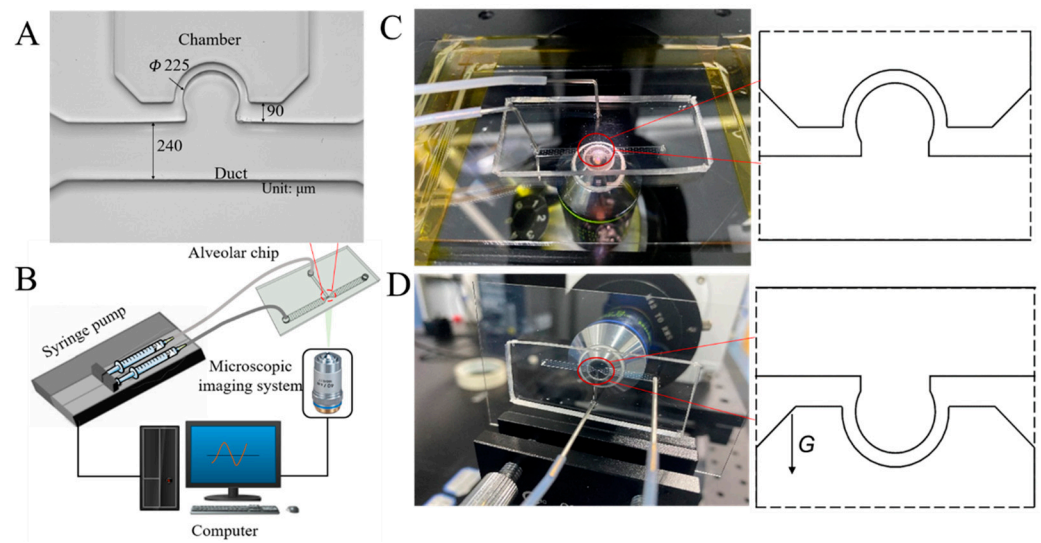
Figure 1. The alveolus chip and experimental system. (A) Photograph of the alveolar chip. (B) Schematic diagram of experimental device. (C) Alveolar chip placed horizontally. (D) Alveolar chip placed vertically.
