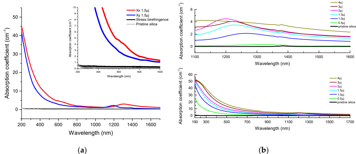
Figure 4. (a) Comparison of absorption coefficient k_{\text{abs}}(\lambda) spectra for different waveplates together with pristine silica. Black line is for the stress-engineered waveplate (a half waveplate at 450 nm) whereas red and blue lines are for nanogratings-based waveplates written in Xx and Xy configurations. (b) Absorption coefficient k_{\text{abs}}(\lambda) spectra of nanogratings-based waveplates for different pulse energies. Note that each waveplate was annealed for 2 hours at 600 °C prior to measurements.
