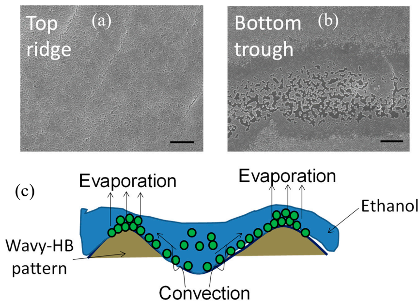
Figure S1. SEM images of deposited nanoparticles (NPs) on (a) top ridge and (b) bottom trough after the deposition process. (c) Illustrative image of the NP convection induced by ethanol evaporation if exposed directly to air. More particles are thus deposited on the top ridge and less particles on bottom trough. Scale bar: 2 \mu\text{m} .
