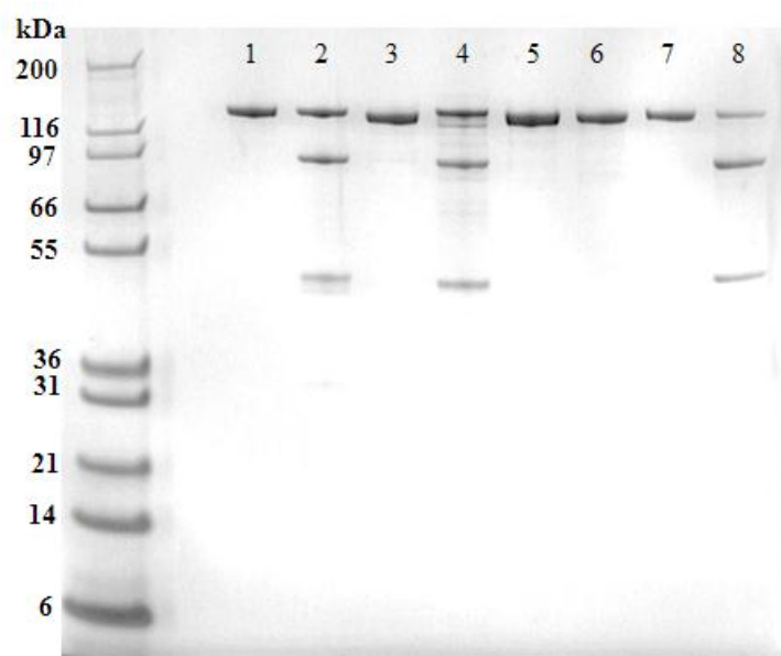
Figure 1. SDS-PAGE gel of approximately 1 µg of purified, recombinant ciBoNT/B1 HP, ciBoNT/C1 HP, ciBoNT/E1 HP, and ciBoNT/F1 HP. Left lane-Mark 12 molecular weight marker, lane 1-ciBoNT/B1 HP, lane 2-BoNT/B1 toxin, lane 3-ciBoNT/C1 HP, lane 4-BoNT/C1 toxin, lane 5-ciBoNT/E1-6xHis HP, lane 6-BoNT/E3 toxin, lane 7-ciBoNT/F1 HP, lane 8-BoNT/F1 toxin.
