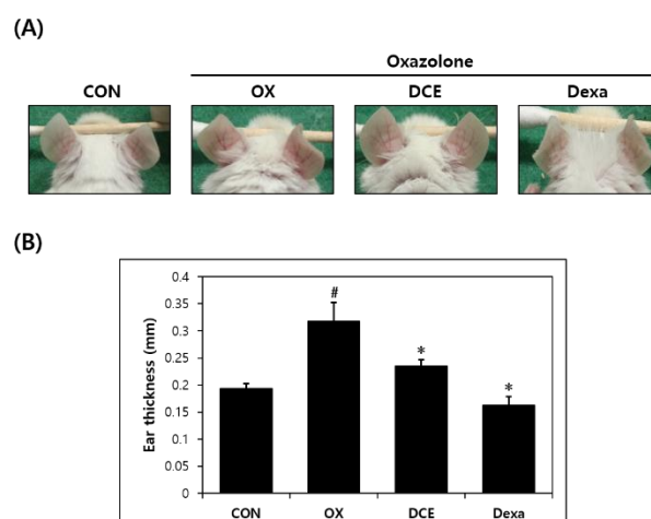
Figure 1. Effect D. costaricensis EtOH extract (DCE) on OX-induced AD-like lesions in the BALB/c mouse model. (A) Clinical features of AD-like symptoms. (B) Ear thickness. CON group: vehicle controls, OX group: oxazolone-treated controls, DCE group: oxazolone plus 1% DCE-treated, and Dexa group: oxazolone plus 0.1% dexamethasone-treated. Data values are presented as means \pm SEMs. # p < 0.05 vs. the CON group, * p < 0.05 vs. the OX group.
