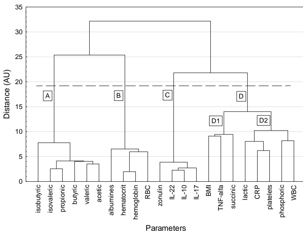
Figure 1. A dendrogram of similarity between studied parameters (method of grouping: Ward agglomeration; function of the distance: Euclidean distance; the dashed horizontal line indicates that grouping was stopped according to the Mojena's rate). BMI: body mass index; CRP: C-reactive protein; RBC: red blood cells; WBC: white blood cells.
