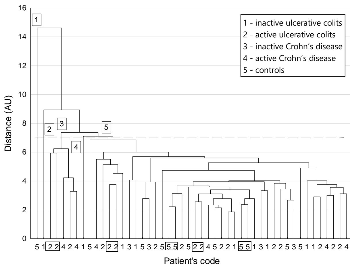
Figure 2. A dendrogram of similarity among study participants (method of grouping: average linkage procedure; function of the distance: Euclidean distance; the dashed horizontal line indicates that grouping was stopped according to the Mojen's rate); patients were labeled according to the classification code; the determined clusters of patients were labeled with numbers: 1–5; rectangles encompass patients belonging to two-element clusters.
