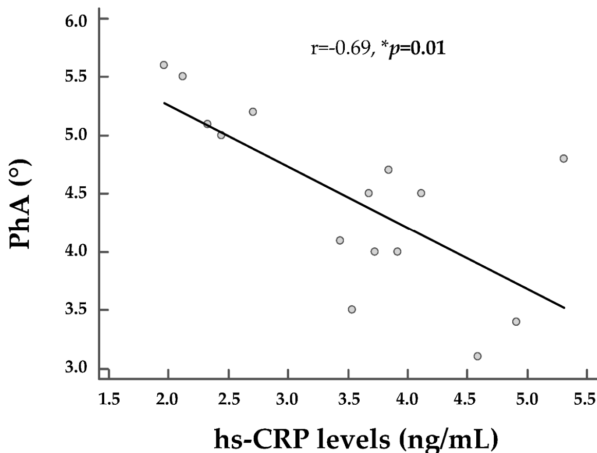
Figure 3. The correlation between PhA and hs-CRP levels, after adjustment for gender, BMI, and waist circumference in PWS adults. PhA showed also a negative association with hs-CRP levels ( r = -0.71 , p = 0.003 ), and as shown in the figure, this negative association remained also after adjustment for covariates ( p = 0.01 ). PhA, phase angle; hs-CRP, high-sensitivity C-reactive protein. *A p -value < 0.05 means a significant difference
