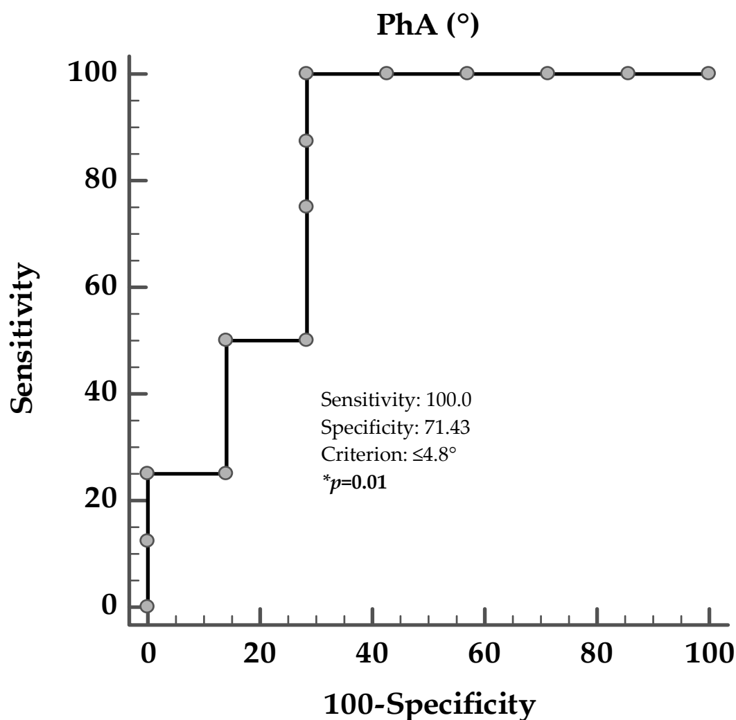
Figure 4. ROC for value of PhA predictive of the highest hs-CRP levels above the median value (3.68 ng/mL). At the ROC analysis, the threshold value of PhA predicting the highest hs-CRP levels (above the median value 3.68 ng/mL) was found at \text{PhA} \leq 4.8^\circ ( p = 0.01 ; AUC, 0.82; standard error, 0.12; 95% CI, 0.58 to 1.00). PhA, phase angle; hs-CRP, high-sensitivity C-reactive protein. *A p-value in bold type denotes a significant difference ( p < 0.05 ).
