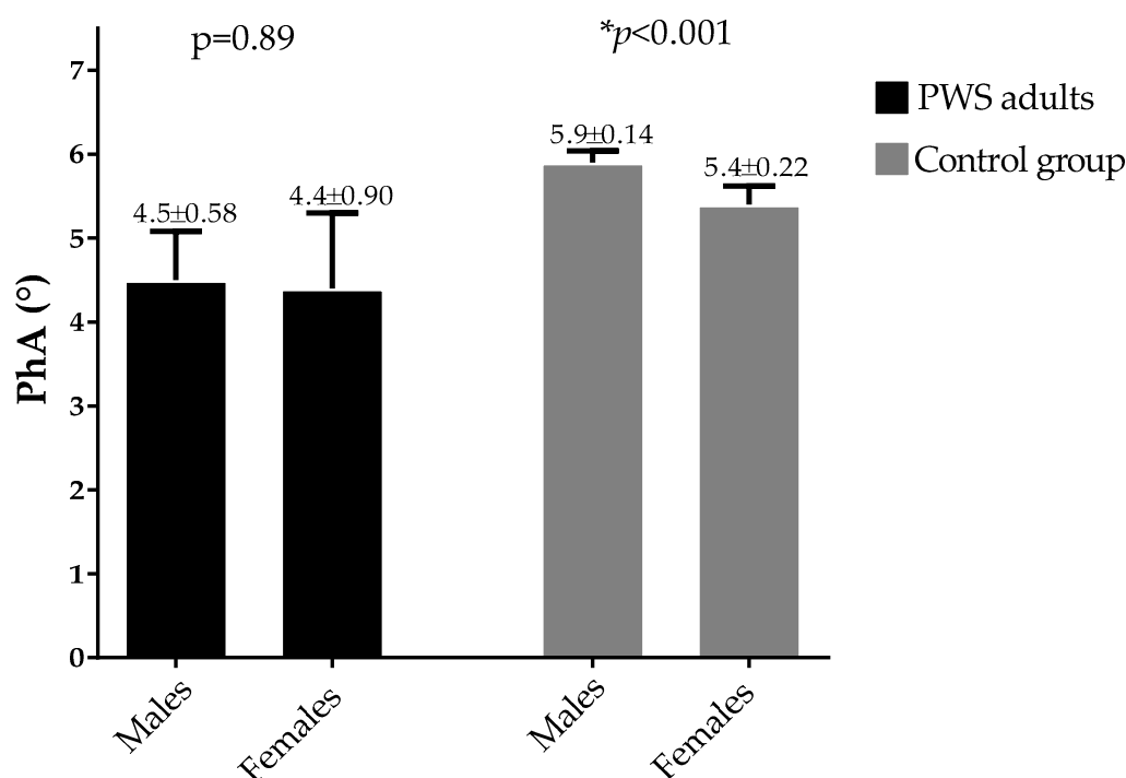
Figure 1. Difference in PhA in PWS adults and control group, according to gender. A clear gender difference in PhA was evident only in the control group, with higher PhA in males compared with females ( p < 0.001 ). PWS, Prader–Willi syndrome; PhA, phase angle. *A p -value < 0.05 means a significant difference.
