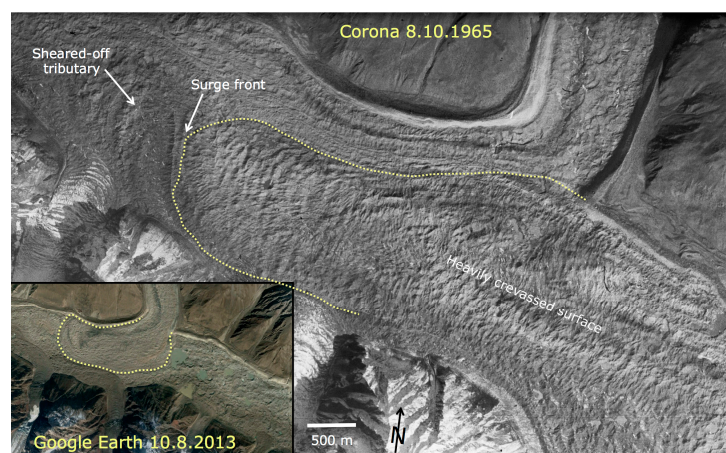
Figure 9. Annotated Corona image from 1965 showing details of the previous surge. For comparison a screenshot of the same region in 2013 from Google Earth is shown in the inset.
