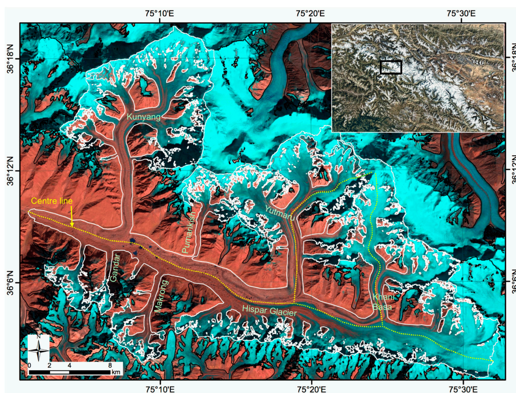
Figure 1. The location of the Hispar Glacier in the Karakoram is indicated on the inset (screen shot from Google Earth) with a black square. The annotated main image depicts the outlines of Hispar Glacier and its tributaries in white and of other glaciers in black. The dotted yellow lines denote centre lines used for extraction of flow velocities (here in 200 m equidistance). Glaciers mentioned in the text are named. The main image is a false colour composite (bands 6, 5, 4 as RGB) from Landsat 8 OLI acquired on 9 October 2013.
