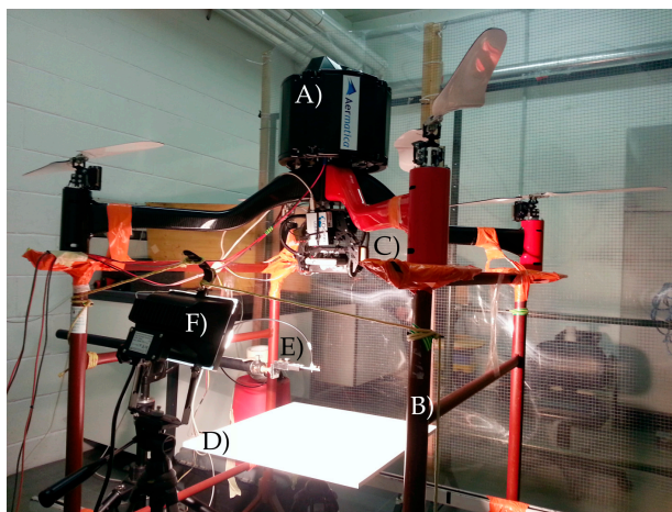
Figure 6. Test-bed used during laboratory tests to simulate in-flight conditions. The HyUAS (A) is attached on a support (B) that permits the vehicle to lift-off keeping the payload; (C) centered in the test-bed. In particular, the figure shows the specific setup used for the radiometric characterization: the halogen light source; (F) illuminates the Spectralon (R) panel; (D) used for cross-calibrating the HyUAS with the reference (calibrated) FieldSpec HH spectrometer (E).
