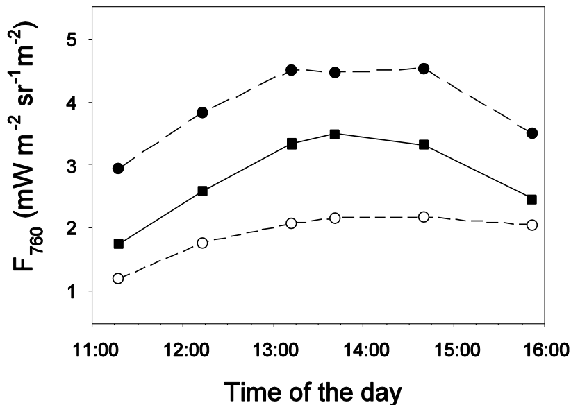
Figure S1: Diurnal changes of canopy sun-induced chlorophyll fluorescence measured at 760 nm ( F_{760} ) in sugar beet. Each data point represents the median F_{760} at each measuring time for: all vegetation pixels including sunlit and shaded surfaces (closed squares), vegetation pixels classified as class 1 (closed circles), vegetation pixels classified as class 2 (open circles). The data was collected over a single day.
