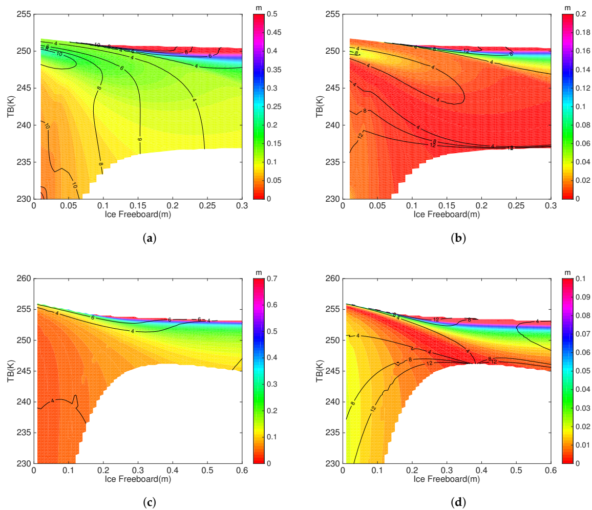
Figure 7. Sensitivity study of retrieved parameters to freeboard measurements. Results for the synergy between TB and FB_{ice} are shown. (a,b) show the sensitivity of the retrieved h_i and h_s to FB_{ice} for FYI, respectively. (c,d) show the results for MYI. The filled color contour is the absolute uncertainty of h_i or h_s (in meters), and the labeled lines are the relative uncertainty (units: %). The uncertainty for FB_{ice} is quantified in terms of standard deviations according to Table 3. The absolute uncertainty in h_i or h_s (denoted \epsilon_{absolute} ) is the quantitative difference in h_i or h_s as caused by perturbation to FB_{ice} or TB by 1 standard deviation. The relative uncertainty of y is computed as: \epsilon_{relative}|_y = \frac{\epsilon_{absolute}|_y}{y} \times 100\% , where y is the corresponding value of h_i or h_s .
