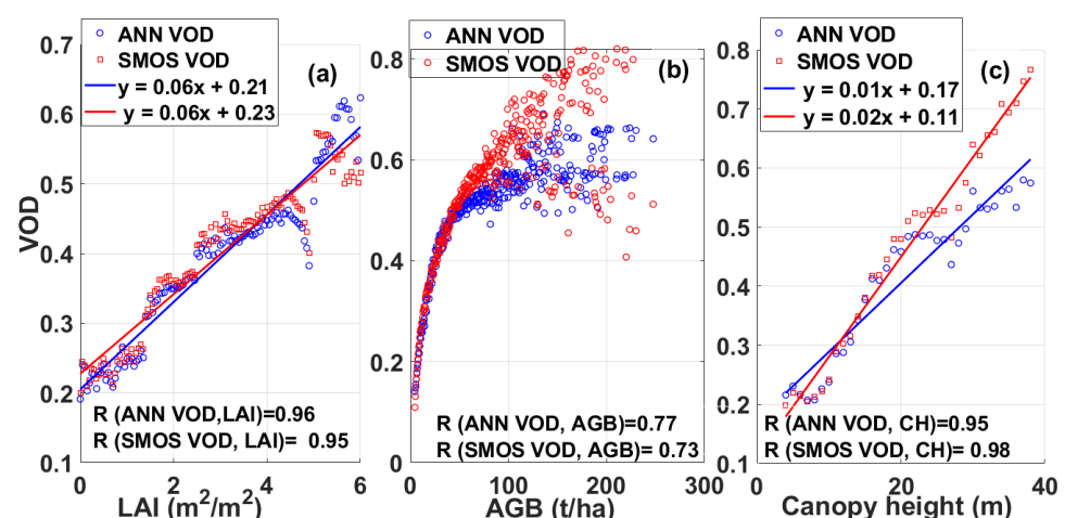
Figure 13. Comparison of VOD estimates from SMOS and ANN against (a) LAI, (b) AGB, and (c) canopy height.
