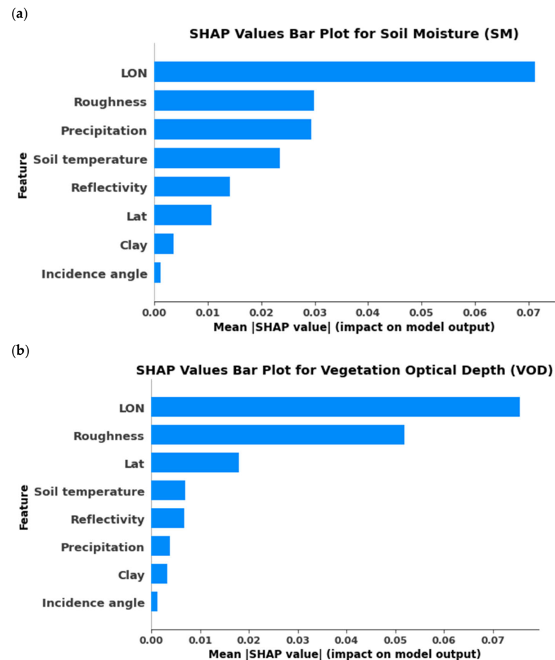
Figure 17. Mean absolute SHAP values of the input features for (a) SM prediction and (b) VOD prediction.
