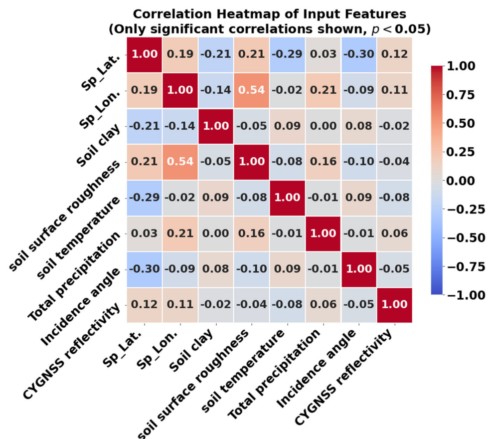
Figure 3. Interdependence of input features based on Pearson correlation.
