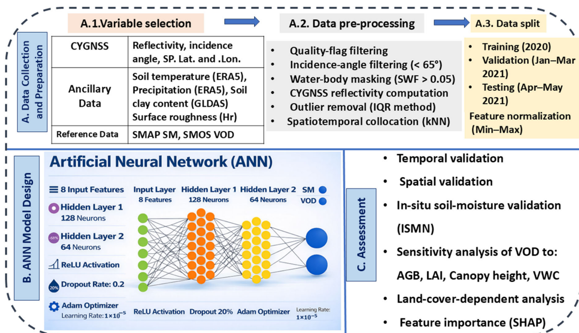
Figure 2. Overall workflow of the proposed ANN-based framework for soil moisture and vegetation optical depth retrieval from CYGNSS data. The main processing steps are highlighted in blue, while other colors are used to distinguish sub-steps within data collection and preprocessing, as well as the layers of the artificial neural network. The colors are used for illustrative purposes only and do not represent quantitative values.
