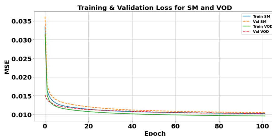
Figure 4. Learning curves of the ANN model for soil moisture and vegetation optical depth estimation.
