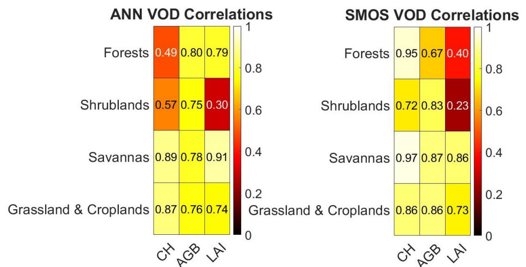
Figure 16. Comparison of ANN-derived VOD and SMOS VOD correlations with vegetation indicators across vegetation classes.
