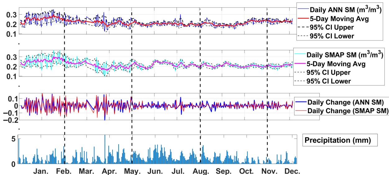
Figure 7. Time-series comparison of ANN-predicted soil moisture (SM; top row) with SMAP observations (second row) for 2021. The panels display daily values, 5-day moving averages with 95% confidence intervals, and day-to-day changes (third row). Total precipitation is shown in the fourth row. Dashed lines are used to distinguish the seasons (spring: March–May; summer: June–August; fall: September–November; winter: December–February).
