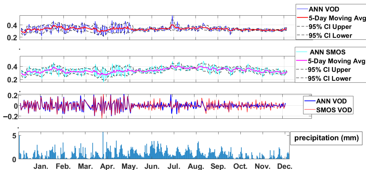
Figure 8. Time-series comparison of ANN-predicted VOD (top row) with SMOS VOD (second row) in 2021. The panels show daily values, 5-day moving averages with 95% confidence intervals, and day-to-day changes (third row). Total precipitation is shown in the fourth row.
