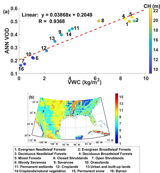
Figure 14. (a) Relationship between ANN-derived VOD and VWC across land cover types. (b) Yearly land cover classification provided by MODIS (MCD12C1) [37] across the CONUS.
