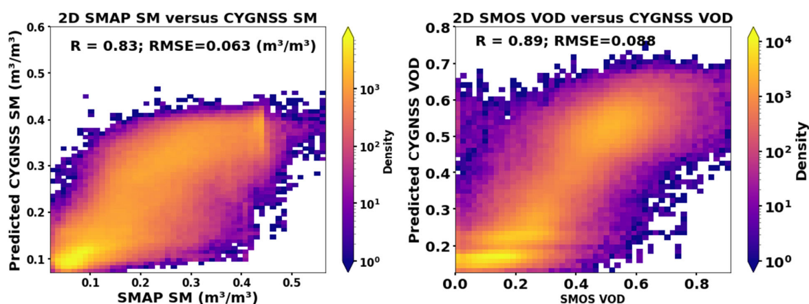
Figure 5. Predicted CYGNSS SM and VOD versus SMAP SM and SMOS VOD on the test dataset.
