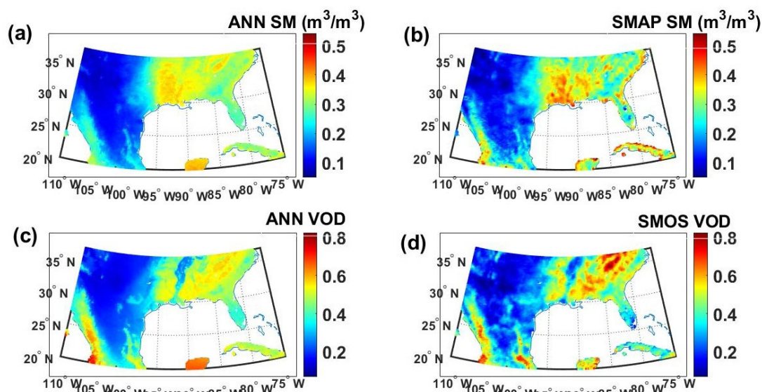
Figure 11. Maps of the mean values of (a) predicted SM and (b) SMAP SM, as well as the (c) predicted VOD and (d) SMOS VOD for the first six months of 2021 (January–June).
