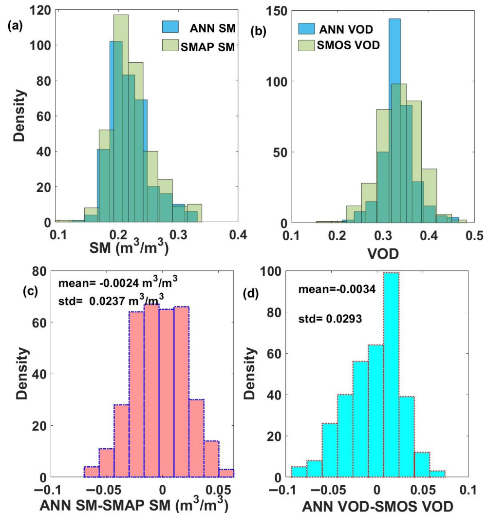
Figure 9. Histograms of (a) the predicted SM and SMAP SM, (b) the predicted VOD and SMOS VOD, (c) the difference between the predicted SM and SMAP SM (shown in pink), and (d) the difference between the predicted VOD and SMOS VOD (shown in cyan).
