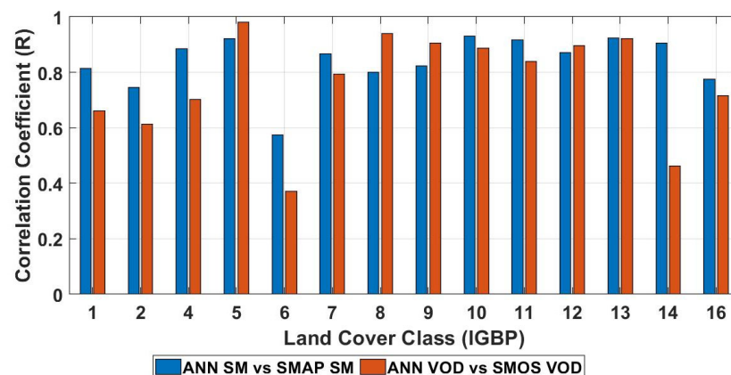
Figure 15. Correlation coefficients between ANN-predicted soil moisture and SMAP soil moisture and between ANN-derived VOD and SMOS VOD across different land cover classifications for the year 2021.
