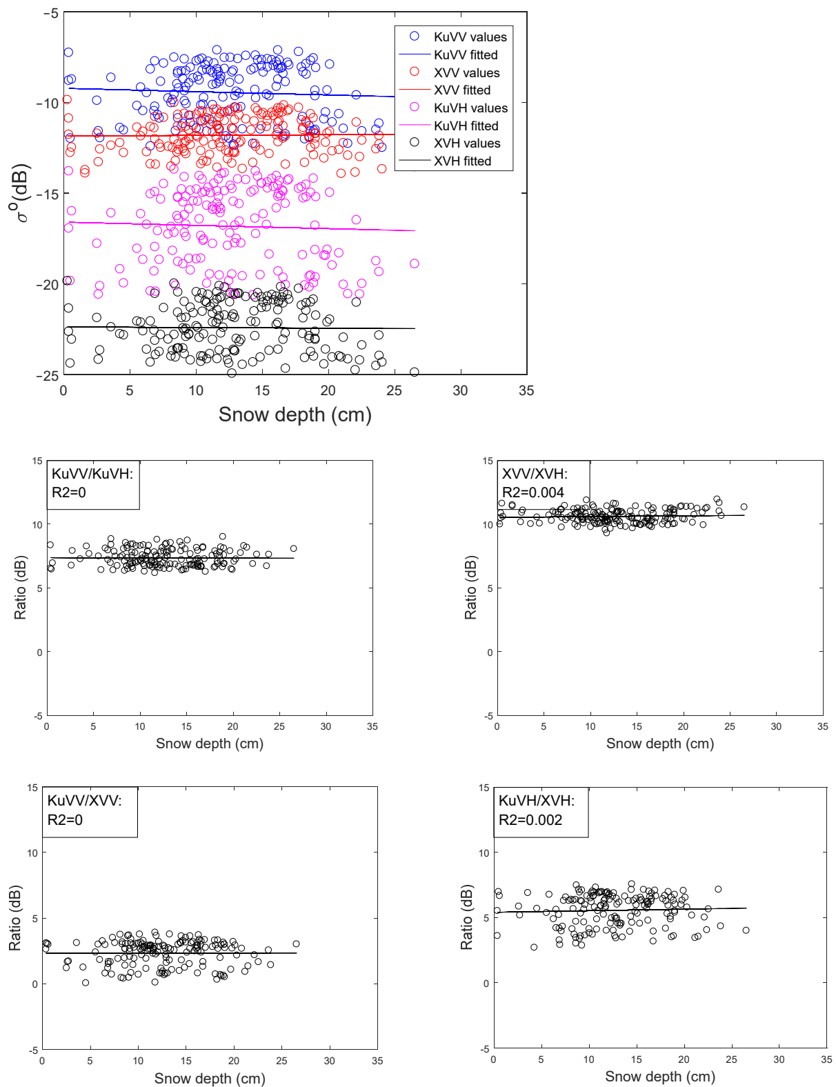
Figure A1. SnowSAR X- and Ku-band backscattering coefficients and their ratios as a function of snow depth on Lake Orajärvi for mission 2. The \sigma^0 was scaled to the reference incidence angle of 43.8 deg for the Ku-band and 43 deg for the X-band.
