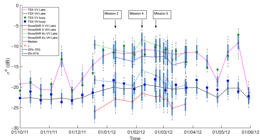
Figure 7. Time series of the average TSX and SnowSAR \sigma^0 data at the VV- and VH-polarizations with boxplots from Lake Orajärvi in 2011–2012. In addition, the mean \sigma^0 of TSX at the IMB location for VV and VH polarizations are shown as a green star and a blue circle, respectively.
