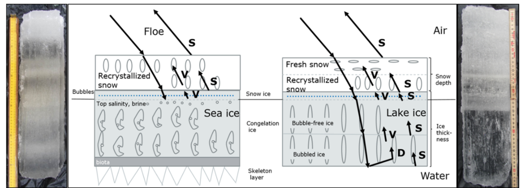
Figure 9. Main sources of radar backscattering (V for volume, S for surface and D for double-bounce scattering) for sea ice and lake ice environments. Radar wave penetration depth is dependent on ice salinity and temperature [12]. In sea ice, the penetration depth is much smaller due to salinity in ice. The ice core sample on the left was collected in Marjaniemi, offshore of Hailuoto, on landfast sea ice in the Baltic Sea. The ice core sample on the right was collected in Lake Orajärvi, Sodankylä, Northern Finland. Some possible forms of snow particles, bubbles and brine inclusions are illustrated in the figure. The arrows show the approximate direction of scattering.
